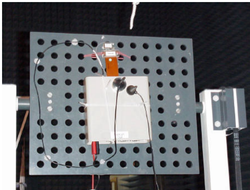
Picture 2 : Setup for radiated tests
