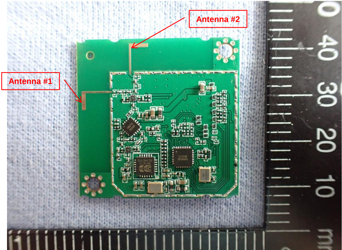
Figure 3 Internal View
