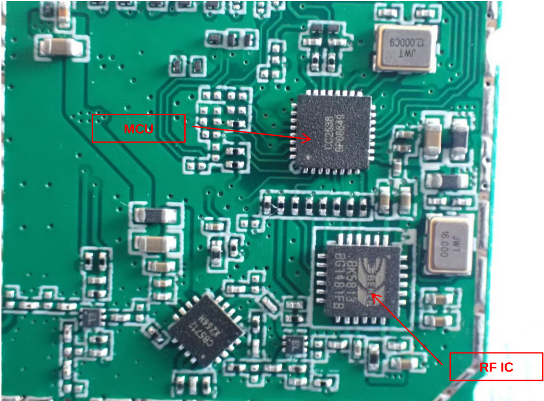
Figure 4 MCU/ RF IC / Oscillator View
