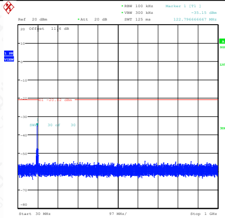
11B-Ant1-2437-30~1000-PASS
