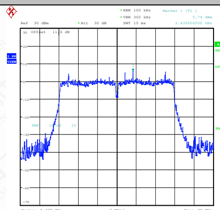
11N20SISO-Ant1-2437-0~Reference-PASS
