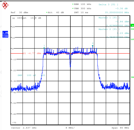
11N40SISO-Ant1-2437-PASS
