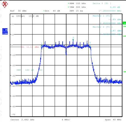
11N20SISO-Ant1-2462-PASS
