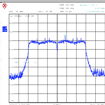
11N20SISO-Ant1-2412-0~Reference-PASS
