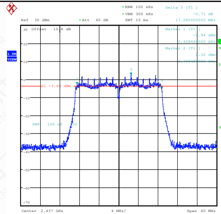
11AC20SISO-Ant1-2437-PASS
