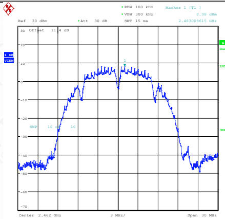
11B-Ant1-2462-0~Reference-PASS
