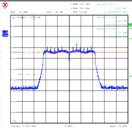
11AC20SISO-Ant1-2412-PASS
