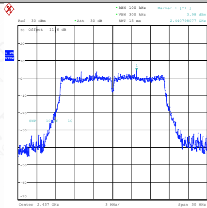
11G-Ant1-2437-0~Reference-PASS
