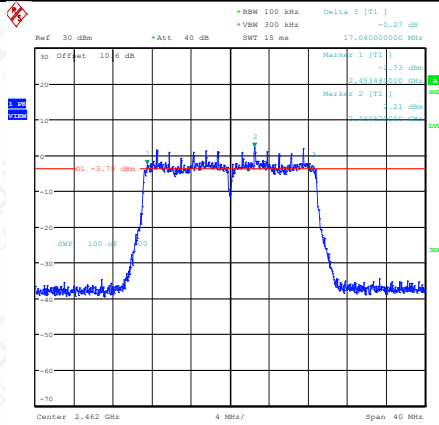
11AC20SISO-Ant1-2462-PASS
