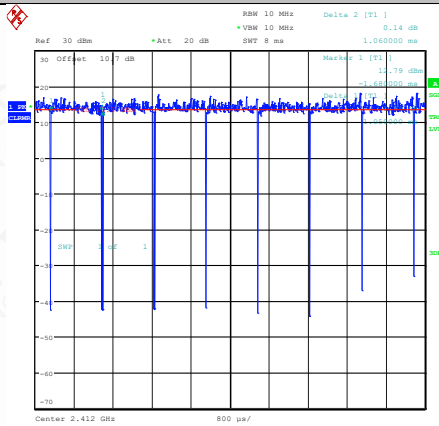
NTNV-11AX20SISO-Ant1-2412
