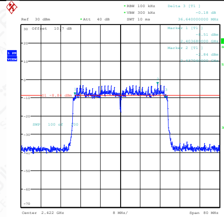
11AX40SISO-Ant1-2422-PASS
