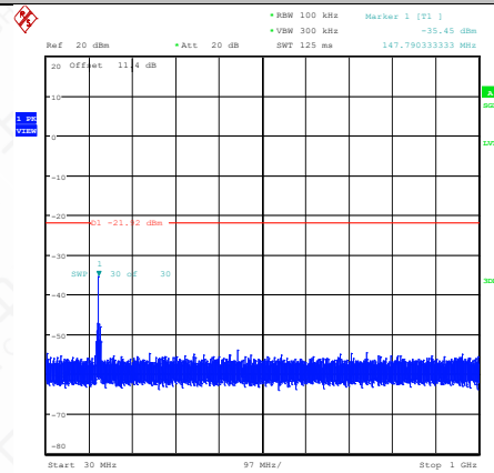
11B-Ant1-2462-30~1000-PASS
