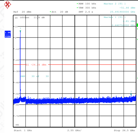
11N20SISO-Ant1-2437-1000~26500-PASS
