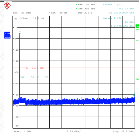
11G-Ant1-2412-1000~26500-PASS
