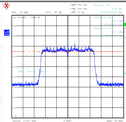
11AX20SISO-Ant1-2437-PASS
