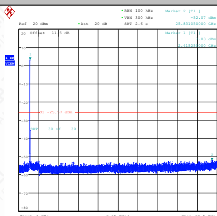
11N20SISO-Ant1-2412-1000~26500-PASS
