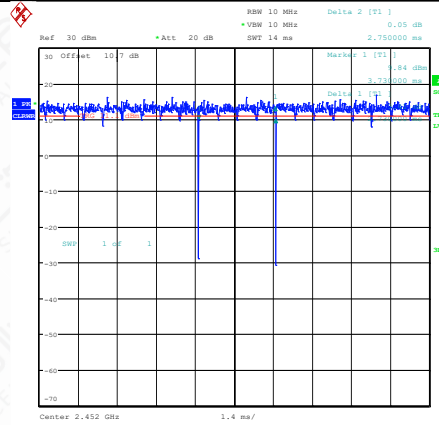
NTNV-11AC40SISO-Ant1-2452
