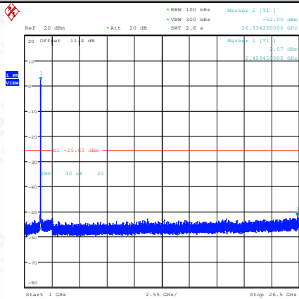
11N20SISO-Ant1-2462-1000~26500-PASS
