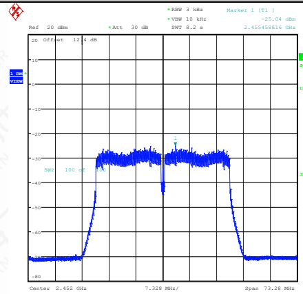
11N40SISO-Ant1-2452-PASS
