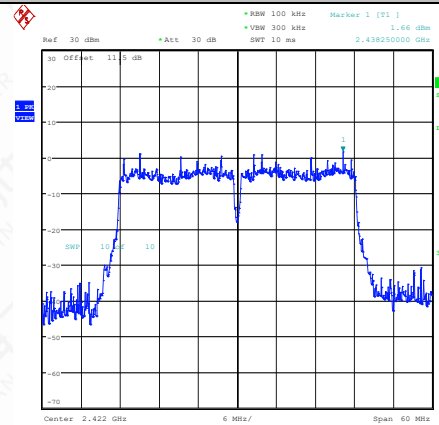
11N40SISO-Ant1-2422-0~Reference-PASS
