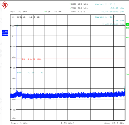
11B-Ant1-2462-1000~26500-PASS
