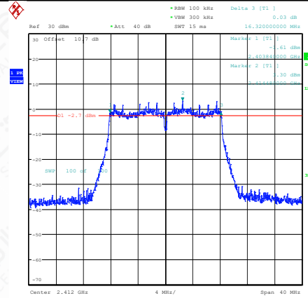
11G-Ant1-2412-PASS
