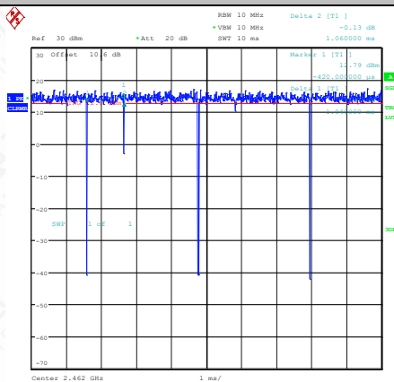
NTNV-11AX20SISO-Ant1-2462
