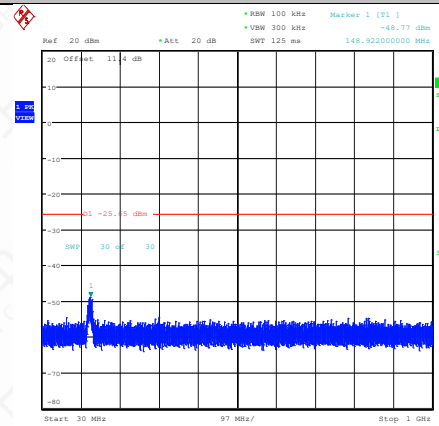
11N20SISO-Ant1-2462-30~1000-PASS
