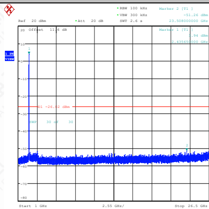
11G-Ant1-2437-1000~26500-PASS
