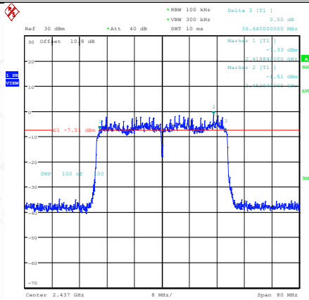
11AX40SISO-Ant1-2437-PASS
