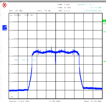
11AX20SISO-Ant1-2412-PASS
