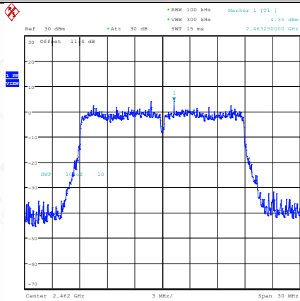
11N20SISO-Ant1-2462-0~Reference-PASS
