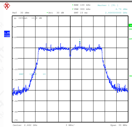
11G-Ant1-2462-0~Reference-PASS
