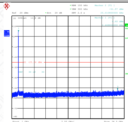
11G-Ant1-2462-1000~26500-PASS
