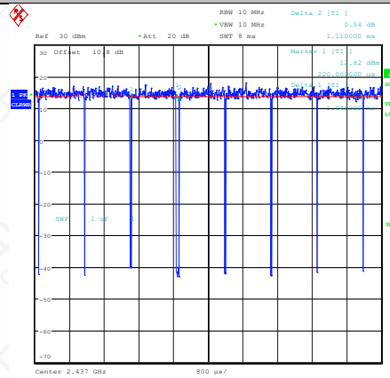
NTNV-11AX20SISO-Ant1-2437
