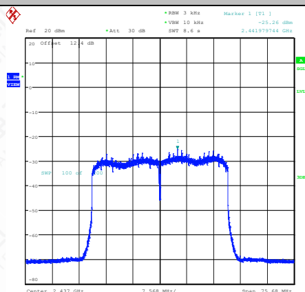
11AX40SISO-Ant1-2437-PASS
