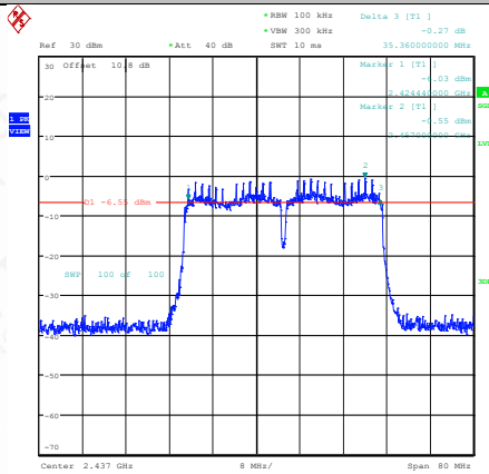
11AC40SISO-Ant1-2437-PASS
