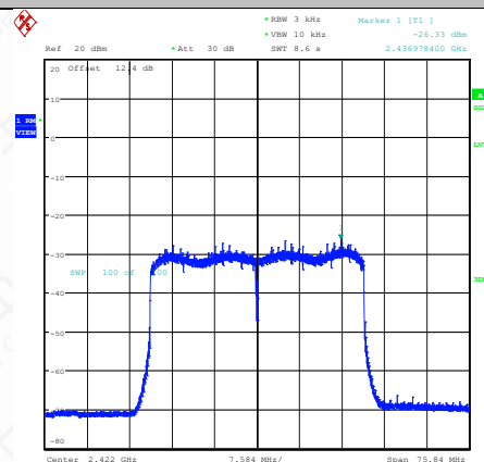
11AX40SISO-Ant1-2422-PASS
