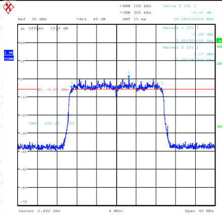
11AX20SISO-Ant1-2462-PASS
