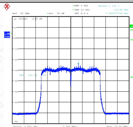
11AX40SISO-Ant1-2452-PASS
