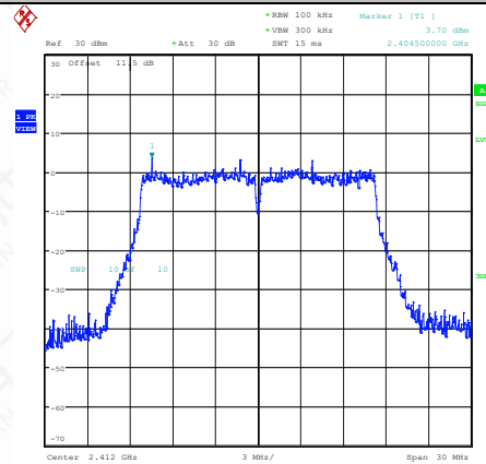
11G-Ant1-2412-0~Reference-PASS
