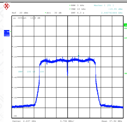
11AX20SISO-Ant1-2437-PASS
