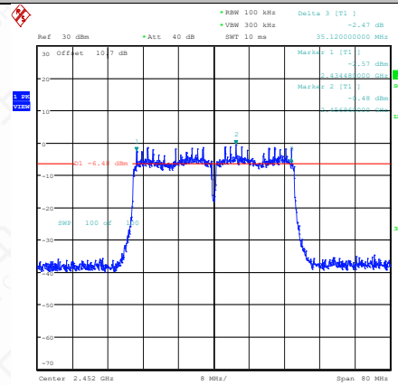
11AC40SISO-Ant1-2452-PASS
