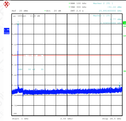
11B-Ant1-2437-1000~26500-PASS
