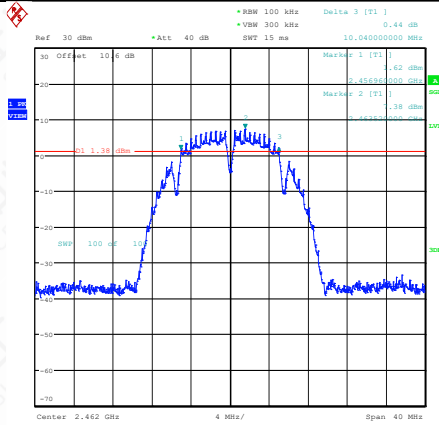
11B-Ant1-2462-PASS
