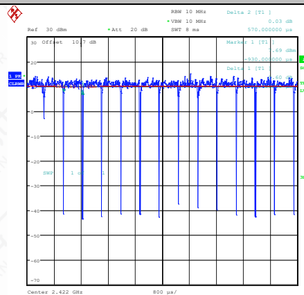
NTNV-11AX40SISO-Ant1-2422
