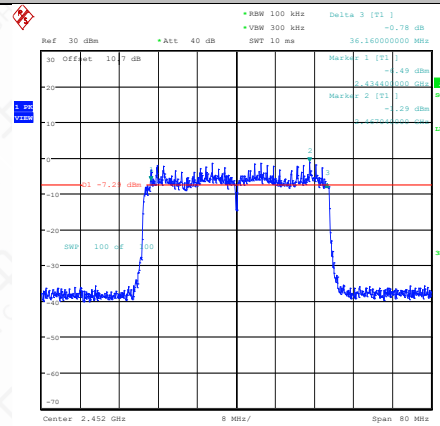
11AX40SISO-Ant1-2452-PASS
