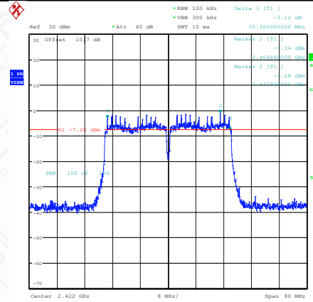
11AC40SISO-Ant1-2422-PASS
