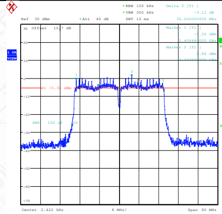
11N40SISO-Ant1-2422-PASS
