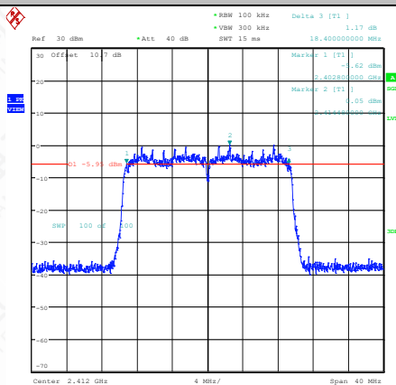
11AX20SISO-Ant1-2412-PASS
