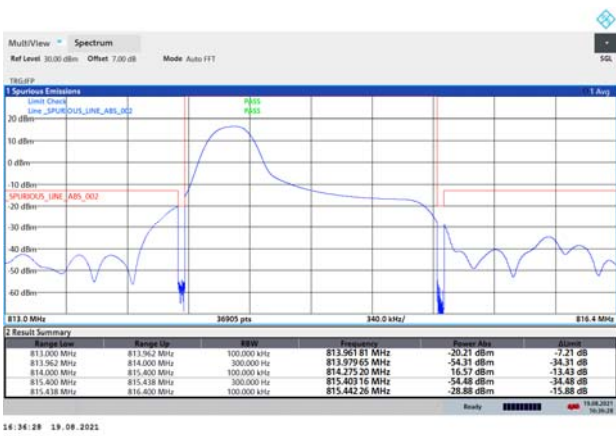
LTE eMTC Band 26 QPSK 1.4MHz CH-Low 100%RB
