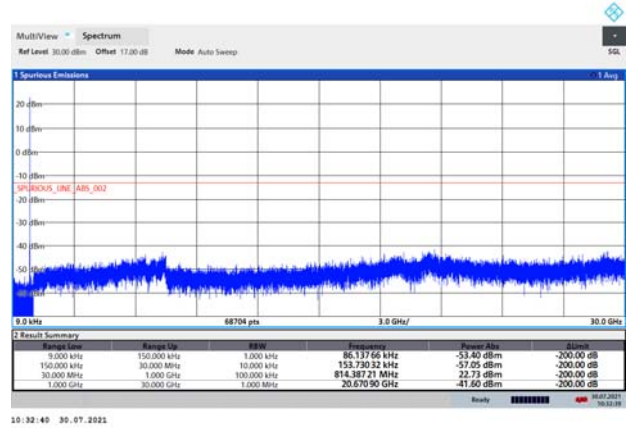
LTE eMTC Band 26 3MHz CH Middle 9kHz~30GHz
