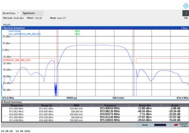
LTE eMTC Band 26 QPSK 3MHz CH-Low 1RB
