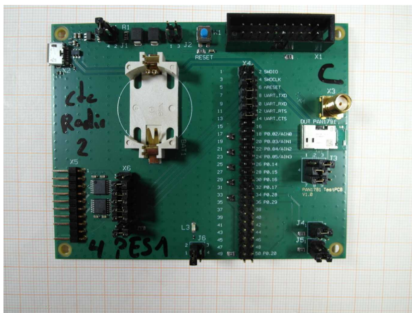
Photo 4 conducted Sample
