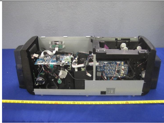
EUT Without Enclosure
