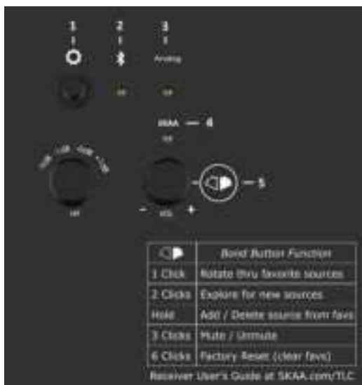
Figure 2: SKAA Bond Button & Bonding Table
