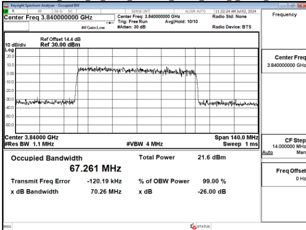
Band77-Part27_70MHz_CP_OFDM_SCS30kHz_16QAM_RB189_0_Chain1_CH656000
