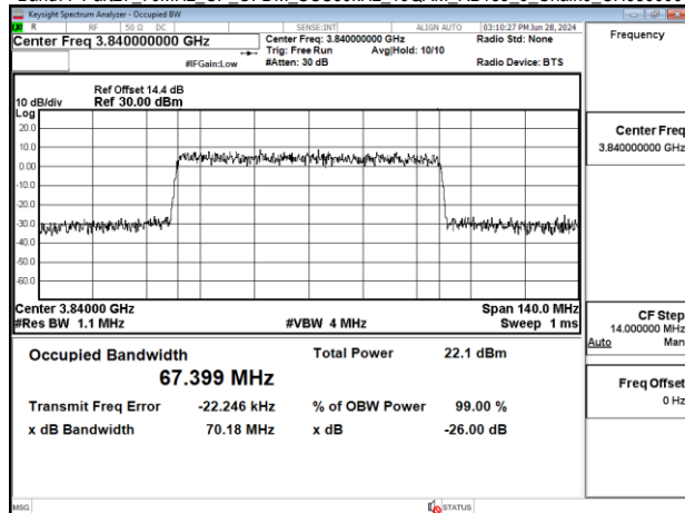
Band77-Part27_70MHz_CP_OFDM_SCS30kHz_16QAM_RB189_0_Chain0_CH656000
