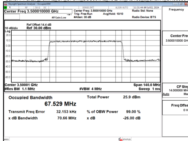
Band77-Part27_70MHz_CP_OFDM_SCS30kHz_16QAM_RB189_0_Chain1_CH633334
