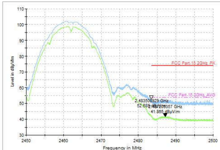
Fig.66 Radiated Restricted Band (802.11b, CH11, 2.45GHz~2.50GHz)
