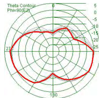
Efficiency68.6%
