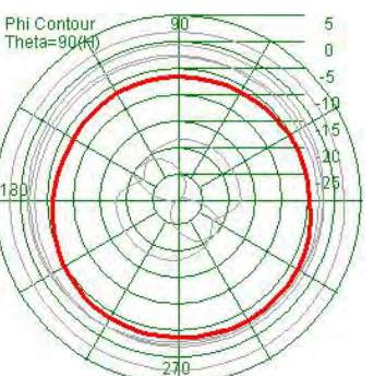
Gain(Peak):2.26dBi
