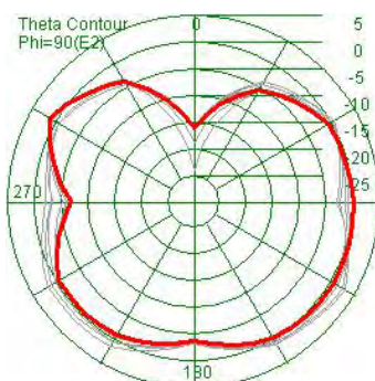
Efficiency:75.9%
