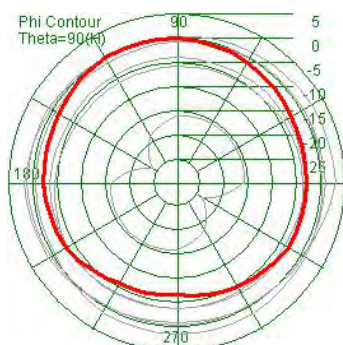
Gain(Peak):2.03dBi
