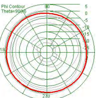
Gain(Peak):1.55dBi
