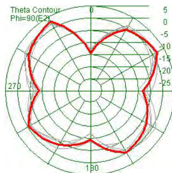
Efficiency:71.5%
