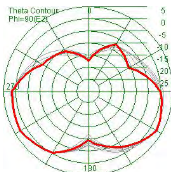
Efficiency:76.7%
