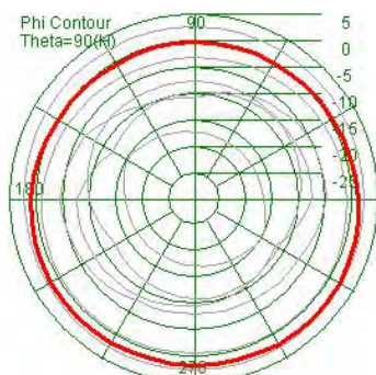
Gain(Peak):2.63dBi
