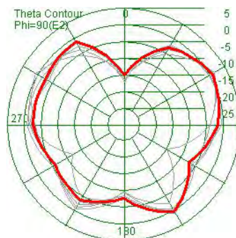
Efficiency:73.4%
