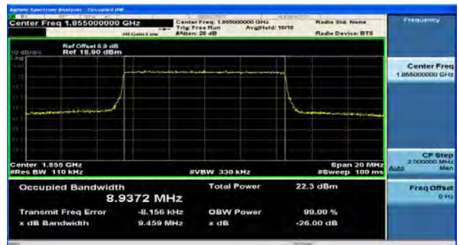
LTE band 2 - Low CH 16QAM-10
