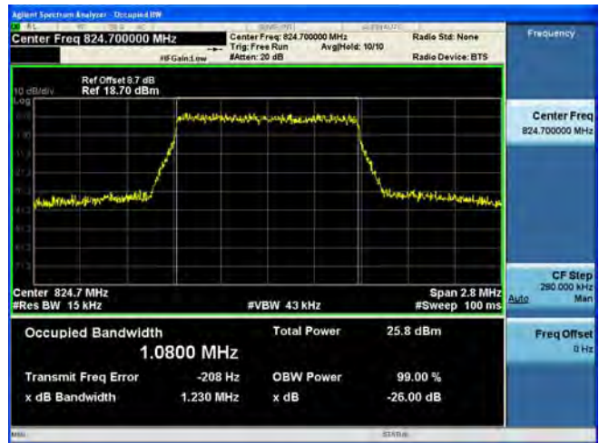
LTE band 5 - Low CH 16QAM-1.4
