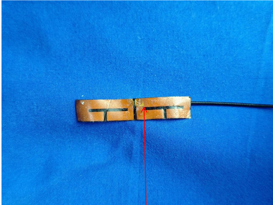
5GWIFI Antenna
