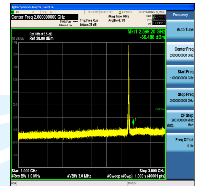
Band7_10MHz_QPSK_20800_1RB#0_1000~3000_1000~3000
