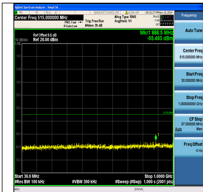
Band7_10MHz_QPSK_20800_1RB#0_30~1000_30~1000
