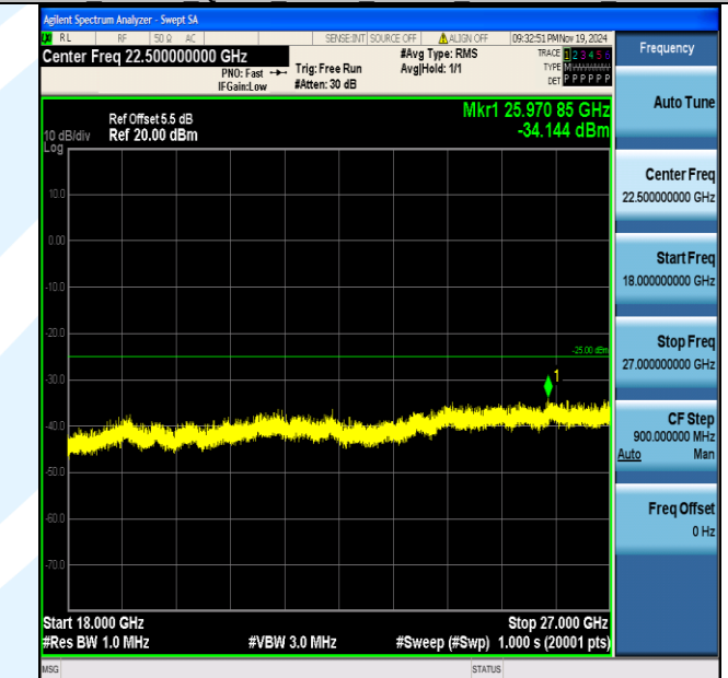
Band7_10MHz_QPSK_20800_1RB#0_18000~27000_18000~27000
