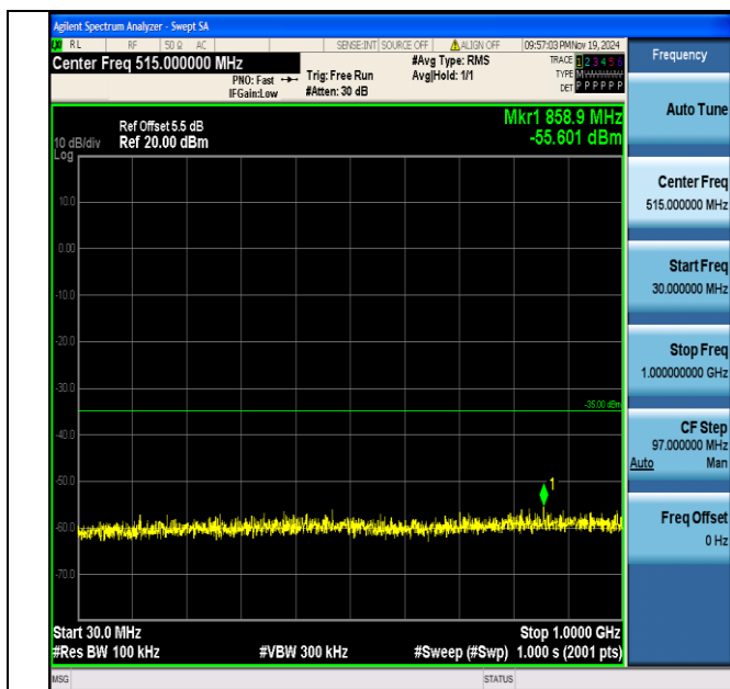
Band7_20MHz_QPSK_21350_1RB#0_30~1000_30~1000
