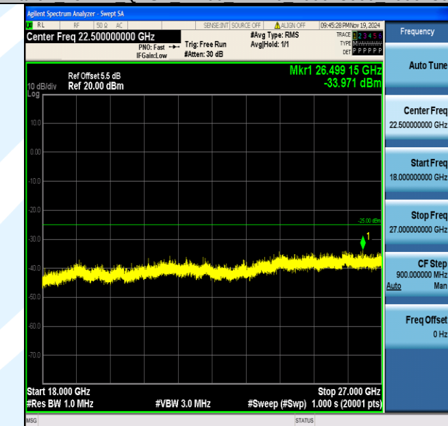
Band7_15MHz_QPSK_21100_1RB#0_18000~27000_18000~27000
