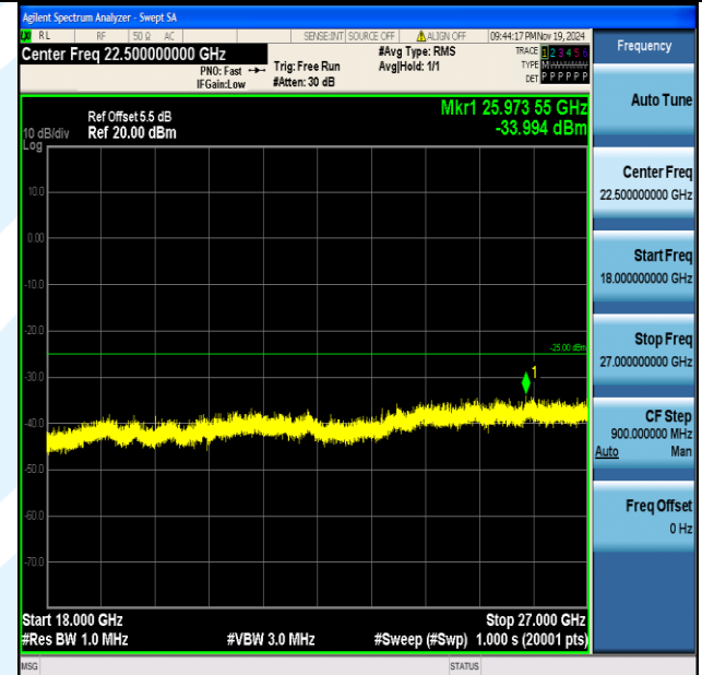
Band7_15MHz_QPSK_20825_1RB#0_18000~27000_18000~27000
