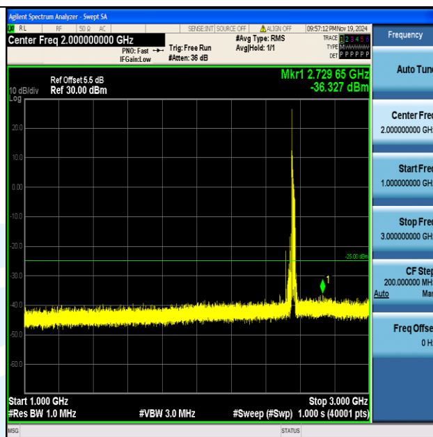
Band7_20MHz_QPSK_21350_1RB#0_1000~3000_1000~3000
