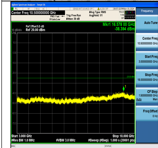
Band7_20MHz_QPSK_21350_1RB#0_3000~18000_3000~18000
