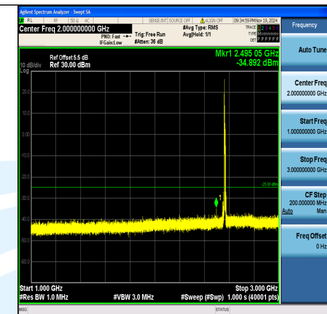
Band7_10MHz_QPSK_21400_1RB#0_1000~3000_1000~3000
