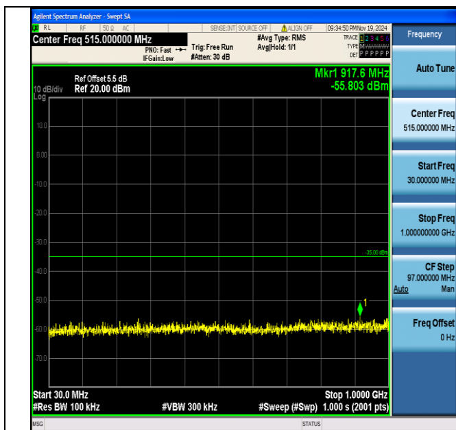
Band7_10MHz_QPSK_21400_1RB#0_30~1000_30~1000
