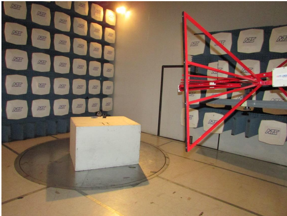
Radiated Spurious Emissions 30-1000MHz Horizontal
