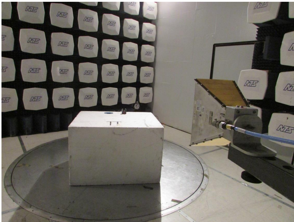
Radiated Spurious Emissions 1-10GHz Horizontal
