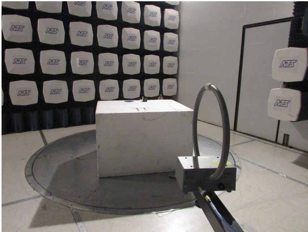
Radiated Spurious Emissions 9kHz-30MHz Perpendicular
