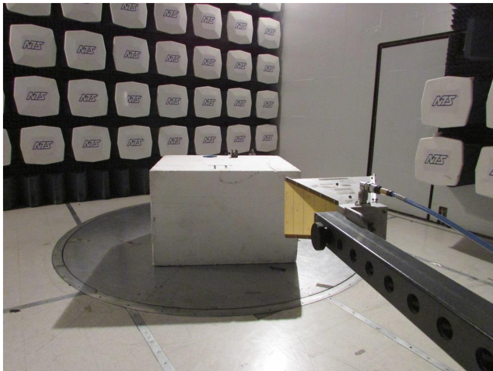
Radiated Spurious Emissions 1-10GHz Vertical
