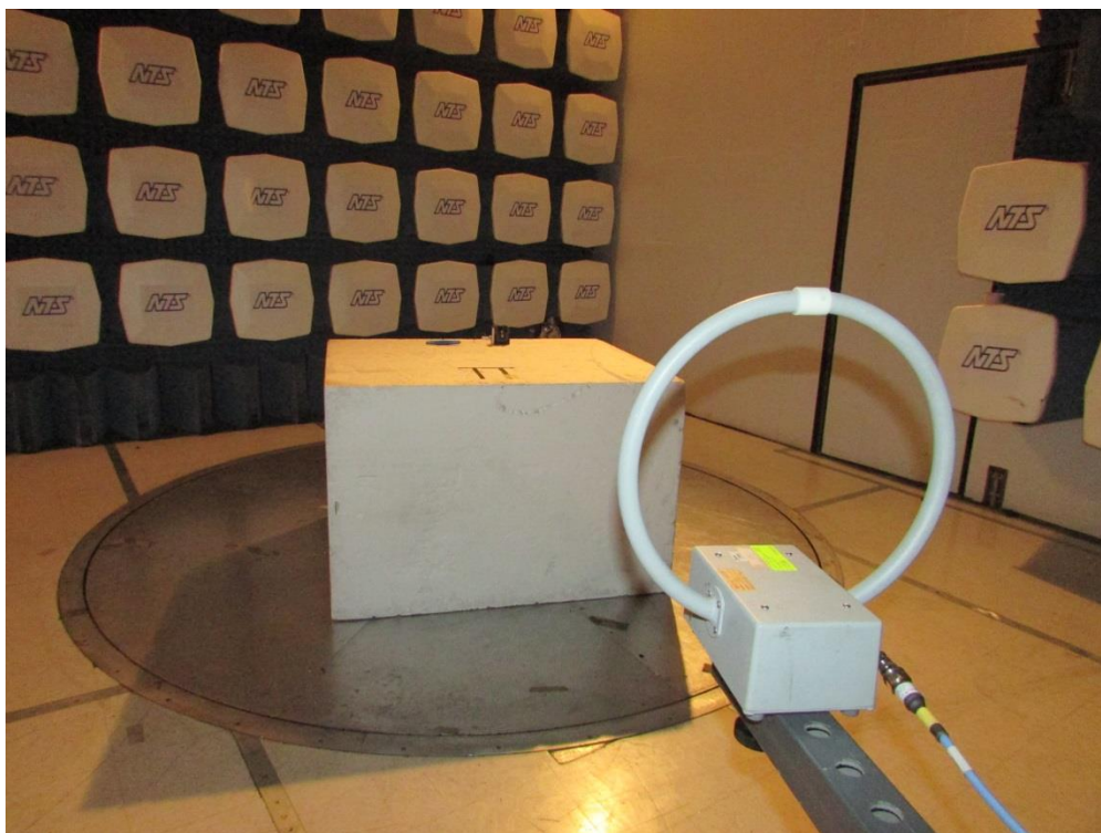
Radiated Spurious Emissions 9kHz-30MHz Parallel
