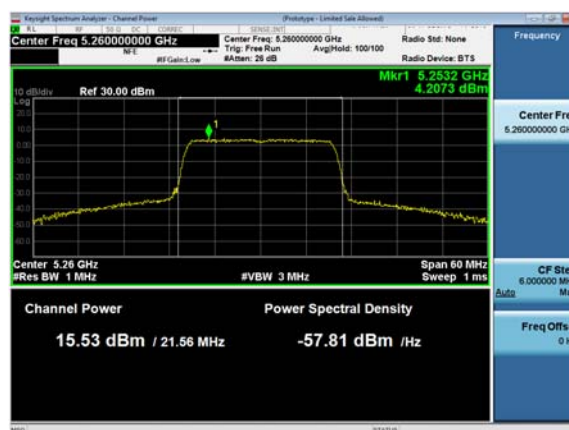
Antenna D
