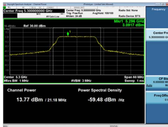
Antenna B
