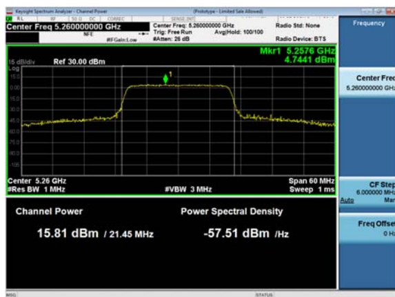
Antenna C
