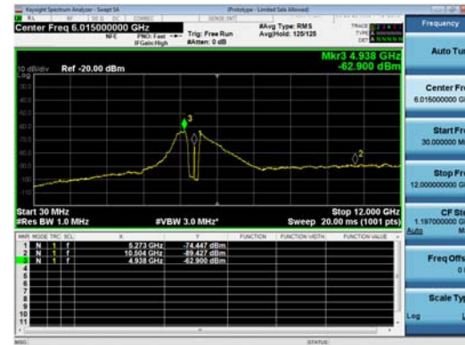
Antenna D
