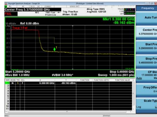
Antenna B
