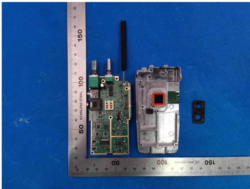
INTENAL VIEW OF EUT (FIGURE 1)
