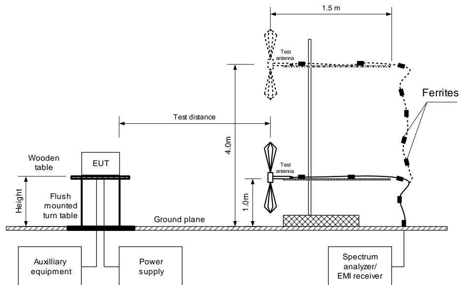
Figure 7.4.2 Setup for radiated spurious emission measurements above 30 MHz
