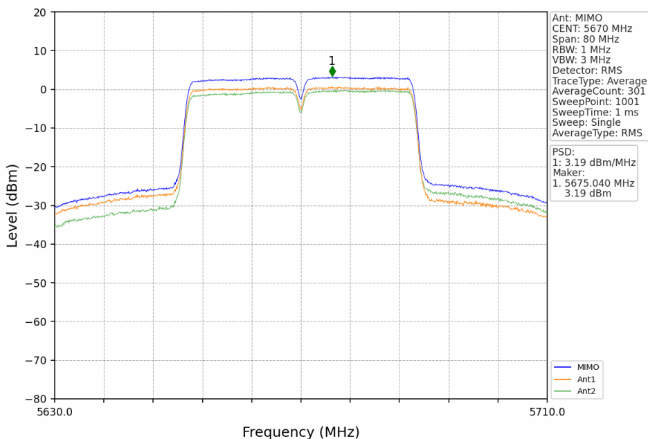
802.11n(HT40)_HCH_5670MHz_MIMO_NTNV
