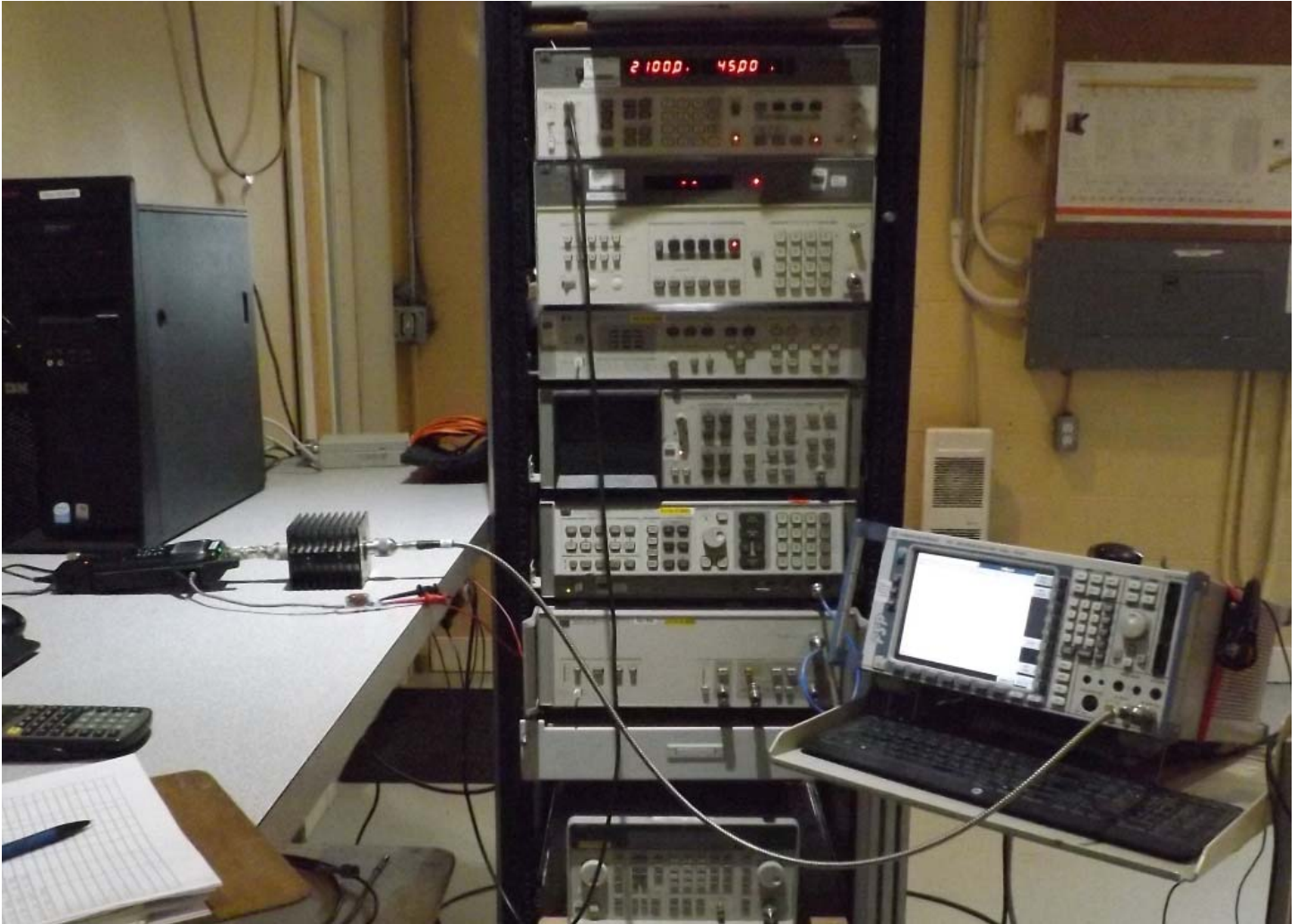
Figure E24.1 – Setup Photo – Conducted Measurements
