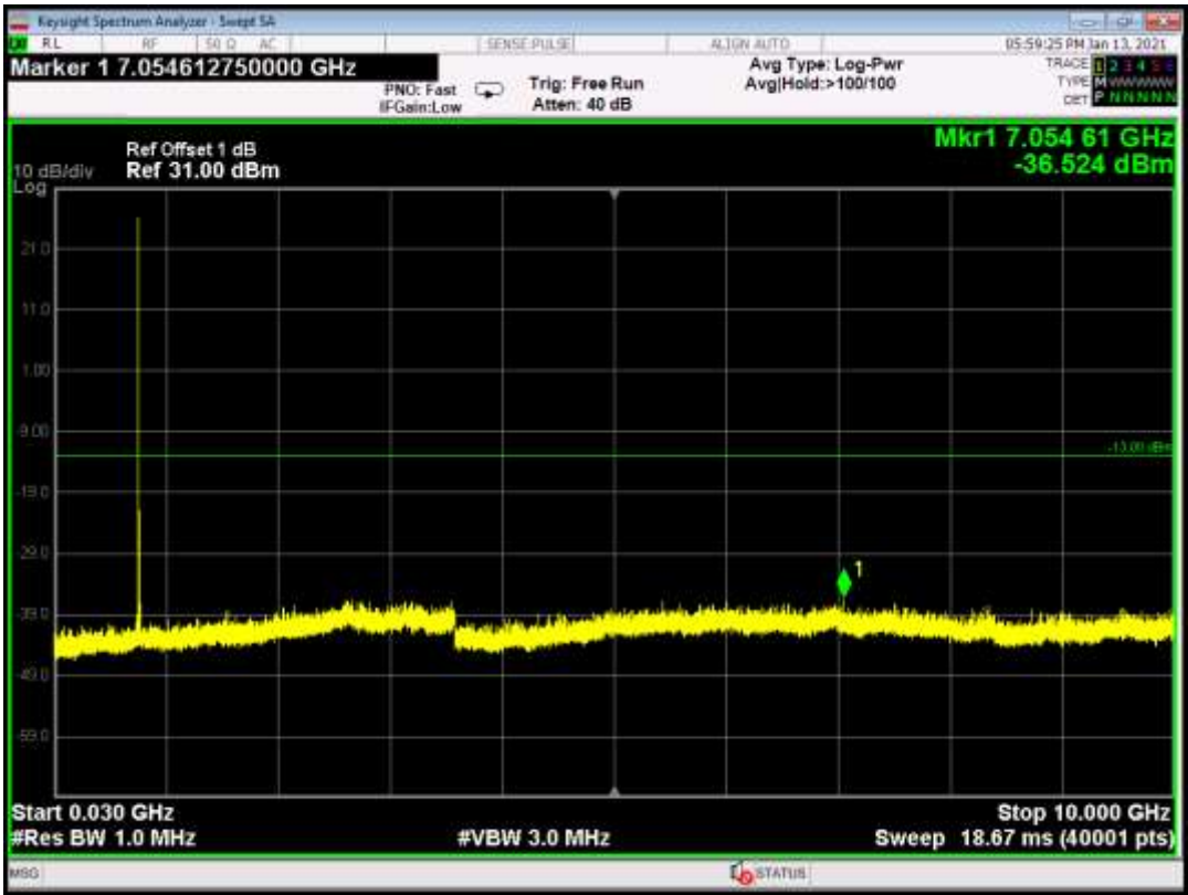
Band13 QPSK BW=1.4MHz Channel=23205 RB Size=1 Position=#0
