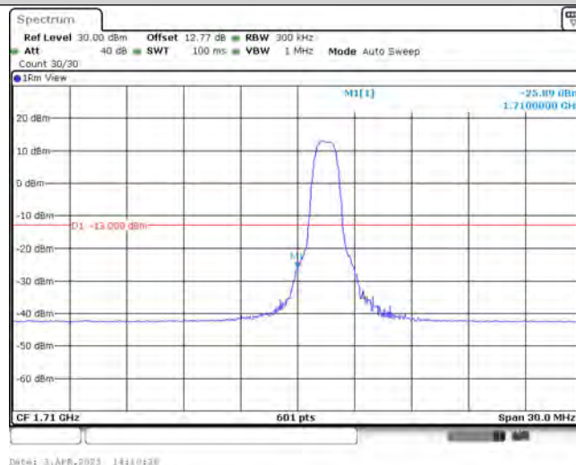
Band4-15MHz-QPSK-20025-6-0-Low--25.89-PASS
