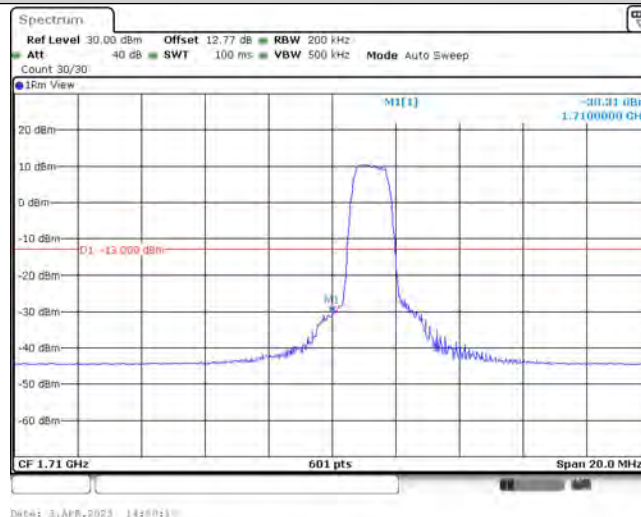
Band66-10MHz-QPSK-132022-6-0-Low--30.31-PASS
