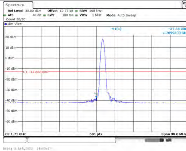
Band66-15MHz-16QAM-132047-1-0-Low--37.56-PASS
