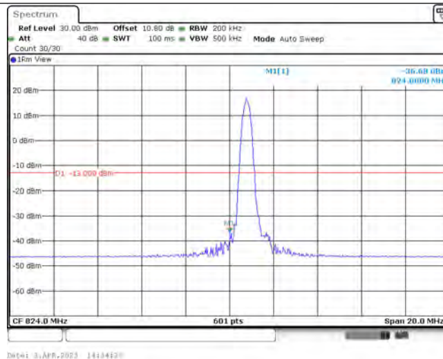
Band5-10MHz-16QAM-20450-1-0-Low--36.68-PASS
