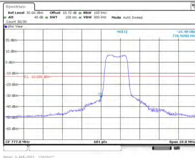
Band13-5MHz-16QAM-23205-6-0-Low--31.98-PASS
