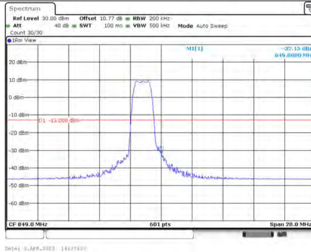
Band5-10MHz-16QAM-20600-6-0-High--32.15-PASS
