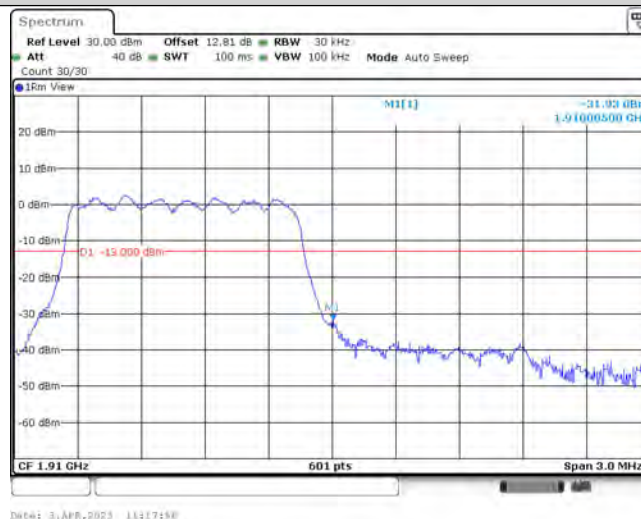
Band2-1.4MHz-QPSK-19193-6-0-High--31.93-PASS
