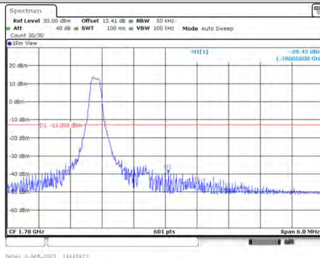
Band66-3MHz-QPSK-132657-1-0-High--39.42-PASS
