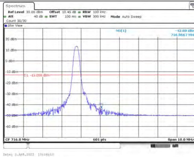
Band12-5MHz-QPSK-23155-1-0-High--43.08-PASS
