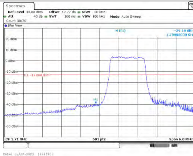
Band66-3MHz-QPSK-131987-6-0-Low--39.16-PASS
