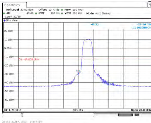
Band66-10MHz-16QAM-132022-6-0-Low--29.96-PASS
