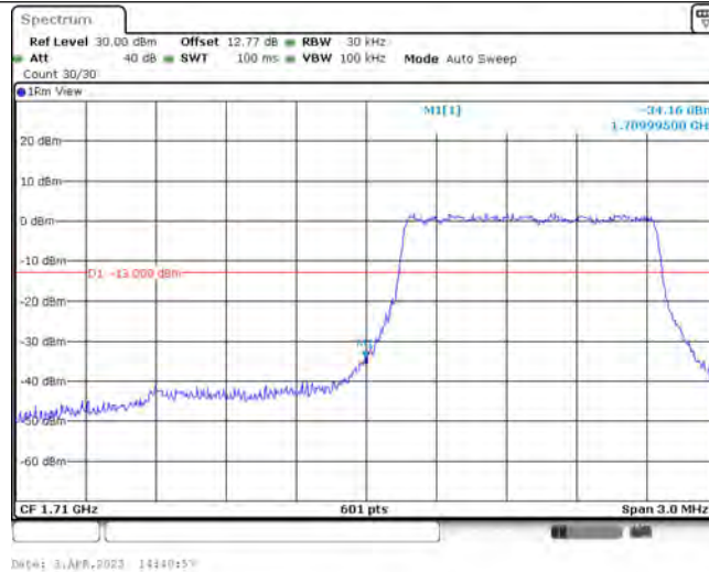
Band66-1.4MHz-16QAM-131979-6-0-Low--34.16-PASS
