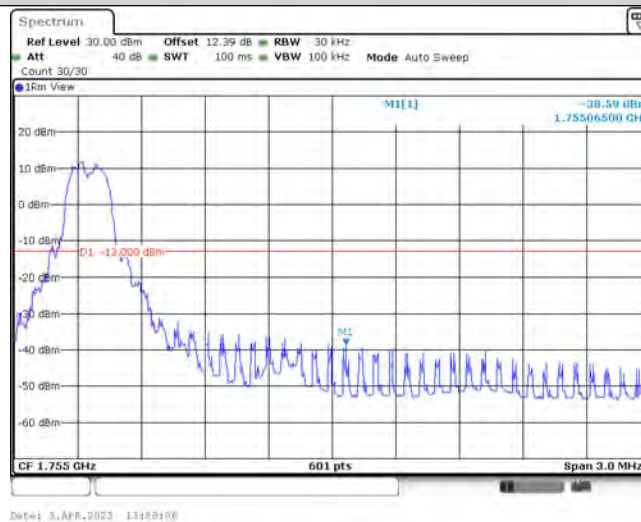
Band4-1.4MHz-QPSK-20393-1-0-High--38.59-PASS
