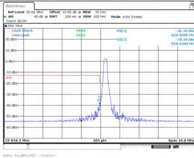
Band26-1.4MHz-16QAM-26740-1-0-Low--36.16,-39.10-PASS
