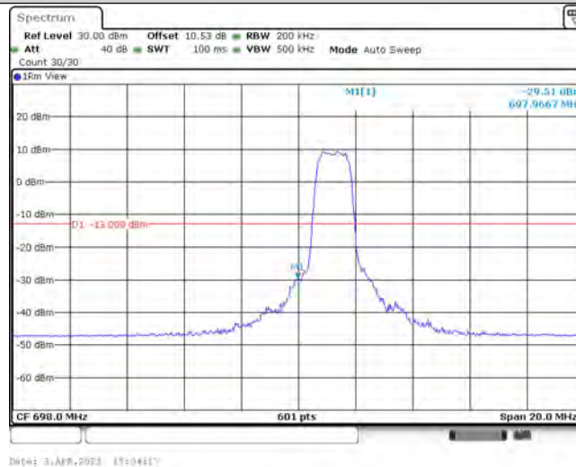
Band85-10MHz-16QAM-134052-6-0-Low--29.51-PASS
