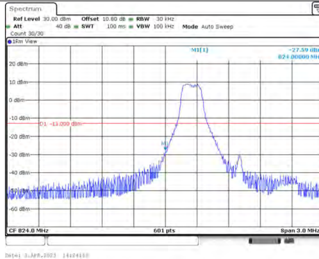
Band5-1.4MHz-16QAM-20407-1-0-Low--27.59-PASS
