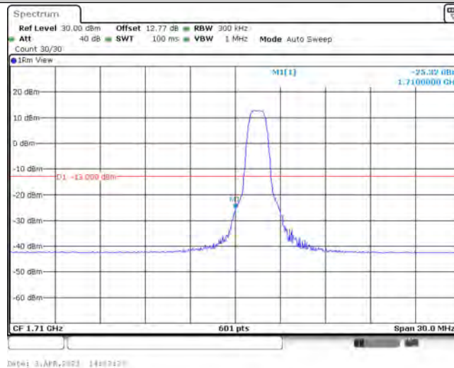
Band66-15MHz-16QAM-132047-6-0-Low--25.32-PASS
