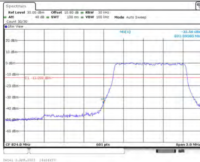
Band5-1.4MHz-16QAM-20407-6-0-Low--35.56-PASS
