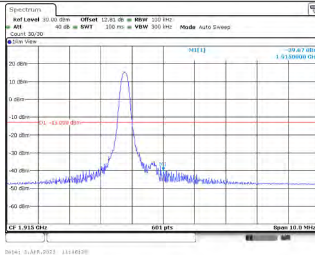
Band25-5MHz-QPSK-26665-1-0-High--39.67-PASS
