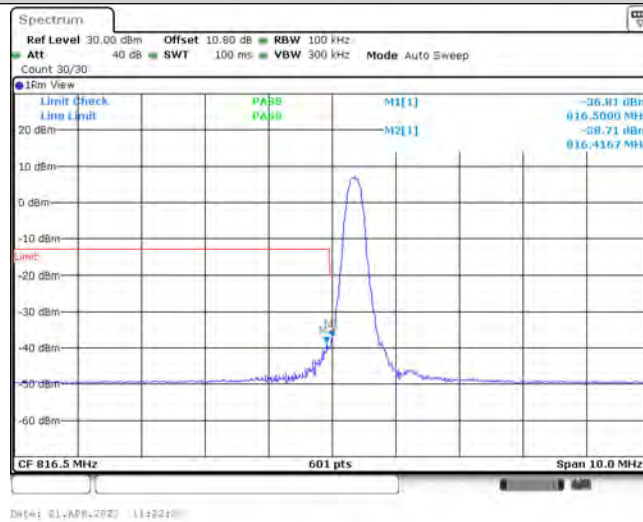
Band26-5MHz-QPSK-26740-1-0-Low--36.81,-38.71-PASS
