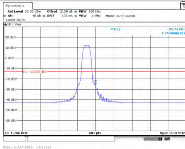
Band4-15MHz-16QAM-20325-6-0-High--25.74-PASS
