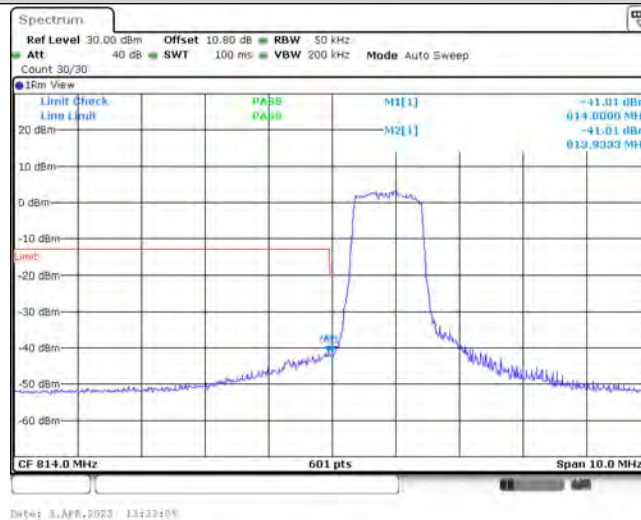
Band26-3MHz-QPSK-26705-6-0-Low--41.01,-41.01-PASS
