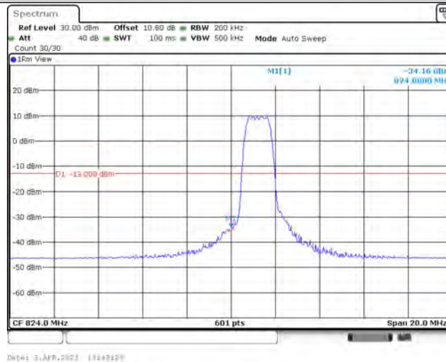
Band26-10MHz-16QAM-26840-6-0-Low--34.16-PASS
