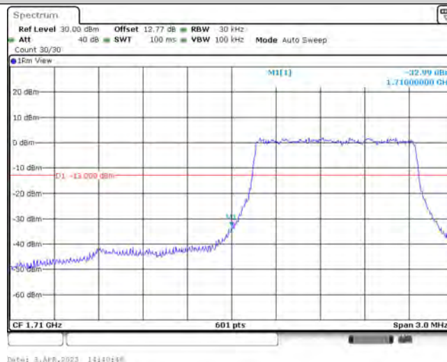
Band66-1.4MHz-QPSK-131979-6-0-Low--32.99-PASS
