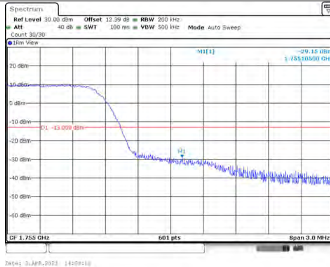
Band4-10MHz-16QAM-20350-6-0-High--29.15-PASS
