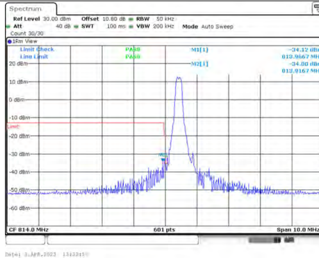
Band26-3MHz-QPSK-26705-1-0-Low--34.12,-34.00-PASS
