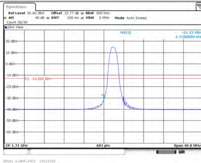
Band4-20MHz-QPSK-20050-6-0-Low--31.12-PASS
