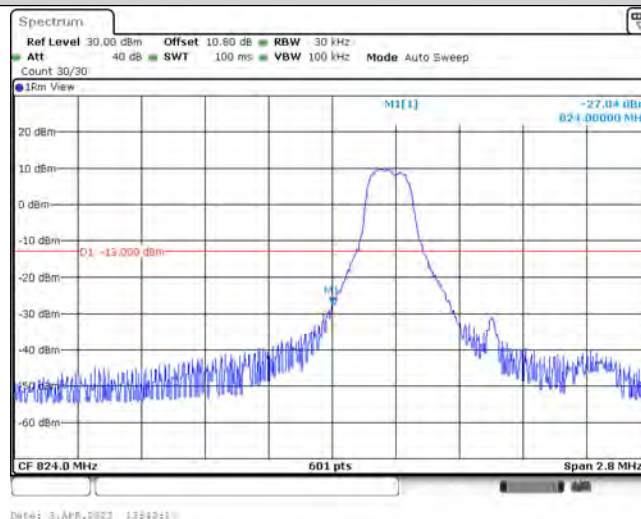
Band26-1.4MHz-16QAM-26797-1-0-Low--27.04-PASS
