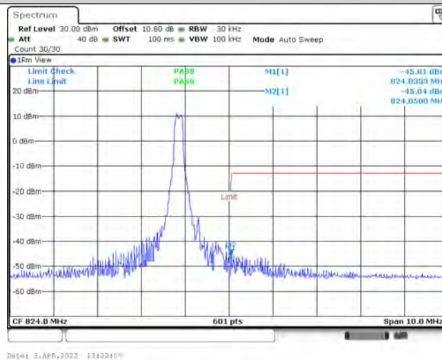
Band26-1.4MHz-QPSK-26783-1-0-High--45.81,-45.04-PASS
