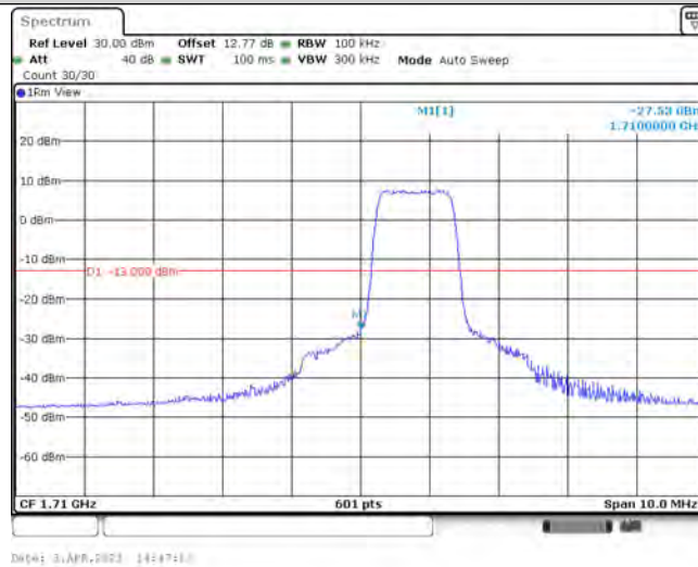
Band66-5MHz-16QAM-131997-6-0-Low--27.53-PASS
