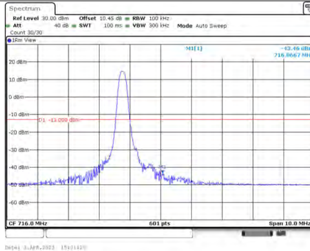
Band85-5MHz-QPSK-134157-1-0-High--43.46-PASS
