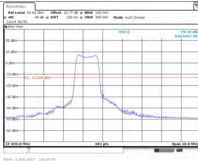
Band5-5MHz-QPSK-20625-6-0-High--29.38-PASS
