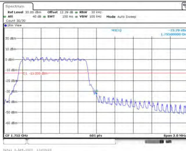
Band4-1.4MHz-QPSK-20393-6-0-High--33.28-PASS
