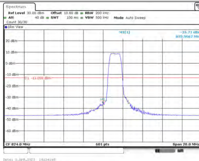
Band5-10MHz-16QAM-20450-6-0-Low--35.71-PASS
