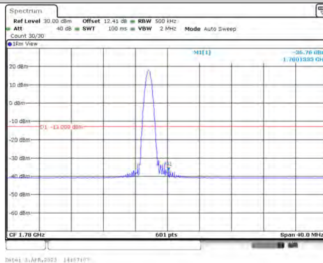
Band66-20MHz-QPSK-132572-1-0-High--36.76-PASS
