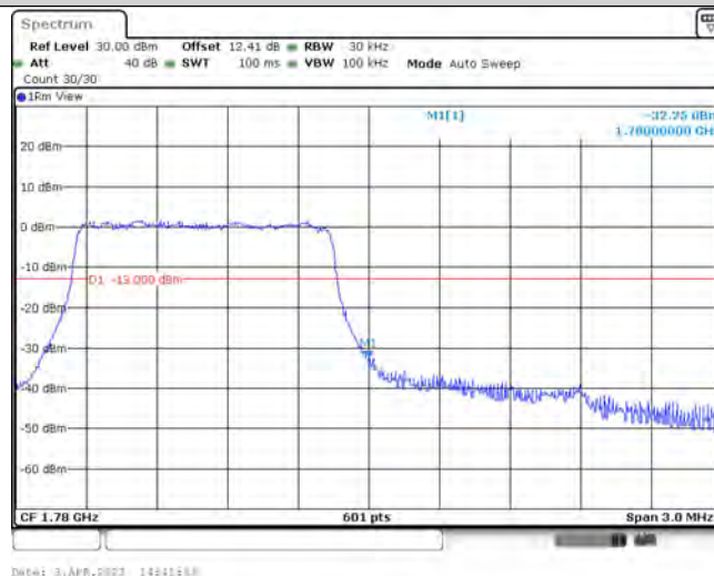
Band66-1.4MHz-16QAM-132665-6-0-High--32.25-PASS
