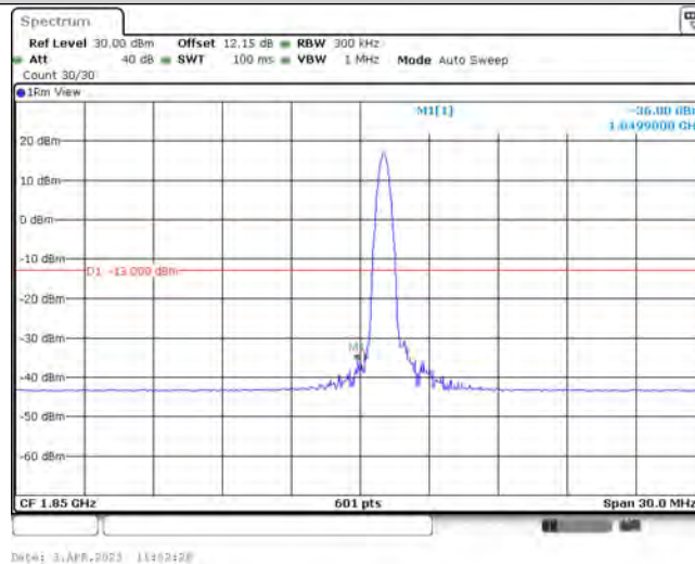
Band25-15MHz-QPSK-26115-1-0-Low--36.00-PASS
