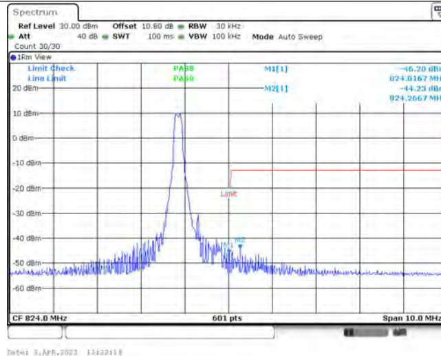
Band26-1.4MHz-16QAM-26783-1-0-High--46.20,-44.23-PASS
