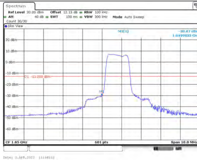
Band25-5MHz-QPSK-26065-6-0-Low--30.07-PASS
