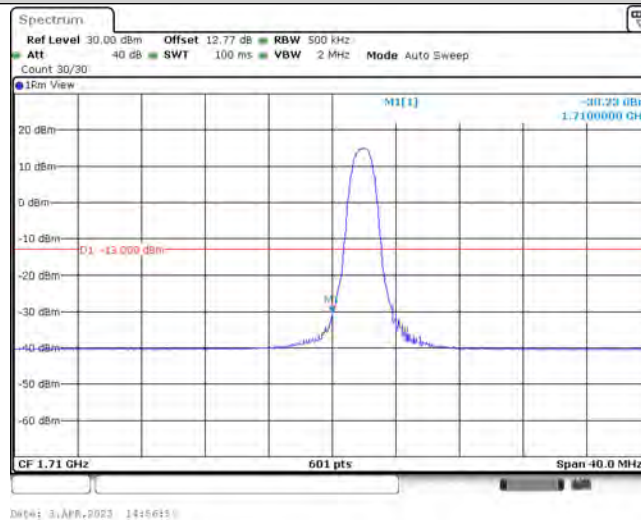
Band66-20MHz-16QAM-132072-6-0-Low--30.23-PASS
