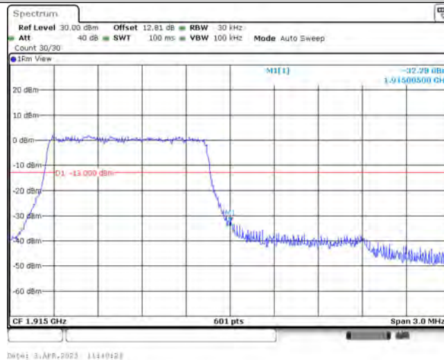
Band25-1.4MHz-QPSK-26683-6-0-High--32.28-PASS
