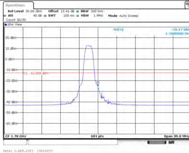
Band66-15MHz-QPSK-132597-6-0-High--25.27-PASS
