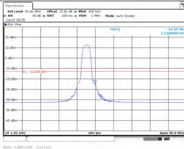
Band2-15MHz-QPSK-19125-6-0-High--25.55-PASS
