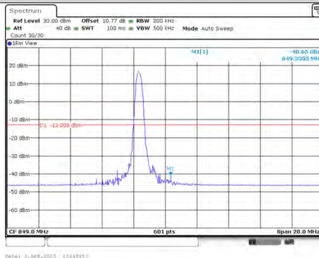
Band26-10MHz-16QAM-26990-1-0-High--40.65-PASS
