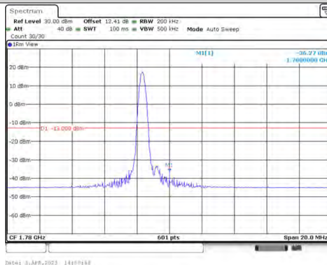
Band66-10MHz-16QAM-132622-1-0-High--36.27-PASS
