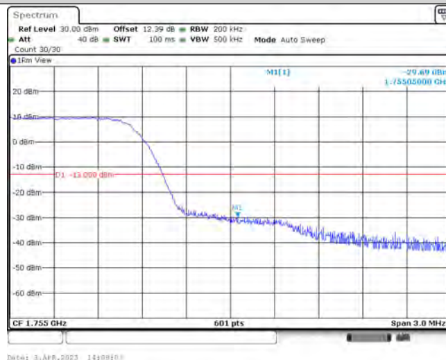
Band4-10MHz-QPSK-20350-6-0-High--29.69-PASS
