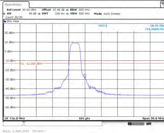
Band85-10MHz-QPSK-134132-6-0-High--28.93-PASS
