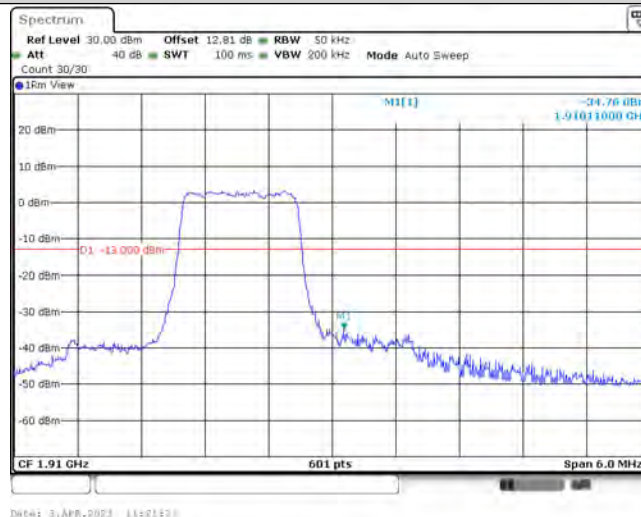
Band2-3MHz-16QAM-19185-6-0-High--34.76-PASS
