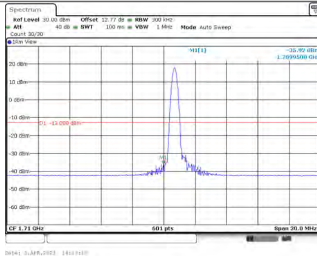
Band4-15MHz-QPSK-20025-1-0-Low--35.92-PASS
