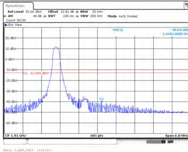
Band2-3MHz-16QAM-19185-1-0-High--40.64-PASS
