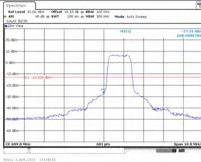
Band12-5MHz-QPSK-23035-6-0-Low--27.25-PASS
