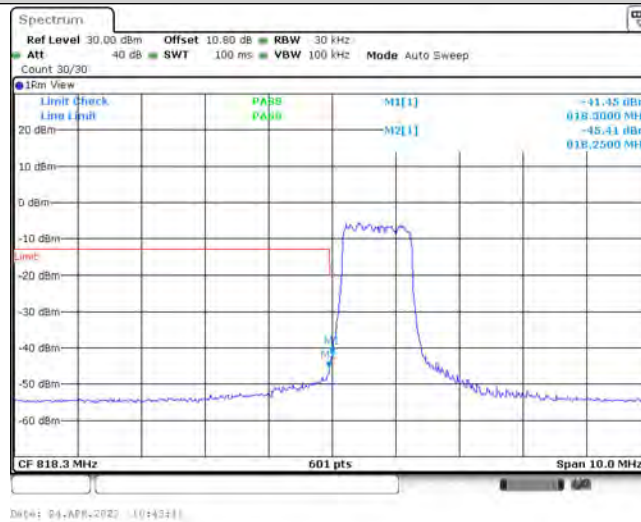
Band26-1.4MHz-QPSK-26740-6-0-Low--41.45,-45.41-PASS
