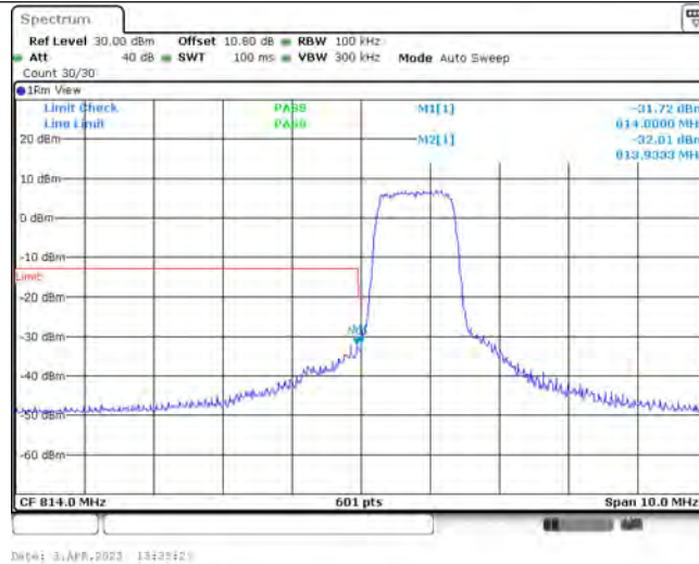
Band26-5MHz-QPSK-26715-6-0-Low--31.72,-32.01-PASS
