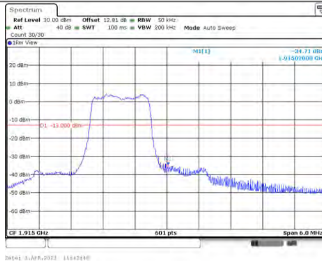
Band25-3MHz-16QAM-26675-6-0-High--34.71-PASS
