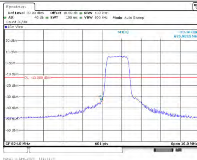
Band5-5MHz-16QAM-20425-6-0-Low--33.16-PASS
