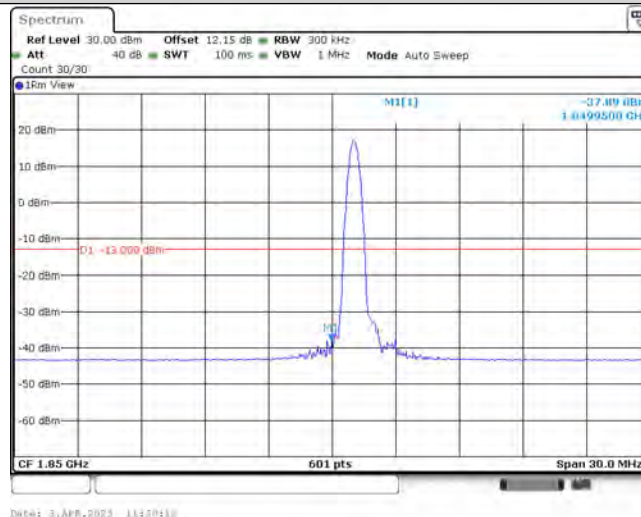
Band2-15MHz-16QAM-18675-1-0-Low--37.89-PASS
