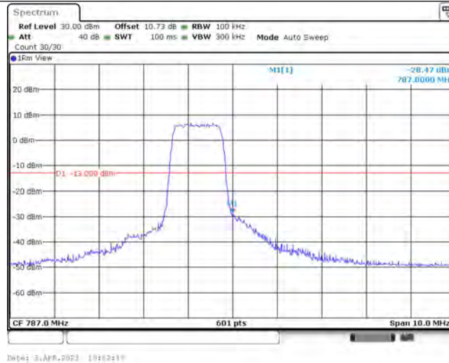
Band13-5MHz-QPSK-23255-6-0-High--28.47-PASS
