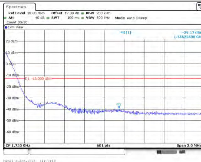
Band4-10MHz-16QAM-20350-1-0-High--39.17-PASS
