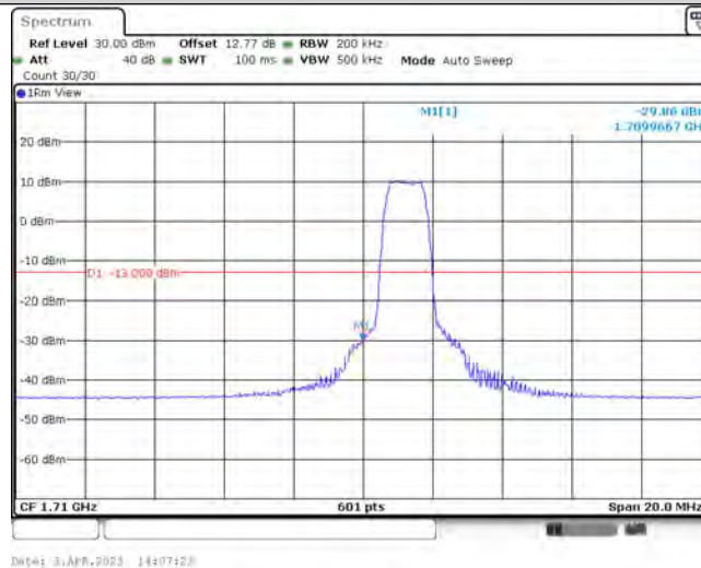
Band4-10MHz-16QAM-20000-6-0-Low--29.86-PASS
