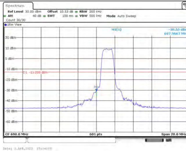
Band85-10MHz-QPSK-134052-6-0-Low--30.55-PASS
