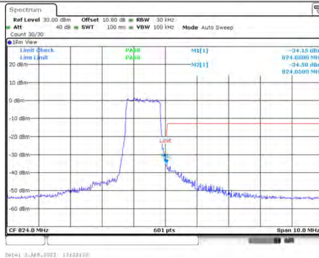
Band26-1.4MHz-16QAM-26783-6-0-High--34.15,-34.58-PASS
