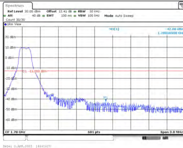
Band66-1.4MHz-16QAM-132665-1-0-High--42.06-PASS
