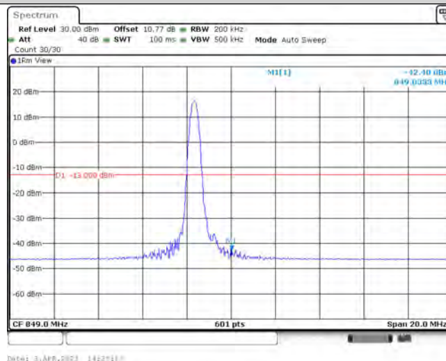
Band5-10MHz-16QAM-20600-1-0-High--42.40-PASS
