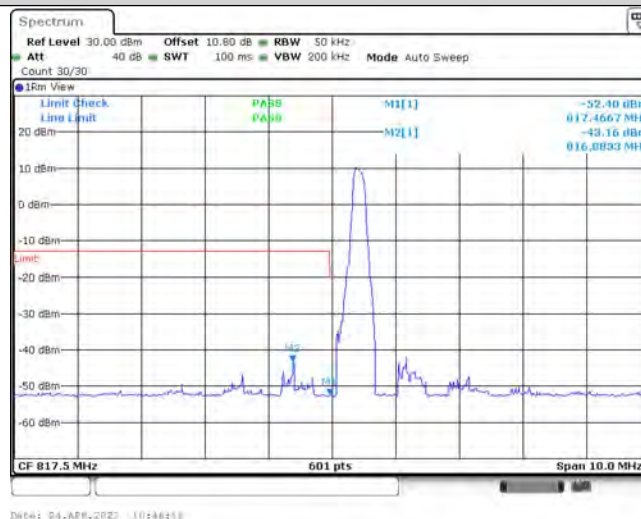
Band26-3MHz-QPSK-26740-1-0-Low--52.40,-43.16-PASS
