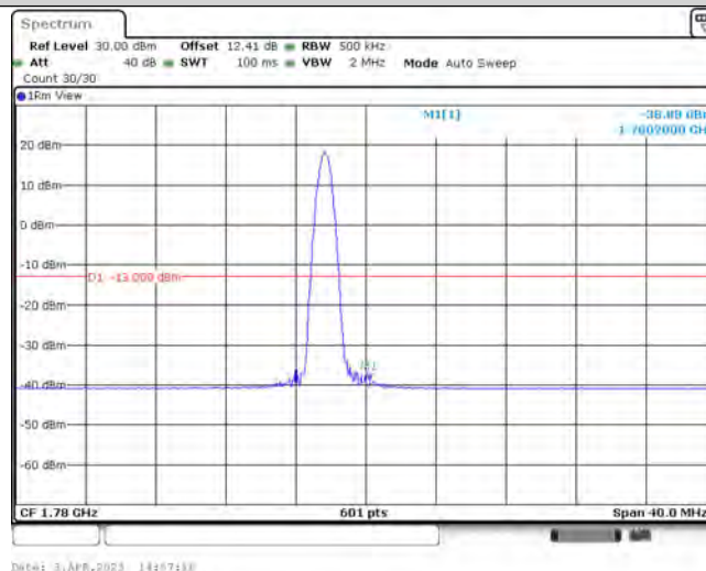
Band66-20MHz-16QAM-132572-1-0-High--38.88-PASS
