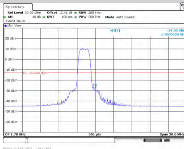
Band66-10MHz-16QAM-132622-6-0-High--28.03-PASS
