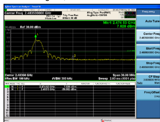
Zigbee, Channel No.: 25
