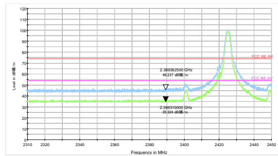
Zigbee-Channel 15: Peak + Average
