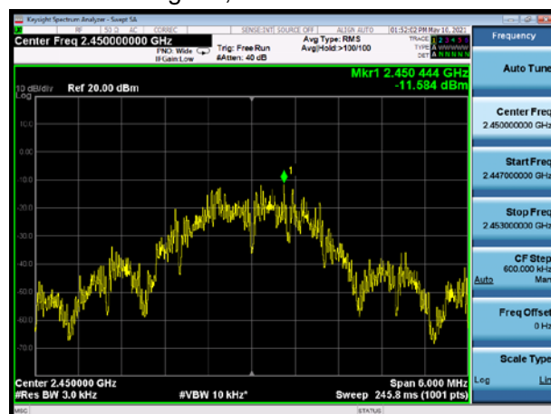
Zigbee, Channel No.: 20
