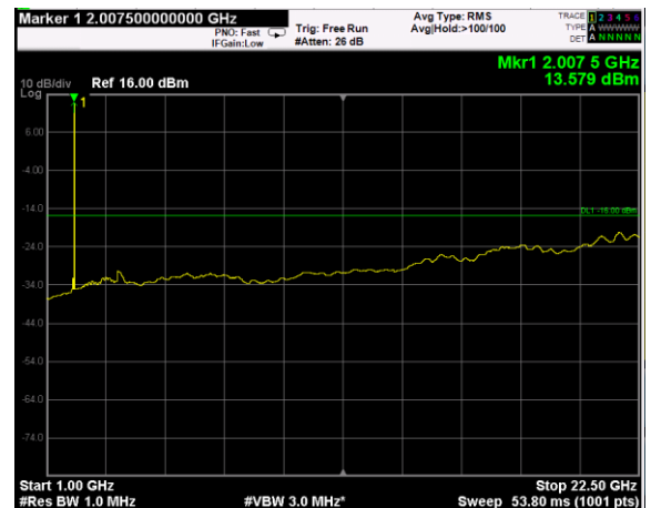
Channel: MIDDLE, Modulation: 256QAM, BW=10MHz, Range: Upper
