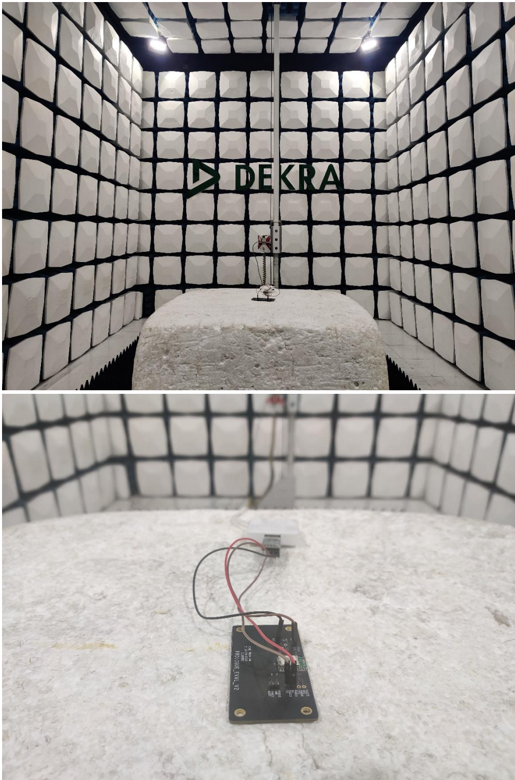
Description: Radiated emission Above 18GHz- Module 2
