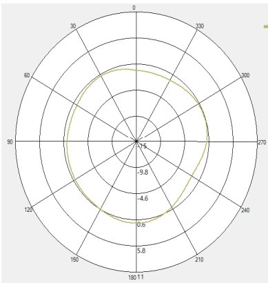
2D Antenna pattern (X->Y;X->Z;Y->Z)
