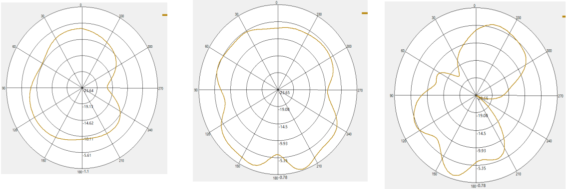
2D Antenna pattern (X->Y;X->Z;Y->Z)
