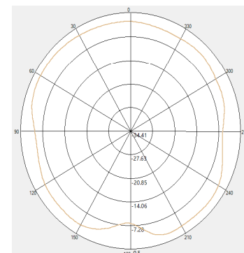
2D Antenna pattern (X→Y;X→Z;Y→Z)
