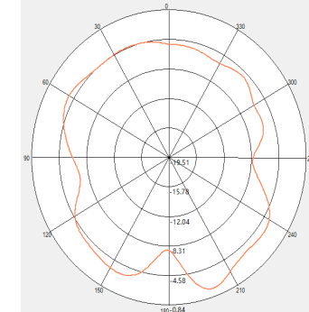
2D Antenna pattern (X→Y;X→Z;Y→Z)
