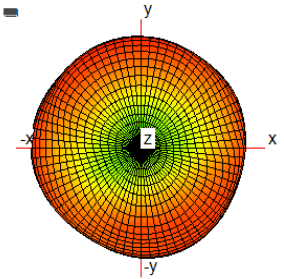
3D Antenna pattern
