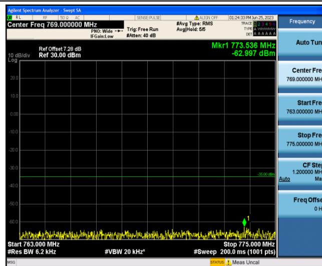
Band13-Stand-Alone-NaN-QPSK-23181-1@0-15kHz-763-775--63--35-PASS
