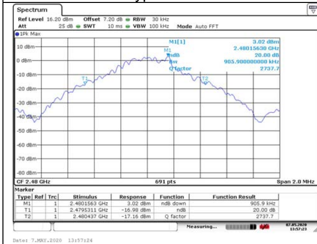
Modulation type: GFSK 2480MHz
