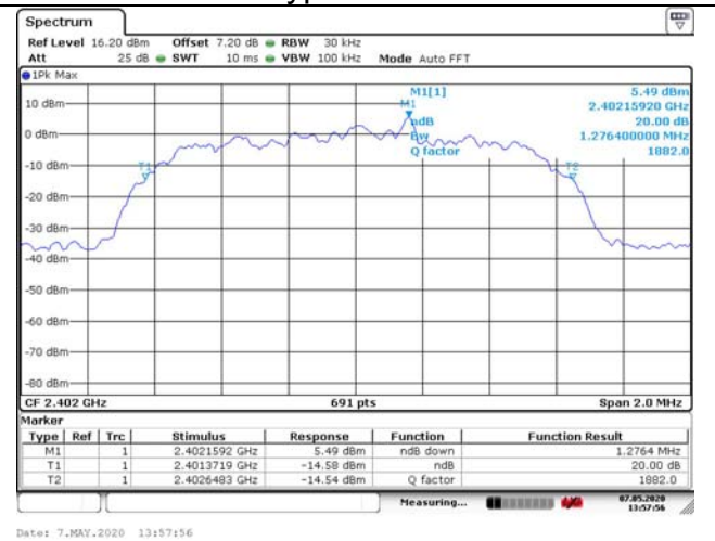
Modulation type: \pi/4 DQPSK 2402MHz
