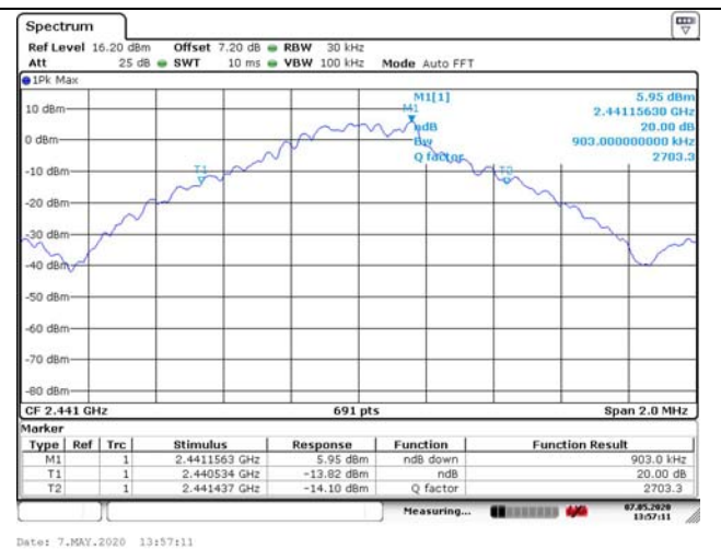
Modulation type: GFSK 2441MHz
