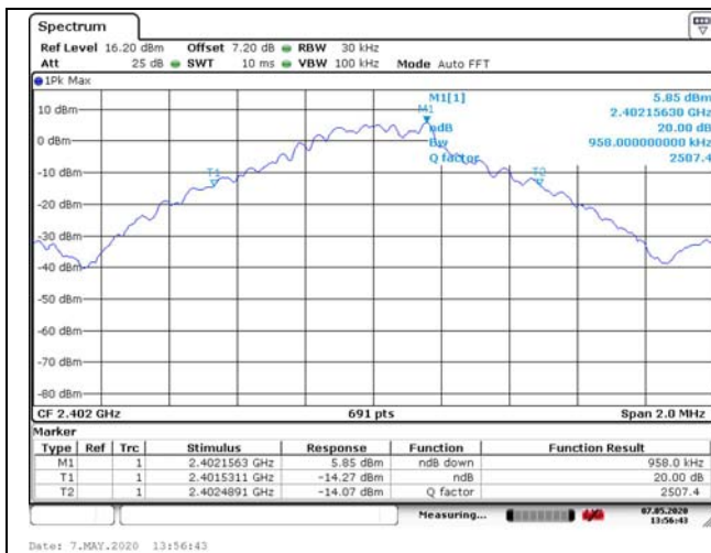
Modulation type: GFSK 2402MHz
