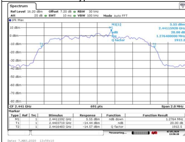
Modulation type: \pi/4 DQPSK 2441MHz
