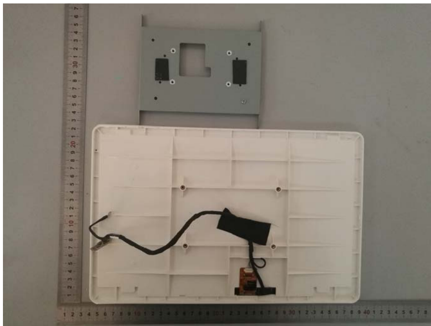
EUT – Cover off View-18
