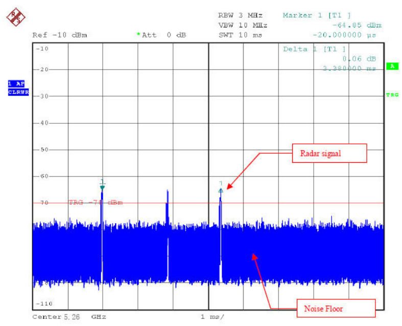
Single Burst of Radar Signal Type 5
