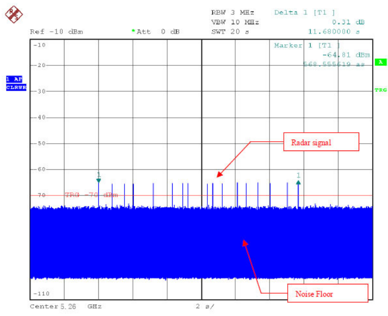
Radar Signal Type 5
