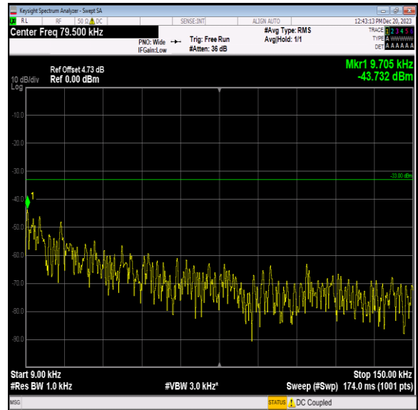
Band5_10MHz_16QAM_20525_1RB#0_0.009~0.15_0.009~0.15
