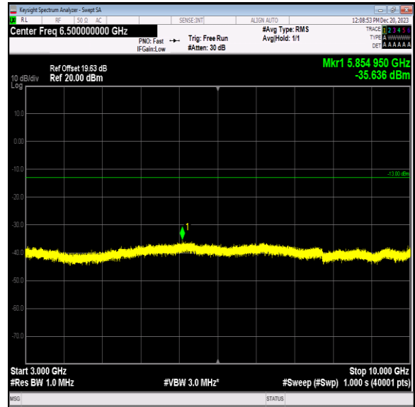
Band5_5MHz_64QAM_20525_1RB#0_3000~10000_3000~10000 000
