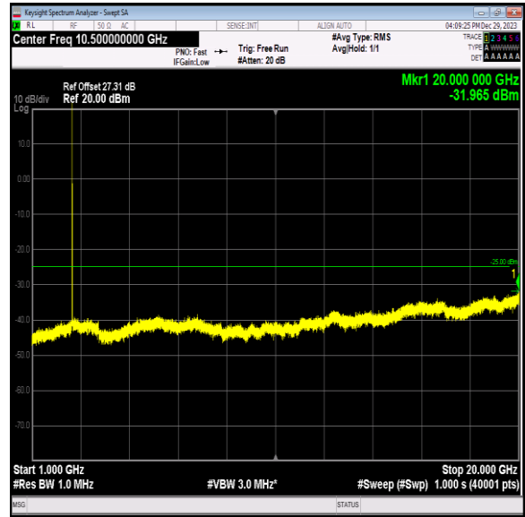
Band7_5MHz_QPSK_21425_1RB#0_1000~20000_1000~20000
