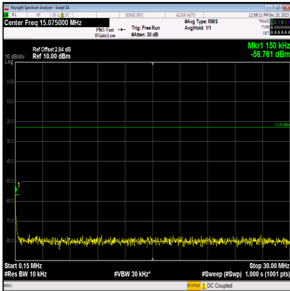
Band5_5MHz_64QAM_20525_1RB#0_0.15~30_0.15~30
