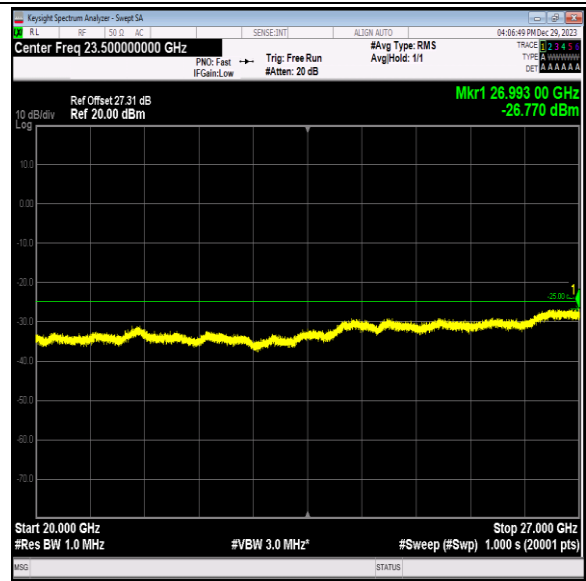
Band7_5MHz_QPSK_21100_1RB#0_20000~27000_20000~27000
