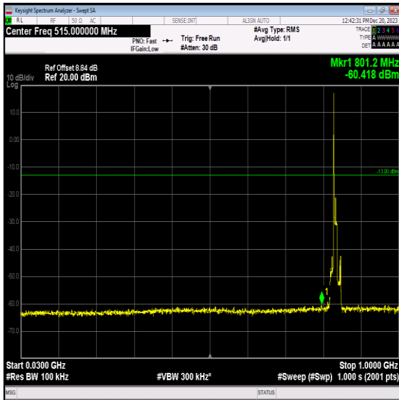
Band5_10MHz_QPSK_20525_1RB#0_30~1000_30~1000
