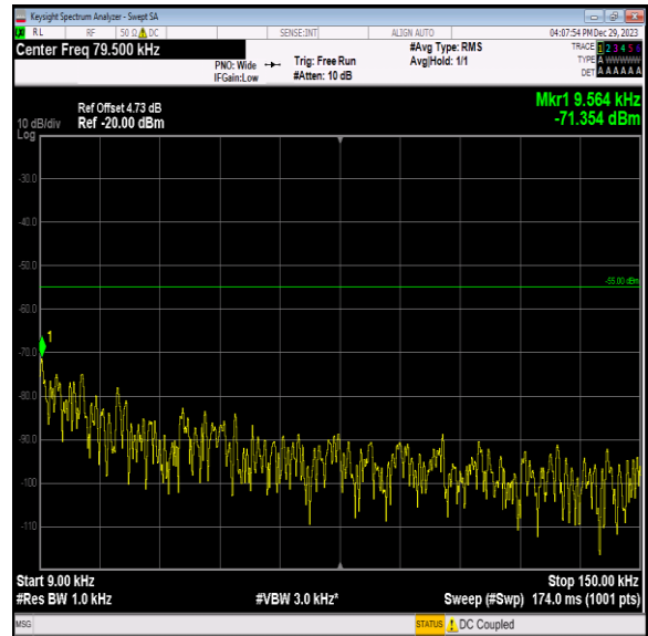
Band7_5MHz_64QAM_21100_1RB#0_0.009~0.15_0.009~0.15
