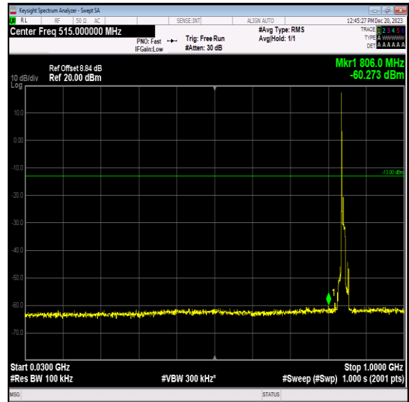
Band5_10MHz_QPSK_20600_1RB#0_30~1000_30~1000
