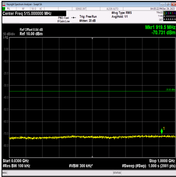
Band7_5MHz_64QAM_20775_1RB#0_30~1000_30~1000
