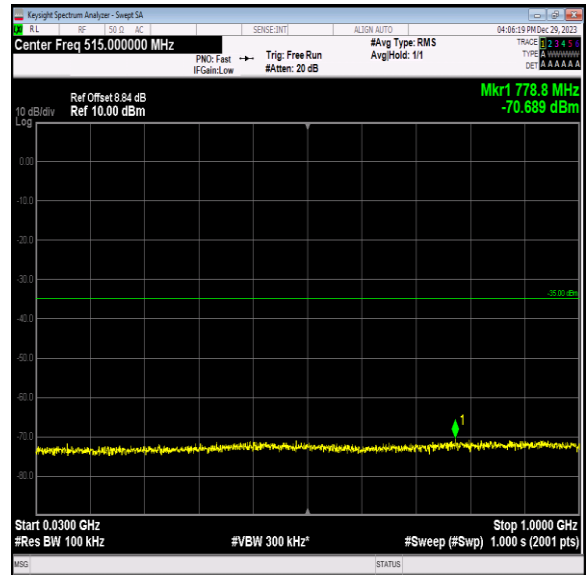
Band7_5MHz_QPSK_21100_1RB#0_30~1000_30~1000
