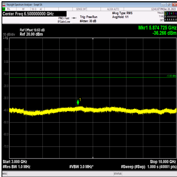
Band5_10MHz_16QAM_20450_1RB#0_3000~10000_3000~10000
