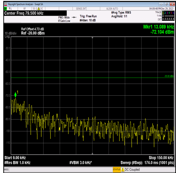
Band7_5MHz_16QAM_21425_1RB#0_0.009~0.15_0.009~0.15
