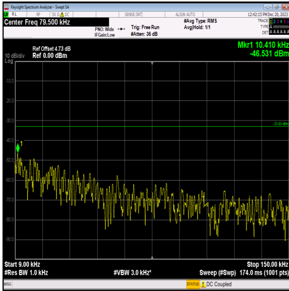
Band5_10MHz_QPSK_20525_1RB#0_0.009~0.15_0.009~0.1 5
