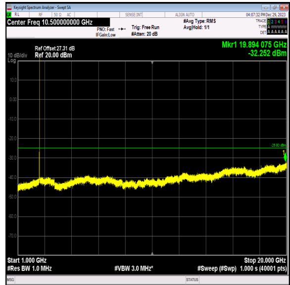
Band7_5MHz_16QAM_21100_1RB#0_1000~20000_1000~20 000
