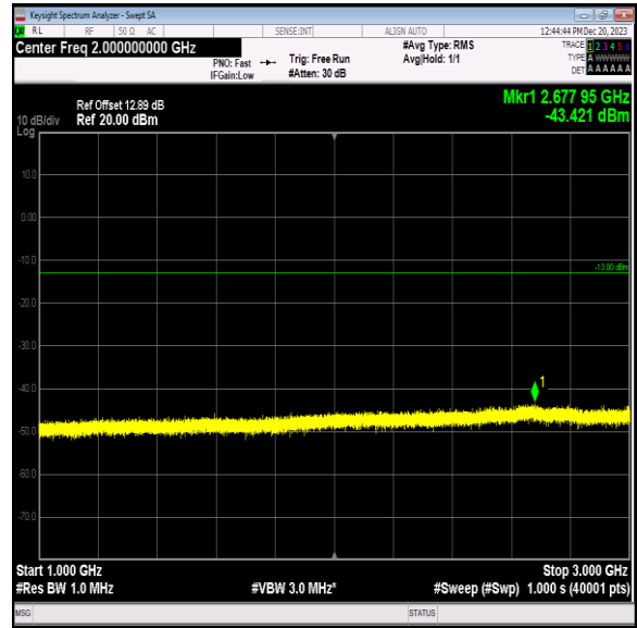
Band5_10MHz_64QAM_20525_1RB#0_1000~3000_1000~3000
