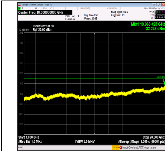
Band7_5MHz_QPSK_21100_1RB#0_1000~20000_1000~20000
