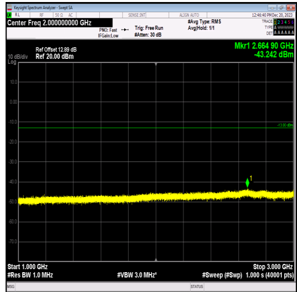
Band5_10MHz_16QAM_20600_1RB#0_1000~3000_1000~3000 00
