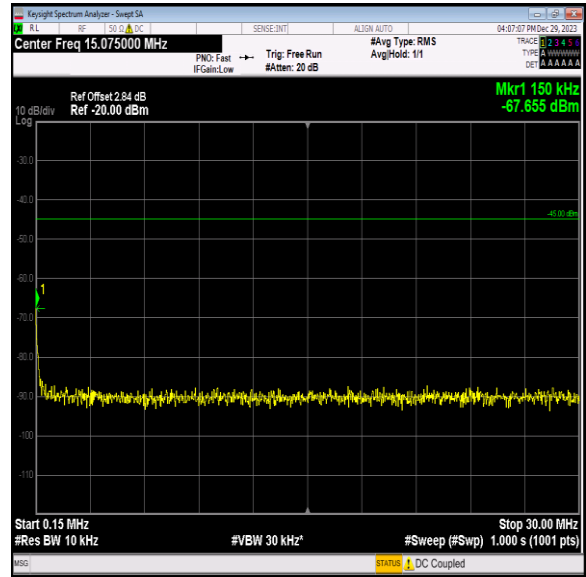
Band7_5MHz_16QAM_21100_1RB#0_0.15~30_0.15~30
