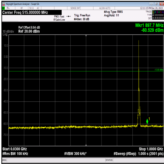
Band5_5MHz_64QAM_20625_1RB#0_30~1000_30~1000
