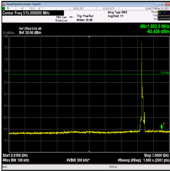
Band5_10MHz_64QAM_20525_1RB#0_30~1000_30~1000
