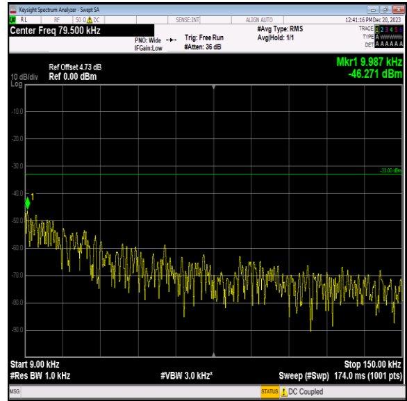
Band5_10MHz_64QAM_20450_1RB#0_0.009~0.15_0.009~0. 15
