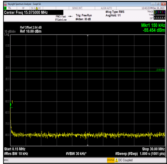
Band5_10MHz_QPSK_20525_1RB#0_0.15~30_0.15~30
