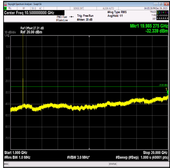
Band7_5MHz_64QAM_20775_1RB#0_1000~20000_1000~20000
