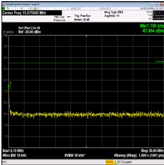
Band7_5MHz_16QAM_21425_1RB#0_0.15~30_0.15~30
