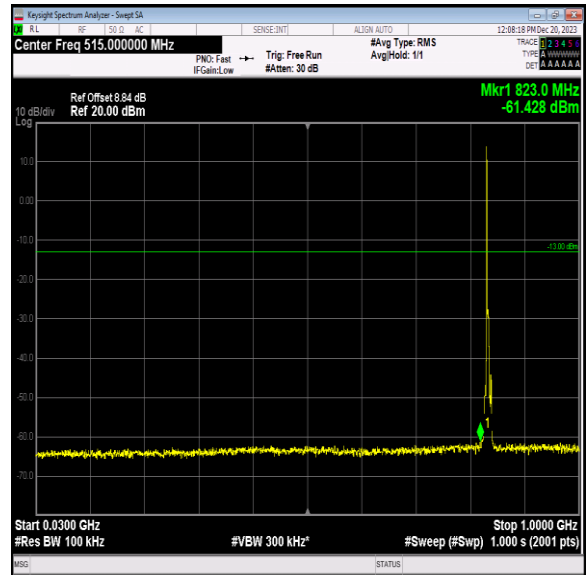
Band5_5MHz_64QAM_20525_1RB#0_30~1000_30~1000
