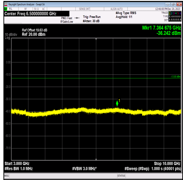
Band5_10MHz_QPSK_20600_1RB#0_3000~10000_3000~10 000
