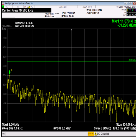
Band7_5MHz_16QAM_21100_1RB#0_0.009~0.15_0.009~0.1 5
