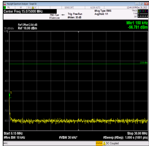
Band5_10MHz_64QAM_20525_1RB#0_0.15~30_0.15~30
