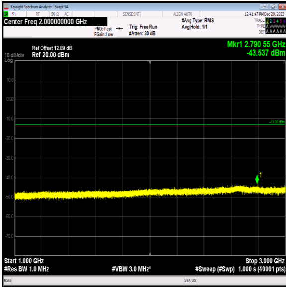
Band5_10MHz_64QAM_20450_1RB#0_1000~3000_1000~30 00
