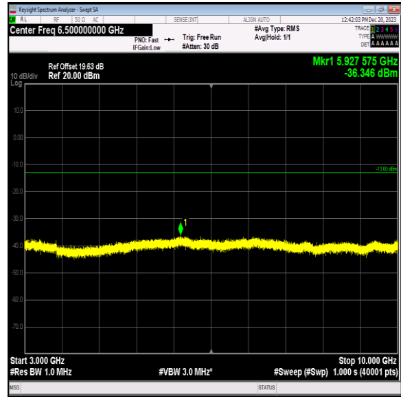
Band5_10MHz_64QAM_20450_1RB#0_3000~10000_3000~1 0000
