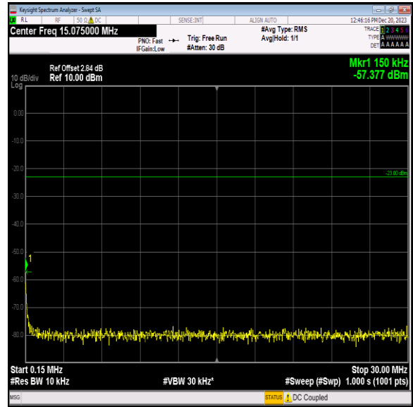
Band5_10MHz_16QAM_20600_1RB#0_0.15~30_0.15~30
