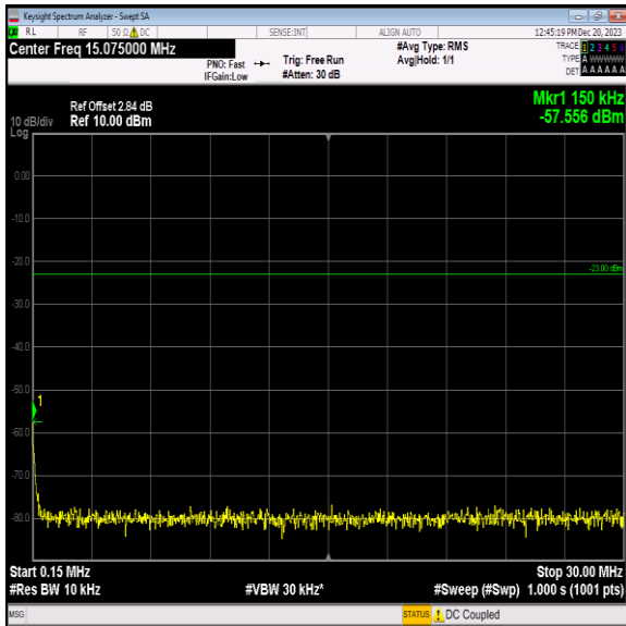
Band5_10MHz_QPSK_20600_1RB#0_0.15~30_0.15~30
