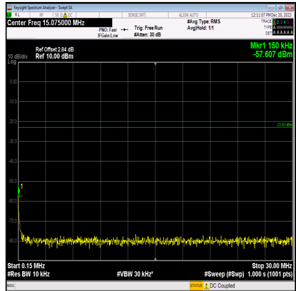
Band5_5MHz_64QAM_20625_1RB#0_0.15~30_0.15~30
