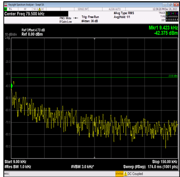
Band5_10MHz_QPSK_20450_1RB#0_0.009~0.15_0.009~0.15 5
