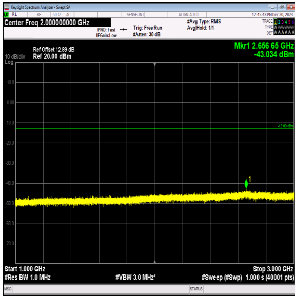
Band5_10MHz_QPSK_20600_1RB#0_1000~3000_1000~300 0
