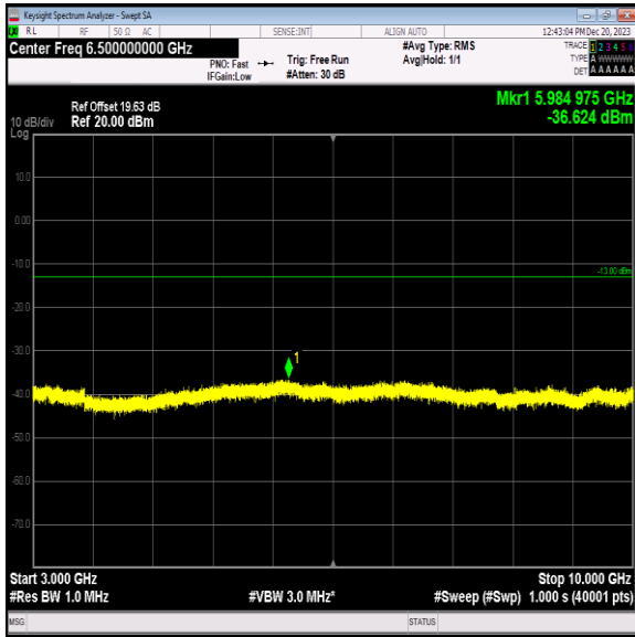
Band5_10MHz_QPSK_20525_1RB#0_3000~10000_3000~10000
