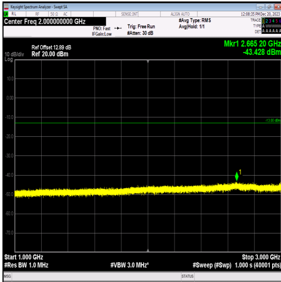
Band5_5MHz_64QAM_20525_1RB#0_1000~3000_1000~3000 0
