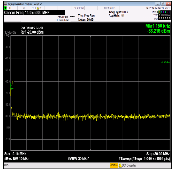
Band7_5MHz_64QAM_20775_1RB#0_0.15~30_0.15~30
