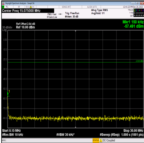
Band5_10MHz_64QAM_20450_1RB#0_0.15~30_0.15~30
