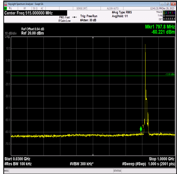
Band5_10MHz_64QAM_20450_1RB#0_30~1000_30~1000
