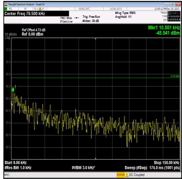
Band5_10MHz_QPSK_20600_1RB#0_0.009~0.15_0.009~0.15
