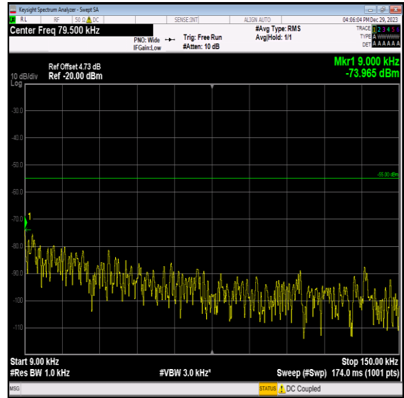
Band7_5MHz_QPSK_21100_1RB#0_0.009~0.15_0.009~0.15
