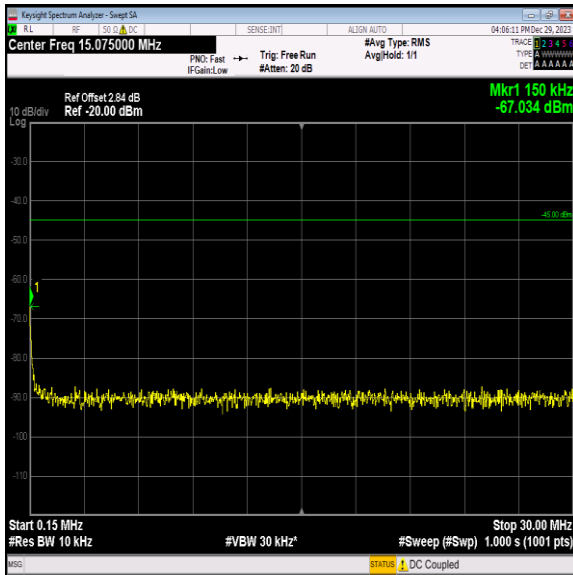
Band7_5MHz_QPSK_21100_1RB#0_0.15~30_0.15~30
