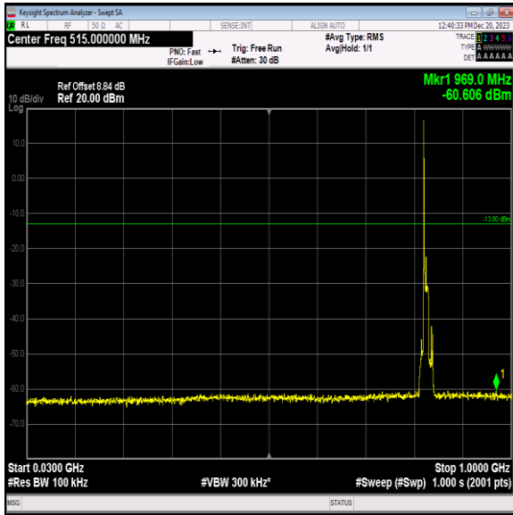
Band5_10MHz_16QAM_20450_1RB#0_30~1000_30~1000
