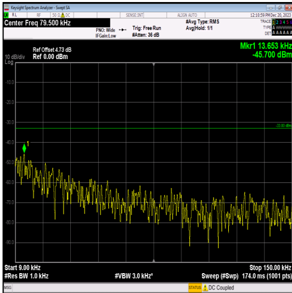
Band5_5MHz_64QAM_20625_1RB#0_0.009~0.15_0.009~0.15 5
