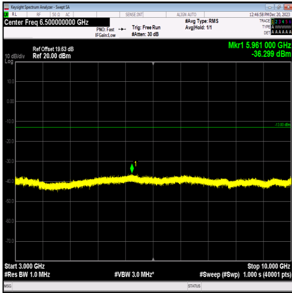
Band5_10MHz_16QAM_20600_1RB#0_3000~10000_3000~1 0000
