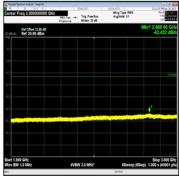
Band5_5MHz_64QAM_20625_1RB#0_1000~3000_1000~3000 0
