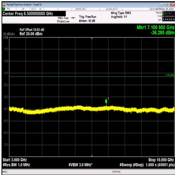
Band5_5MHz_64QAM_20625_1RB#0_3000~10000_3000~10000
