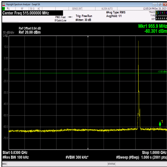
Band5_5MHz_64QAM_20425_1RB#0_30~1000_30~1000
