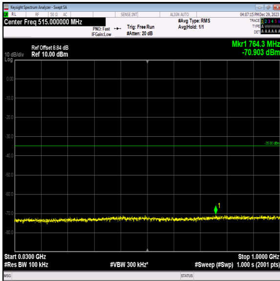
Band7_5MHz_16QAM_21100_1RB#0_30~1000_30~1000
