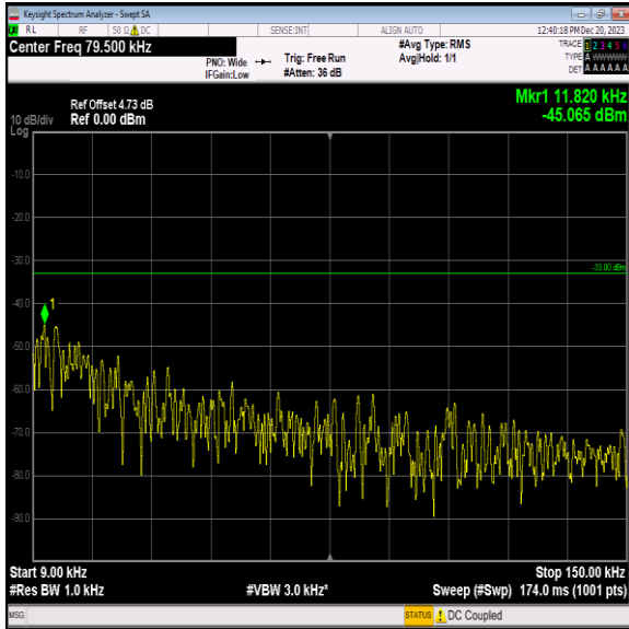
Band5_10MHz_16QAM_20450_1RB#0_0.009~0.15_0.009~0. 15
