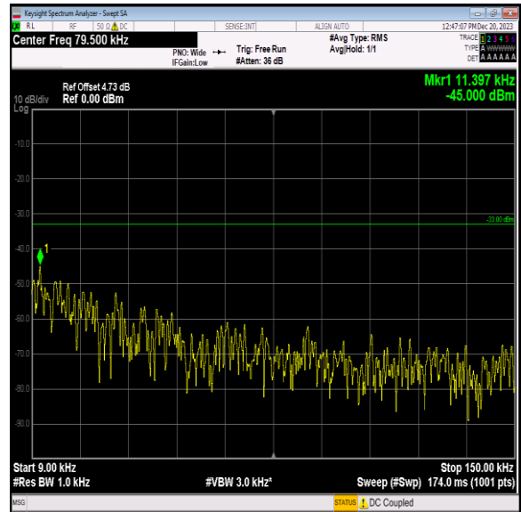
Band5_10MHz_64QAM_20600_1RB#0_0.009~0.15_0.009~0.15
