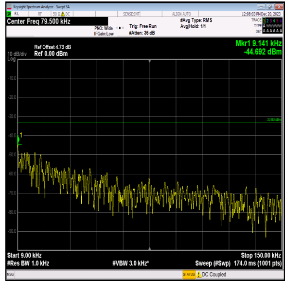
Band5_5MHz_64QAM_20525_1RB#0_0.009~0.15_0.009~0.15
