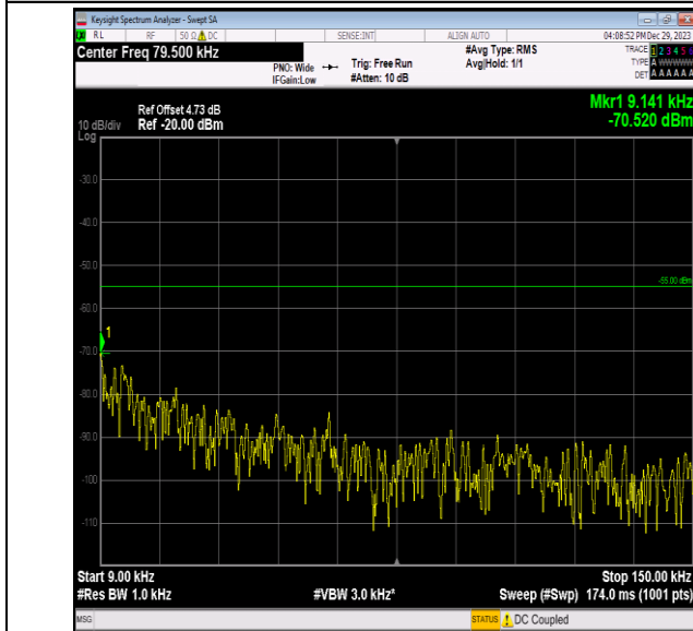
Band7_5MHz_QPSK_21425_1RB#0_0.009~0.15_0.009~0.15
