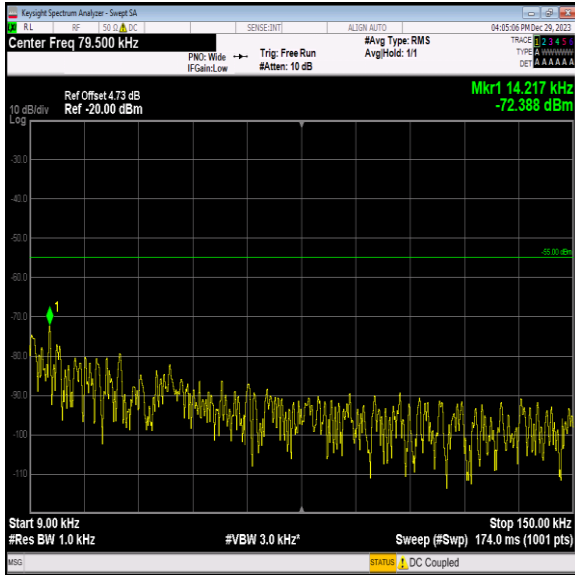
Band7_5MHz_64QAM_20775_1RB#0_0.009~0.15_0.009~0.15
