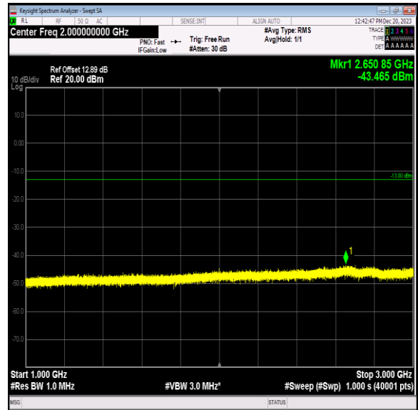
Band5_10MHz_QPSK_20525_1RB#0_1000~3000_1000~300 0
