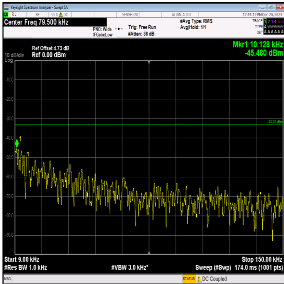
Band5_10MHz_64QAM_20525_1RB#0_0.009~0.15_0.009~0. 15
