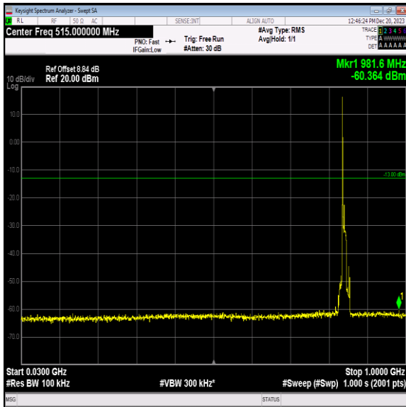
Band5_10MHz_16QAM_20600_1RB#0_30~1000_30~1000
