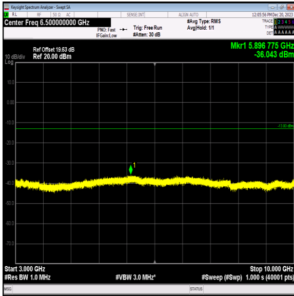
Band5_5MHz_64QAM_20425_1RB#0_3000~10000_3000~10000
