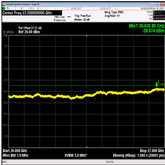
Band7_5MHz_QPSK_21425_1RB#0_20000~27000_20000~27000
