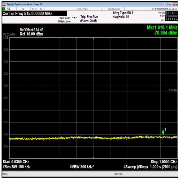
Band7_5MHz_QPSK_21425_1RB#0_30~1000_30~1000
