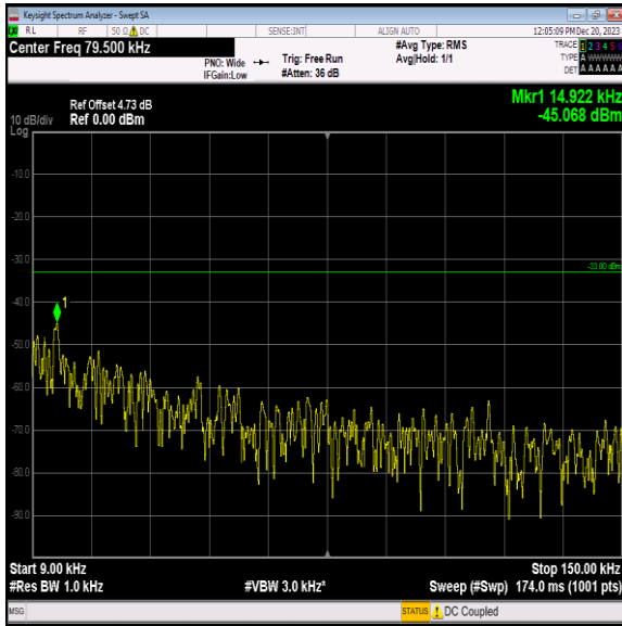
Band5_5MHz_64QAM_20425_1RB#0_0.009~0.15_0.009~0.1 5
