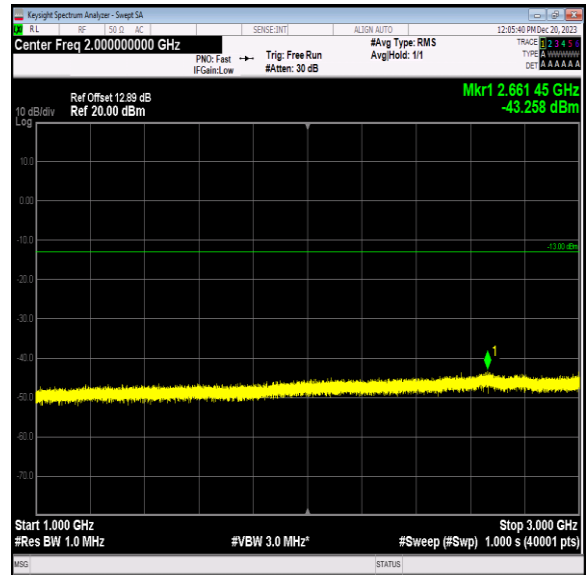
Band5_5MHz_64QAM_20425_1RB#0_1000~3000_1000~300 0
