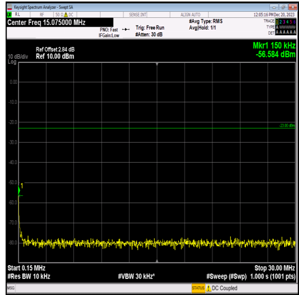
Band5_5MHz_64QAM_20425_1RB#0_0.15~30_0.15~30
