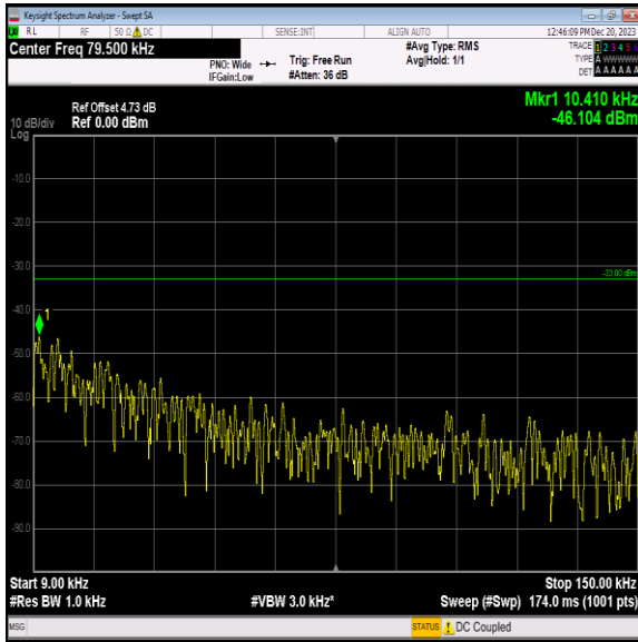
Band5_10MHz_16QAM_20600_1RB#0_0.009~0.15_0.009~0.15 15
