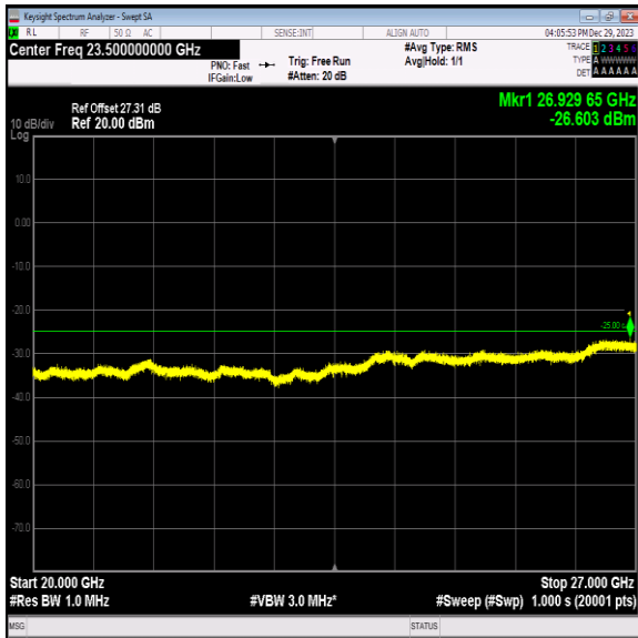
Band7_5MHz_64QAM_20775_1RB#0_20000~27000_20000~27000
