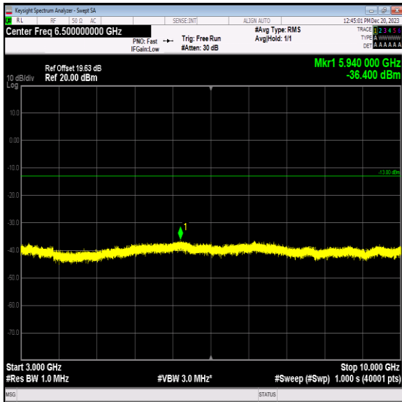
Band5_10MHz_64QAM_20525_1RB#0_3000~10000_3000~10000
