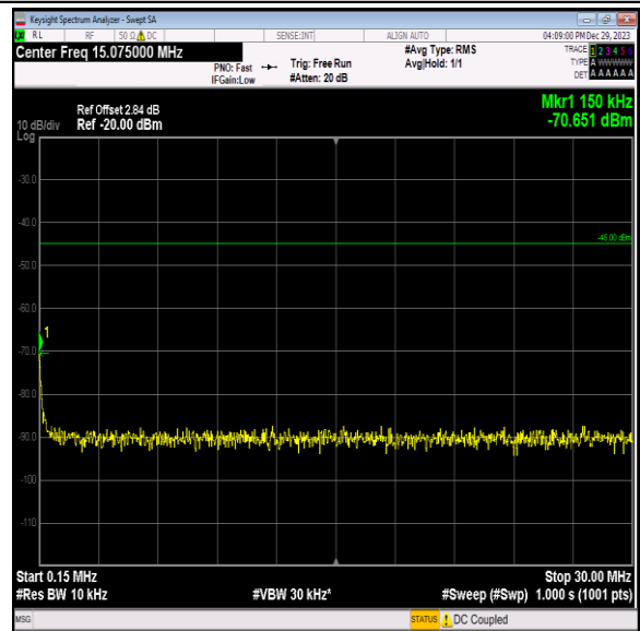
Band7_5MHz_QPSK_21425_1RB#0_0.15~30_0.15~30
