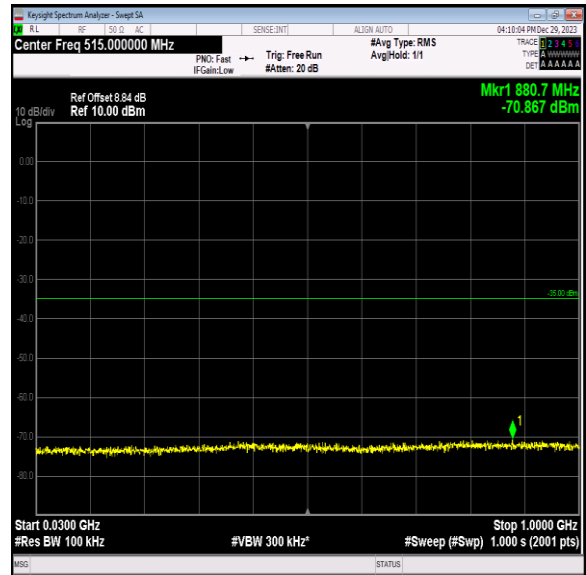
Band7_5MHz_16QAM_21425_1RB#0_30~1000_30~1000
