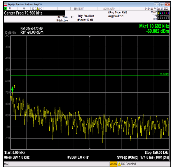
Band7_5MHz_16QAM_20775_1RB#0_0.009~0.15_0.009~0.15
