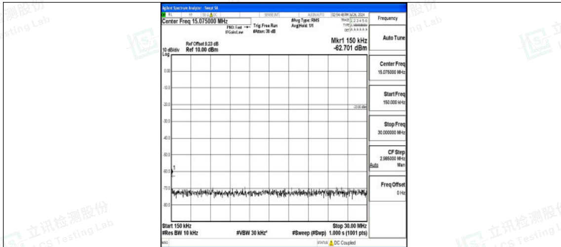
Band5-3MHz-16QAM-20415-1RB#0-0.15~30-PASS
