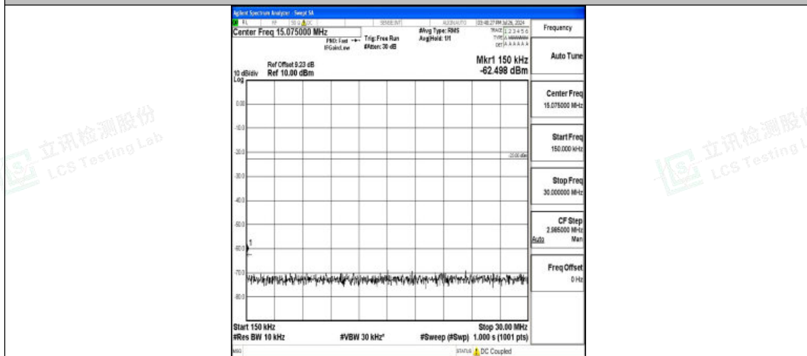
Band5-10MHz-QPSK-20525-1RB#0-0.15~30-PASS
