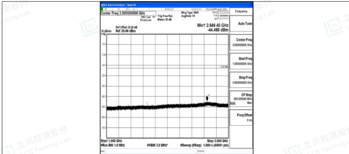
Band5-5MHz-16QAM-20525-1RB#0-1000~3000-PASS
