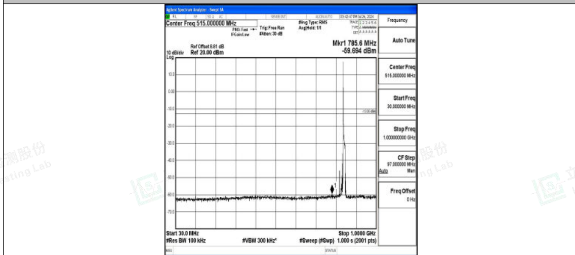
Band5-10MHz-QPSK-20600-1RB#0-30~1000-PASS
