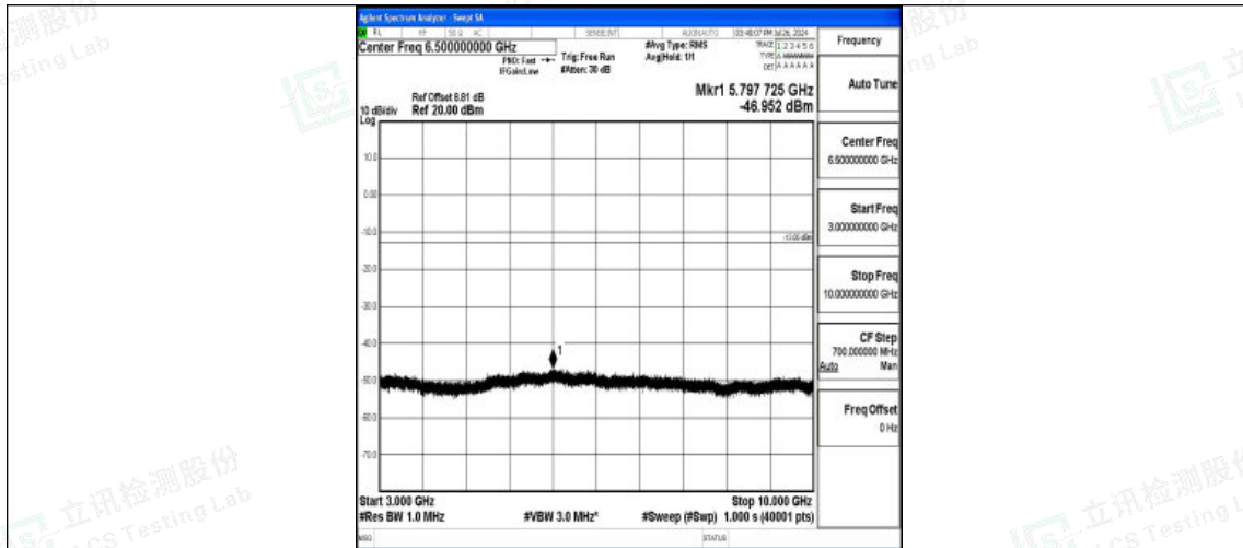
Band5-10MHz-16QAM-20450-1RB#0-3000~10000-PASS
