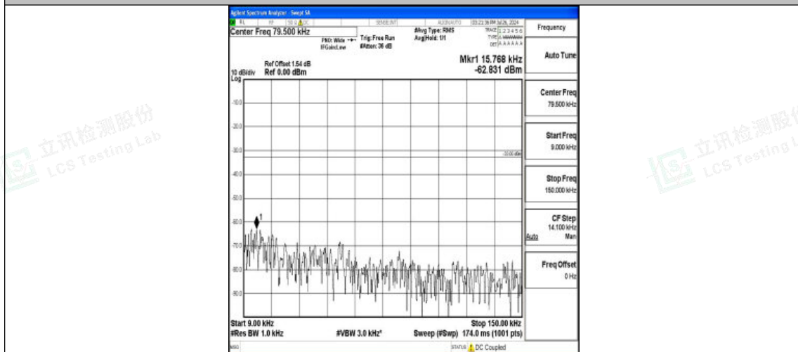
Band5-5MHz-QPSK-20625-1RB#0-0.009~0.15-PASS
