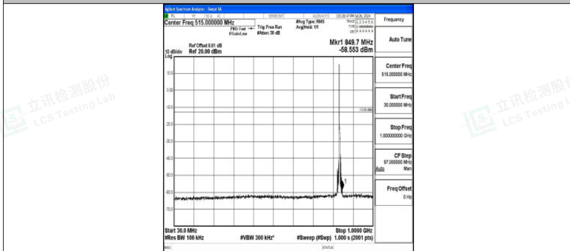
Band5-5MHz-16QAM-20525-1RB#0-30~1000-PASS
