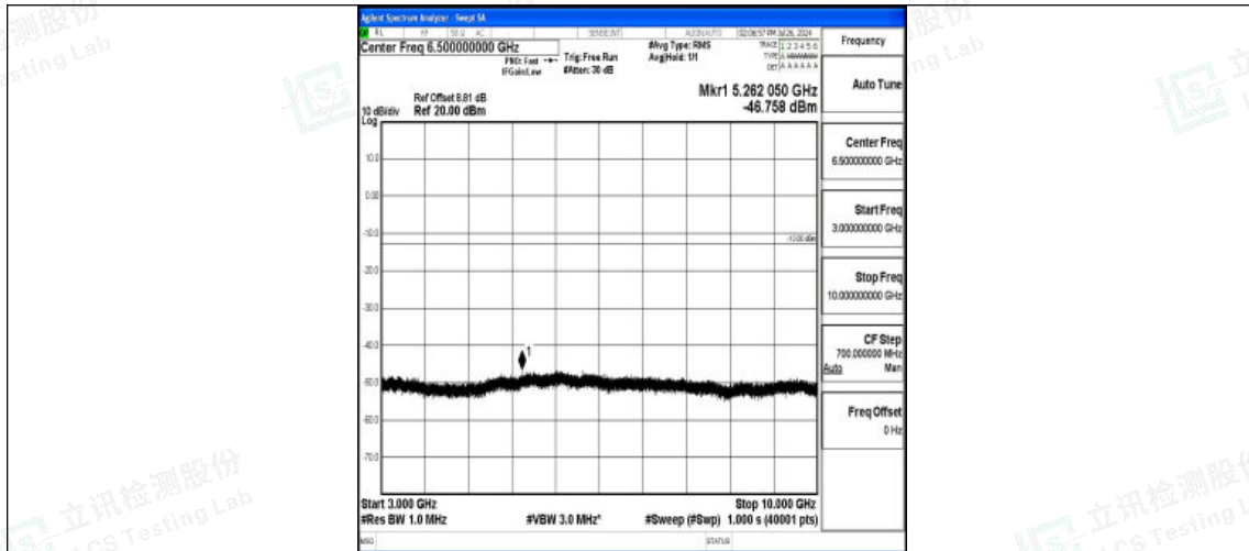
Band5-1.4MHz-QPSK-20643-1RB#0-3000~10000-PASS
