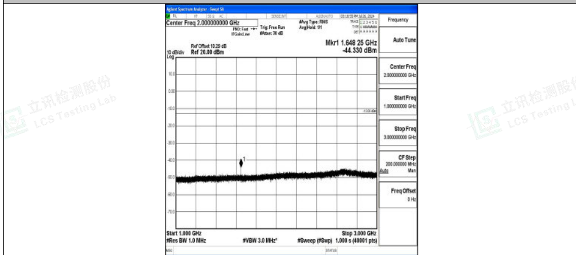
Band5-5MHz-16QAM-20425-1RB#0-1000~3000-PASS
