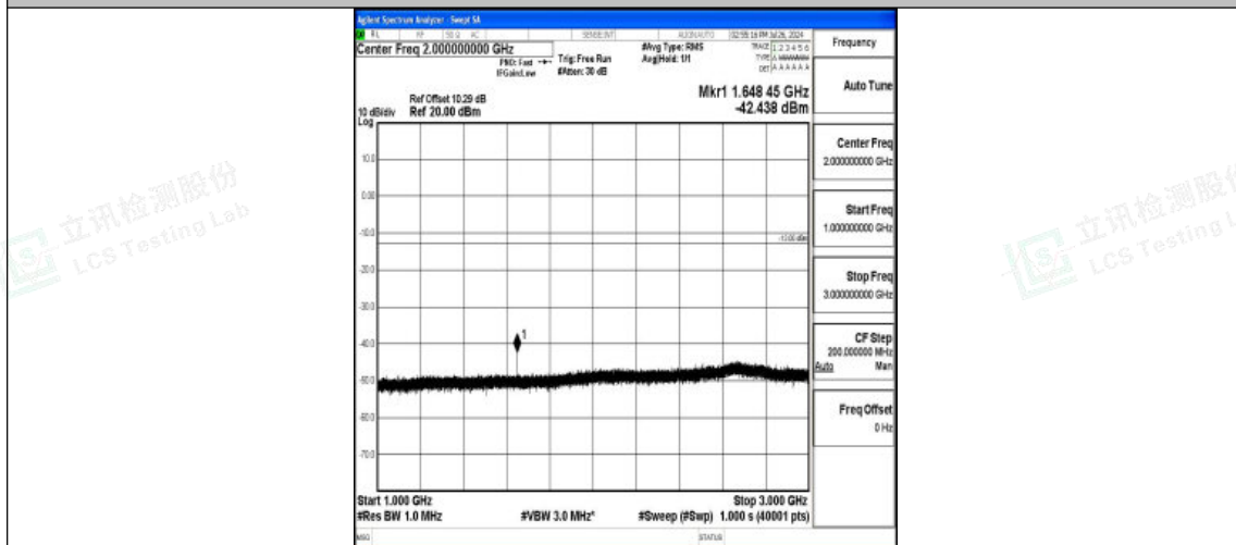
Band5-3MHz-16QAM-20415-1RB#0-1000~3000-PASS
