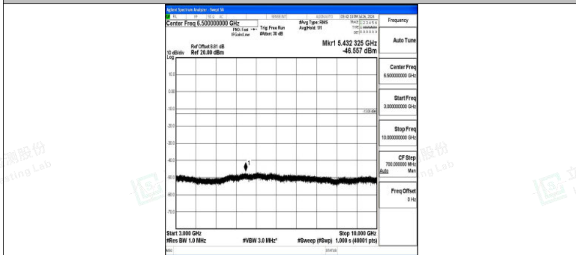
Band5-10MHz-16QAM-20525-1RB#0-3000~10000-PASS
