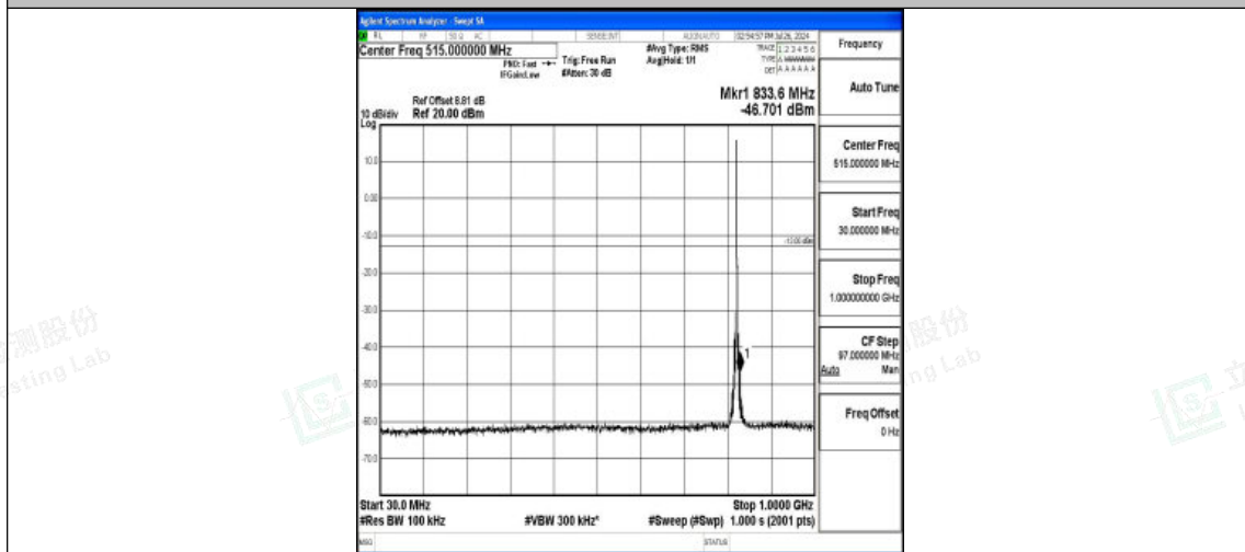
Band5-3MHz-16QAM-20415-1RB#0-30~1000-PASS
