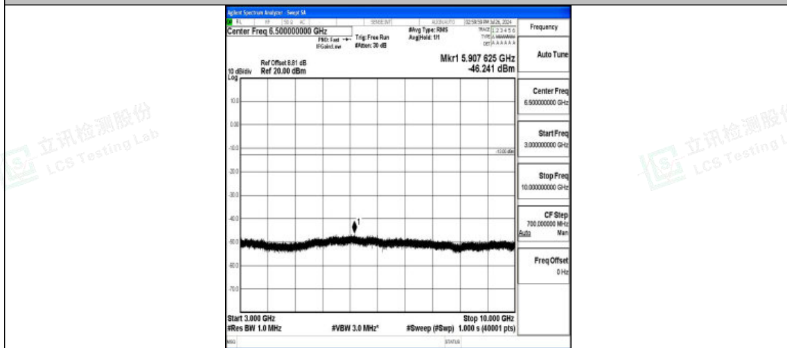
Band5-3MHz-16QAM-20635-1RB#0-3000~10000-PASS
