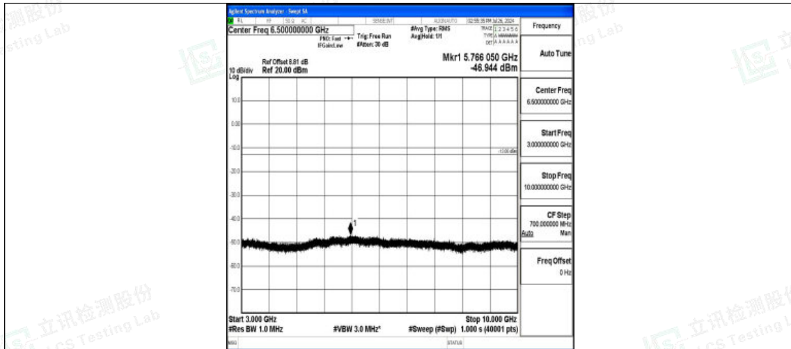
Band5-3MHz-16QAM-20415-1RB#0-3000~10000-PASS
