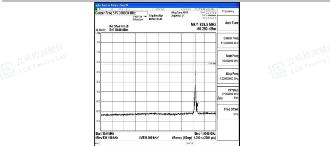
Band5-5MHz-QPSK-20425-1RB#0-30~1000-PASS
