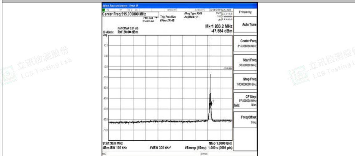
Band5-3MHz-QPSK-20415-1RB#0-30~1000-PASS
