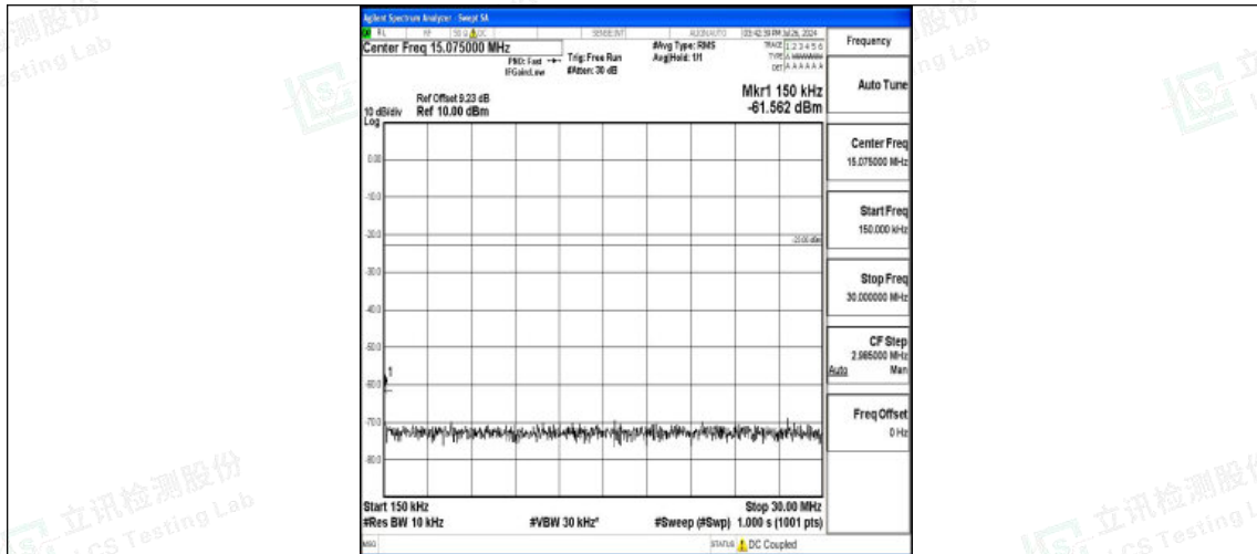
Band5-10MHz-QPSK-20600-1RB#0-0.15~30-PASS
