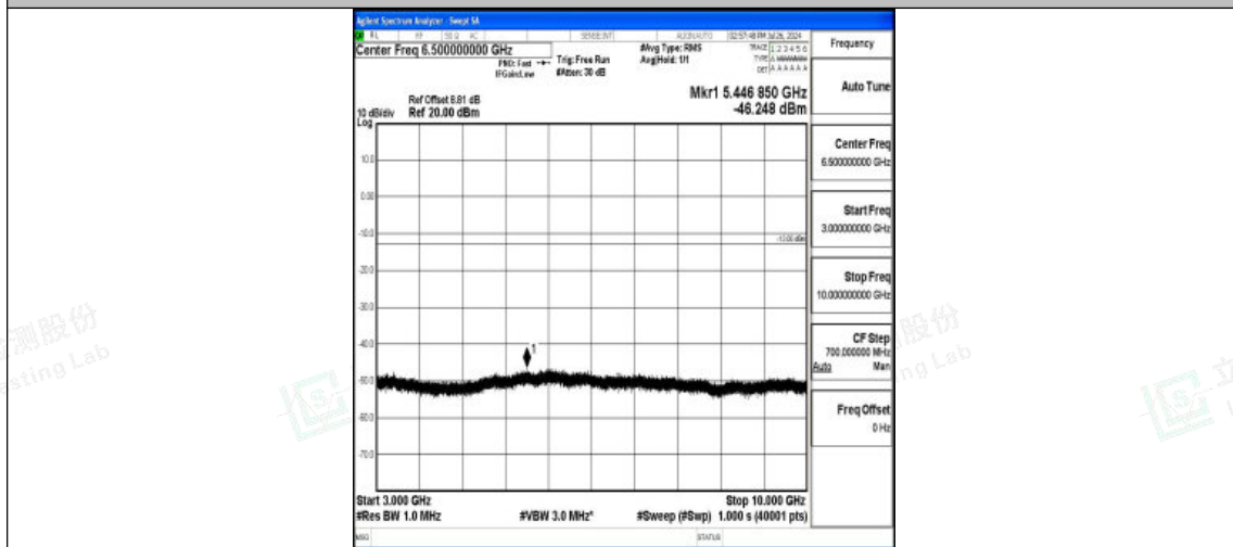
Band5-3MHz-16QAM-20525-1RB#0-3000~10000-PASS
