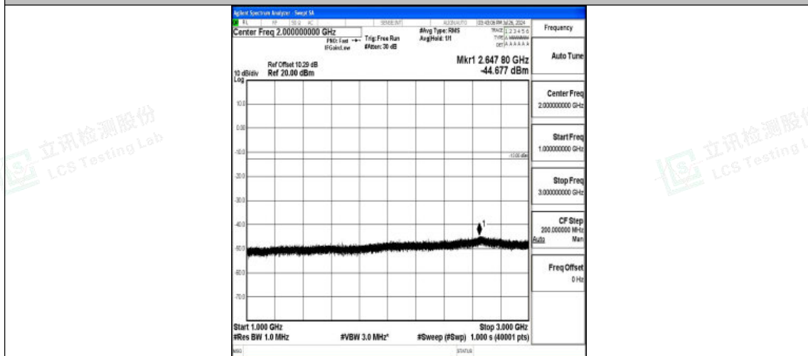
Band5-10MHz-QPSK-20600-1RB#0-1000~3000-PASS
