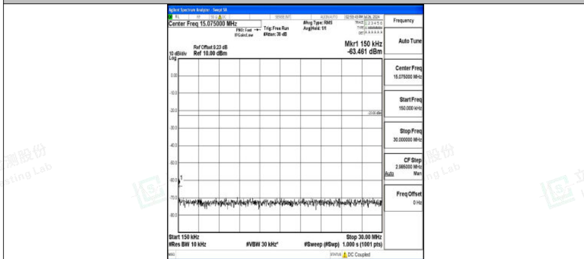
Band5-3MHz-QPSK-20415-1RB#0-0.15~30-PASS
