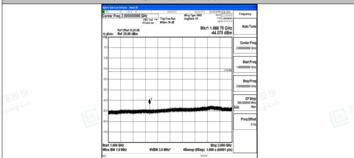
Band5-5MHz-QPSK-20525-1RB#0-1000~3000-PASS
