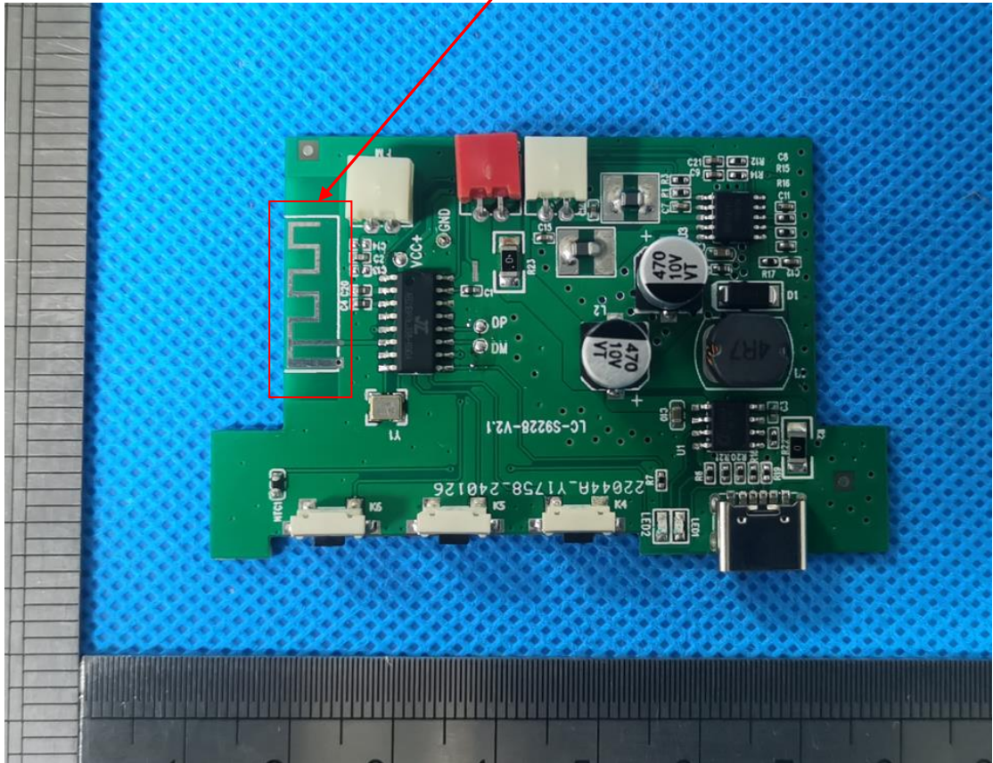
BT antenna
