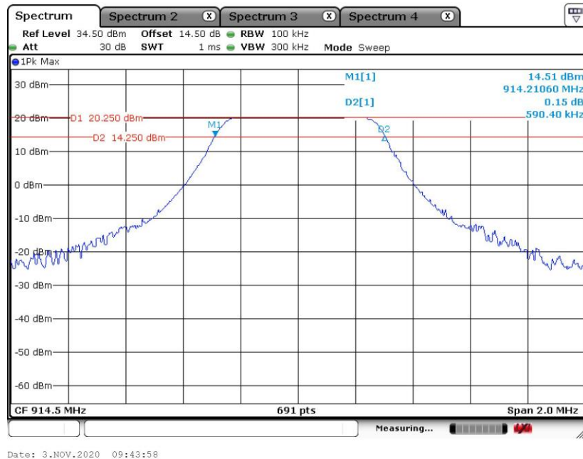
6 dB Bandwidth Plot on 914.5 MHz
