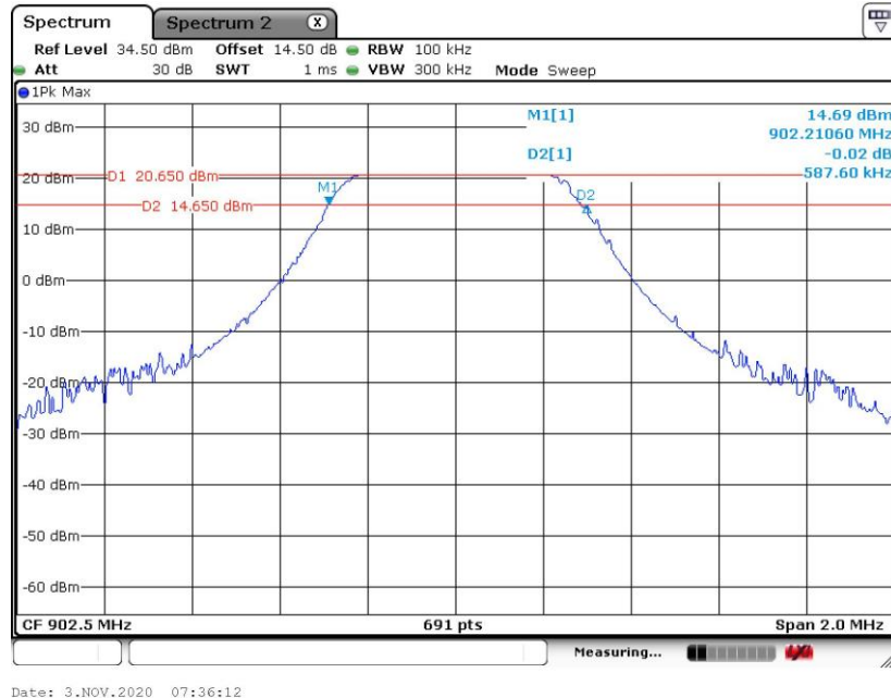
6 dB Bandwidth Plot on 902.5MHz
