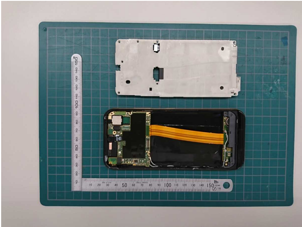
Chassis open 2, Battery
