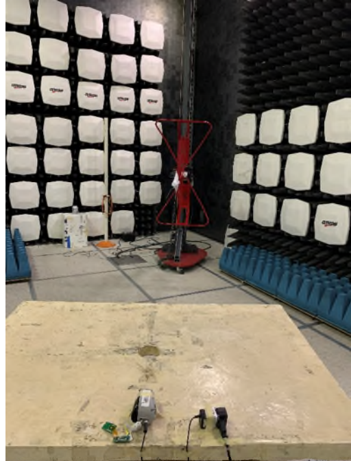
30MHz – 1GHz
