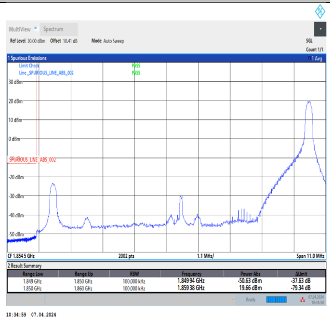
Band2_10MHz_64QAM_18650_1RB#49
