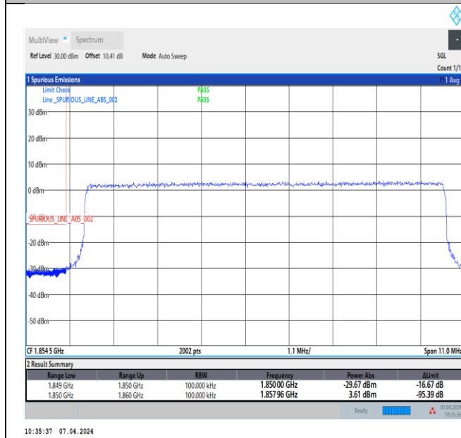
Band2_10MHz_16QAM_18650_50RB#0
