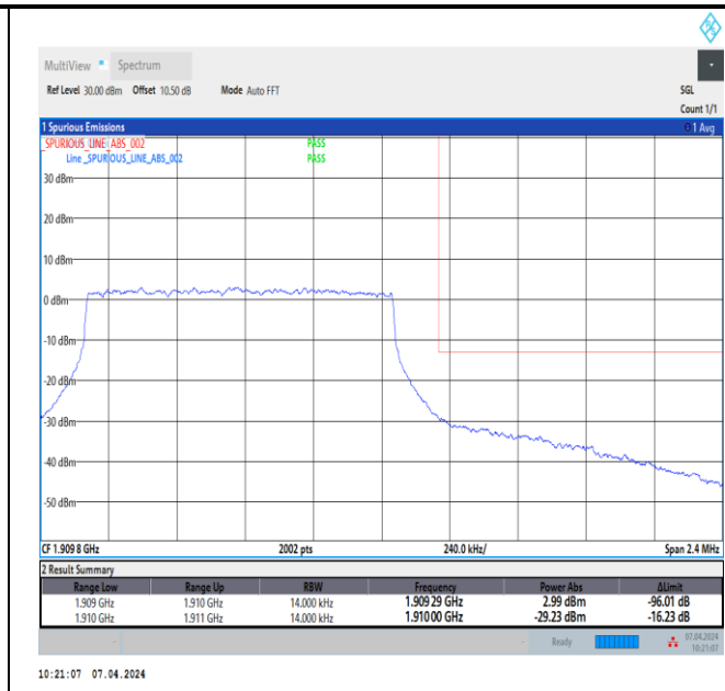
Band2_1.4MHz_64QAM_19193_6RB#0
