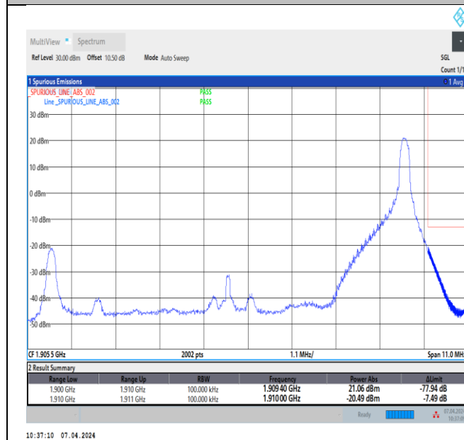
Band2_10MHz_QPSK_19150_1RB#49
