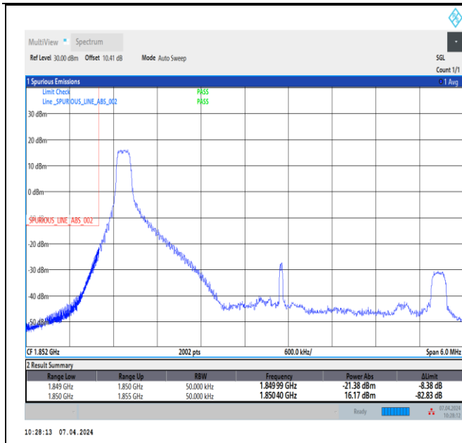
Band2_5MHz_64QAM_18625_1RB#0
