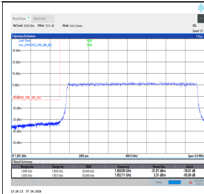
Band2_3MHz_64QAM_18615_15RB#0
