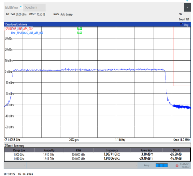
Band2_10MHz_16QAM_19150_50RB#0
