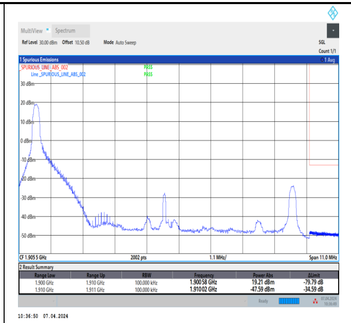
Band2_10MHz_64QAM_19150_1RB#0
