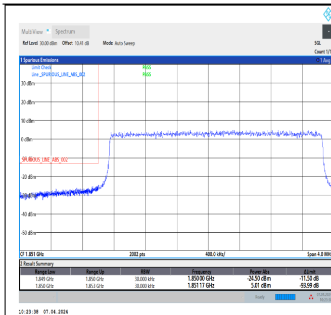
Band2_3MHz_QPSK_18615_15RB#0
