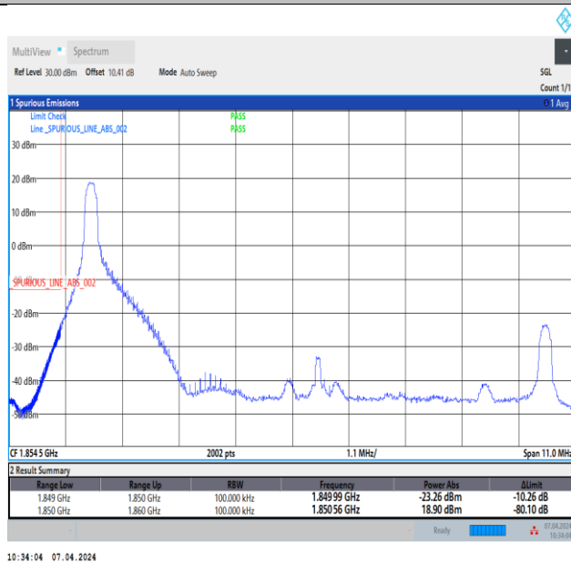
Band2_10MHz_64QAM_18650_1RB#0
