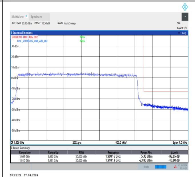
Band2_3MHz_QPSK_19185_15RB#0
