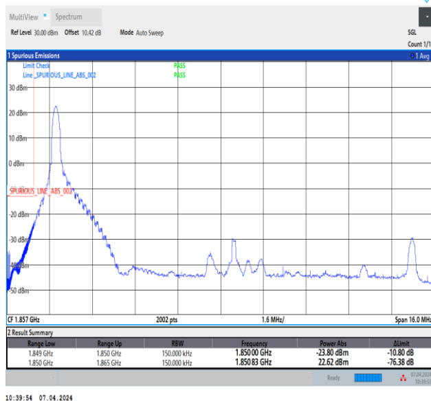
Band2_15MHz_QPSK_18675_1RB#0
