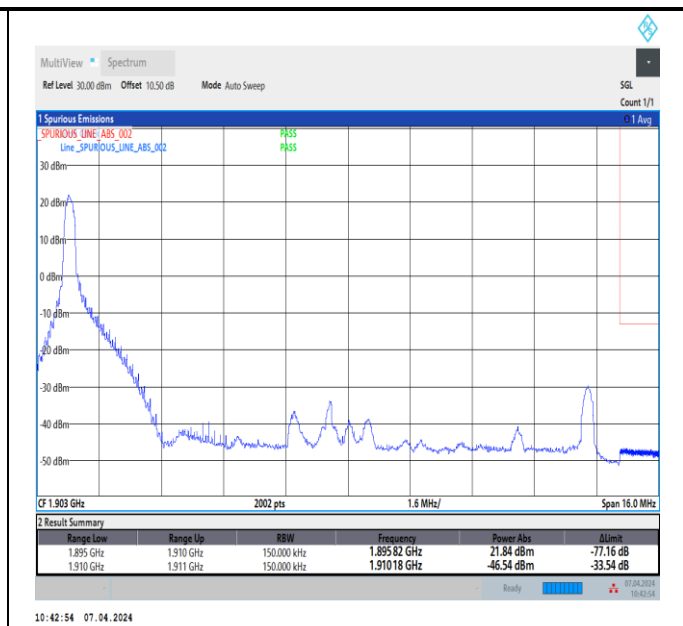
Band2_15MHz_16QAM_19125_1RB#0
