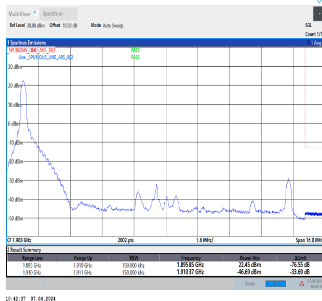
Band2_15MHz_QPSK_19125_1RB#0
