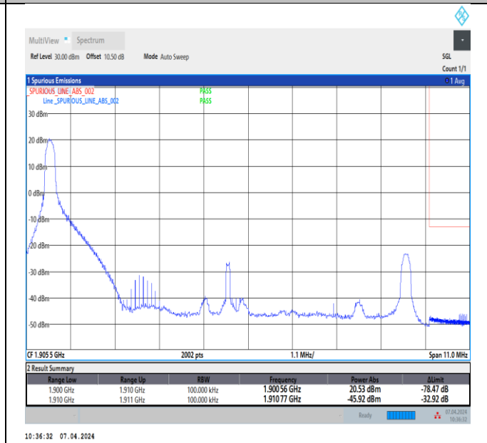
Band2_10MHz_16QAM_19150_1RB#0
