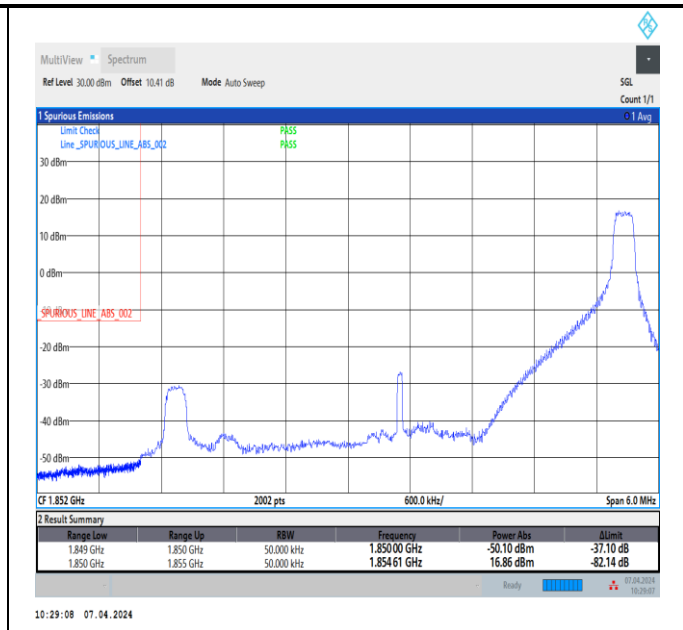
Band2_5MHz_64QAM_18625_1RB#24
