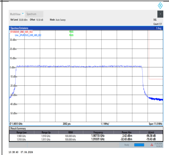
Band2_10MHz_64QAM_19150_50RB#0
