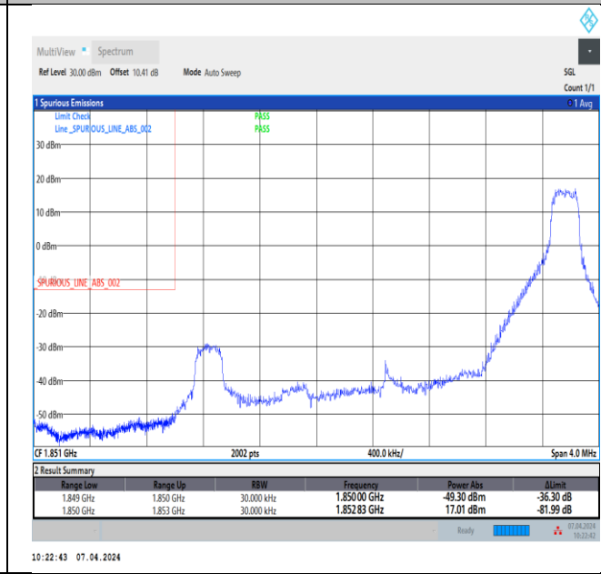
Band2_3MHz_QPSK_18615_1RB#14
