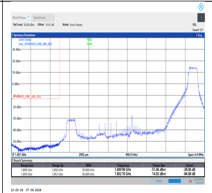
Band2_3MHz_64QAM_18615_1RB#14
