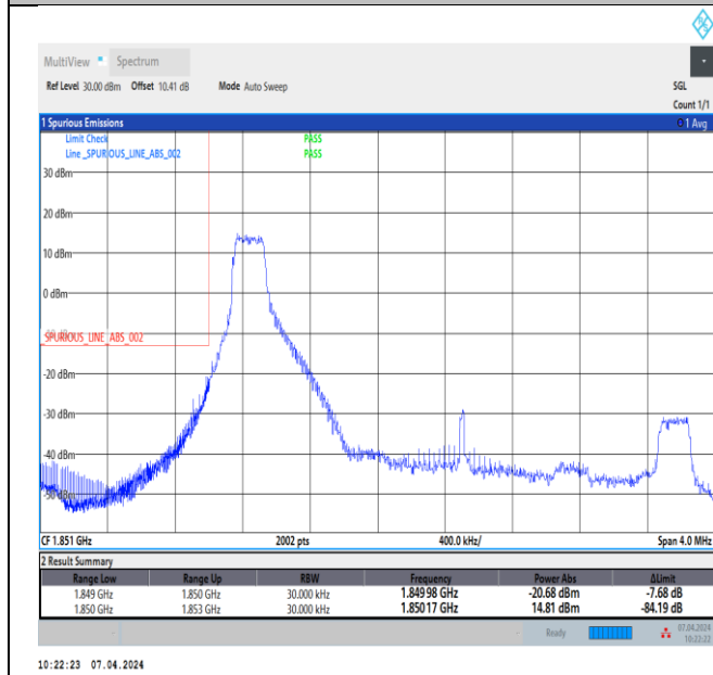
Band2_3MHz_64QAM_18615_1RB#0
