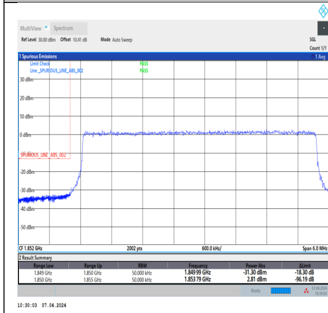
Band2_5MHz_64QAM_18625_25RB#0
