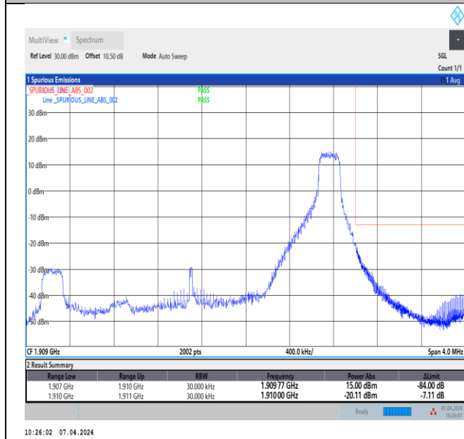
Band2_3MHz_64QAM_19185_1RB#14
