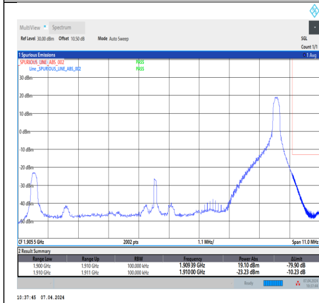
Band2_10MHz_64QAM_19150_1RB#49
