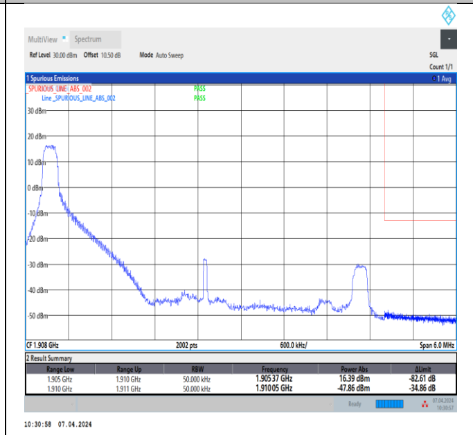
Band2_5MHz_64QAM_19175_1RB#0
