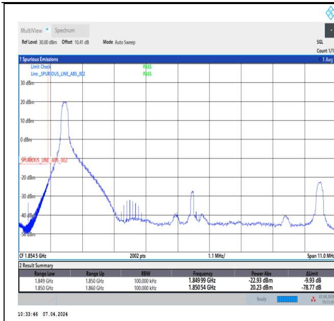
Band2_10MHz_16QAM_18650_1RB#0
