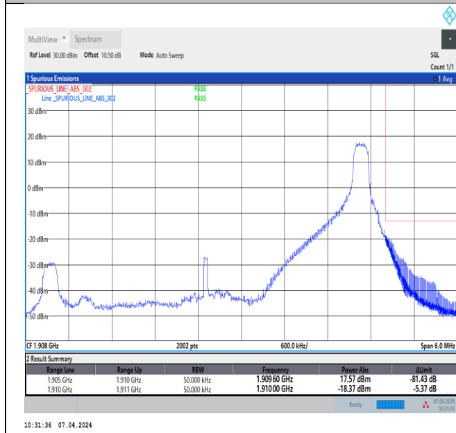
Band2_5MHz_16QAM_19175_1RB#24
