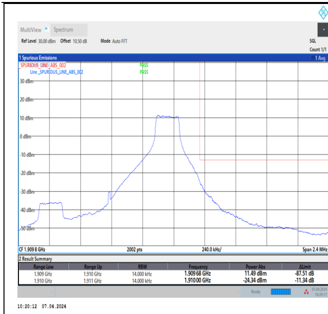
Band2_1.4MHz_64QAM_19193_1RB#5
