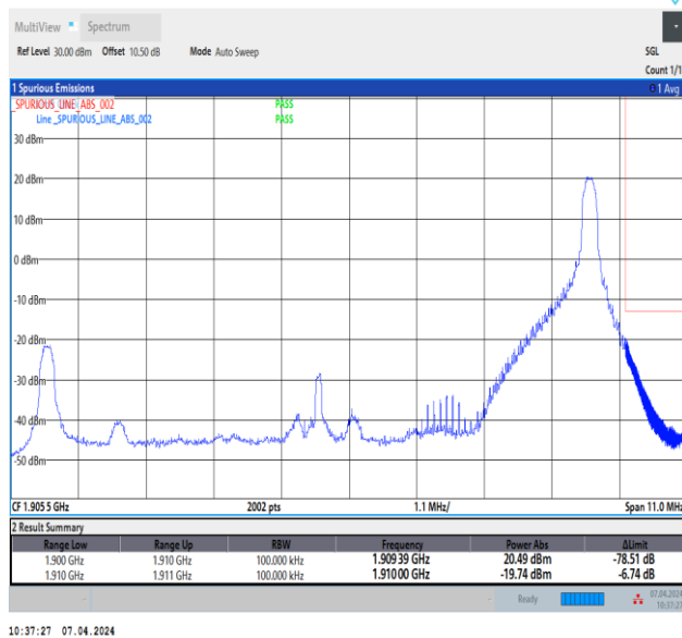
Band2_10MHz_16QAM_19150_1RB#49
