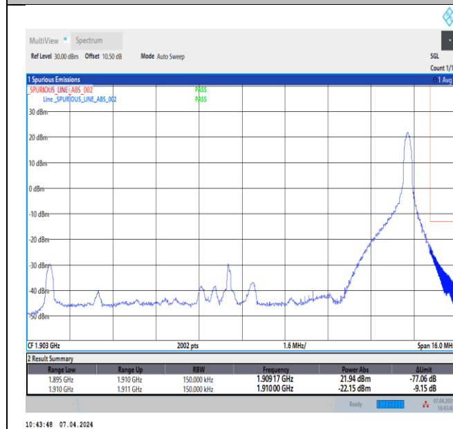
Band2_15MHz_16QAM_19125_1RB#74
