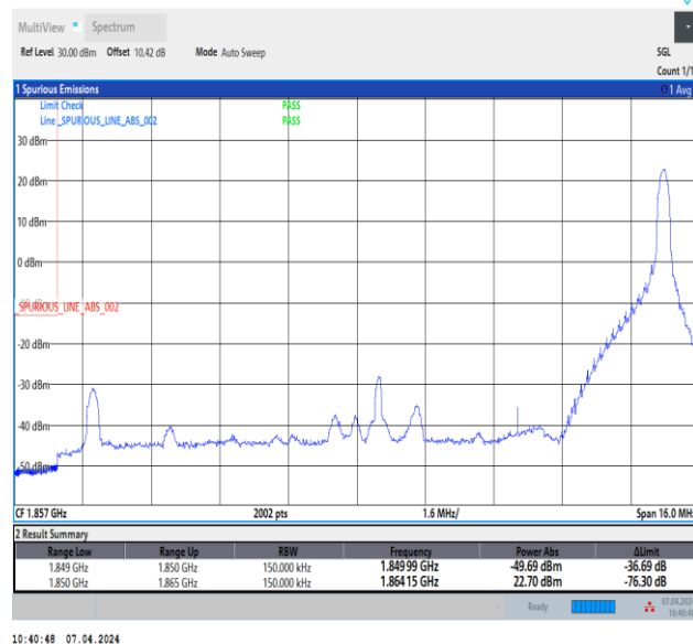
Band2_15MHz_QPSK_18675_1RB#74
