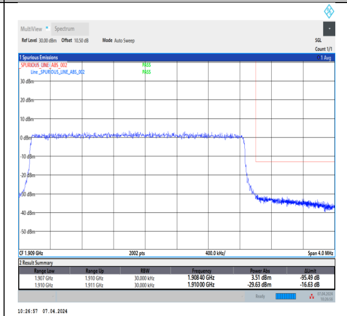
Band2_3MHz_64QAM_19185_15RB#0
