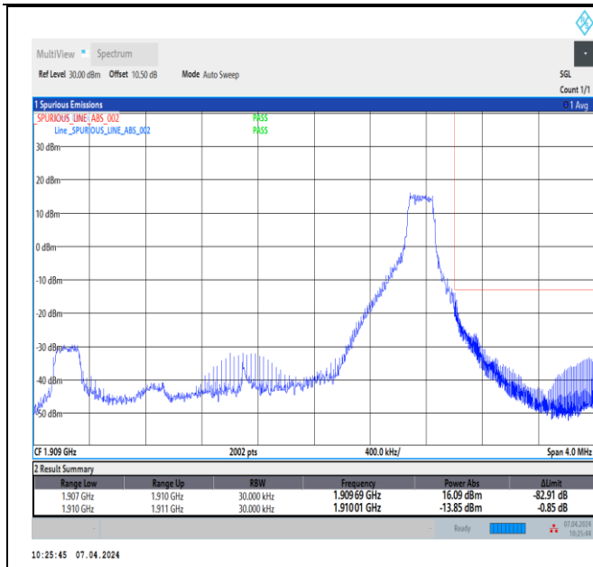
Band2_3MHz_16QAM_19185_1RB#14
