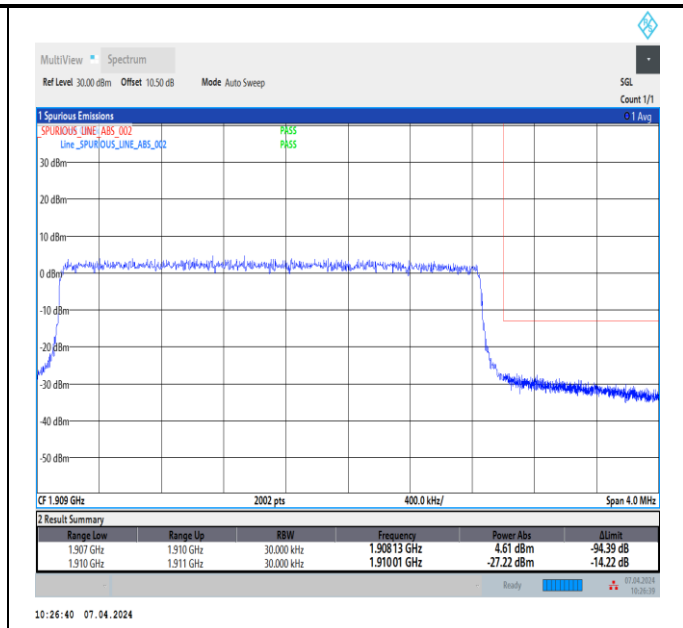
Band2_3MHz_16QAM_19185_15RB#0
