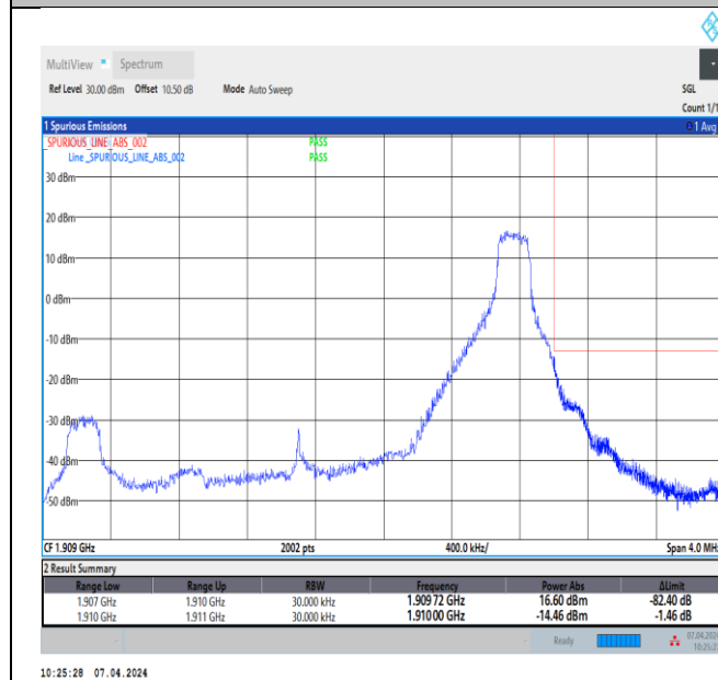
Band2_3MHz_QPSK_19185_1RB#14
