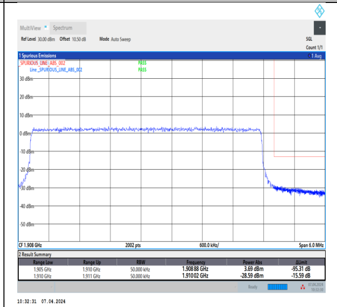
Band2_5MHz_16QAM_19175_25RB#0
