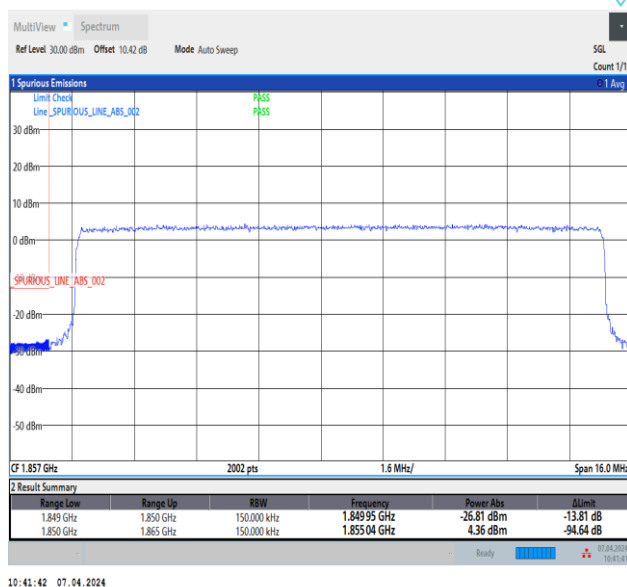
Band2_15MHz_QPSK_18675_75RB#0
