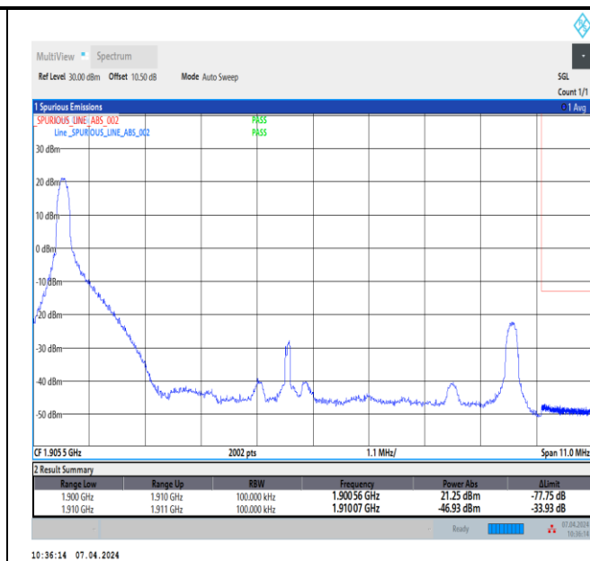
Band2_10MHz_QPSK_19150_1RB#0
