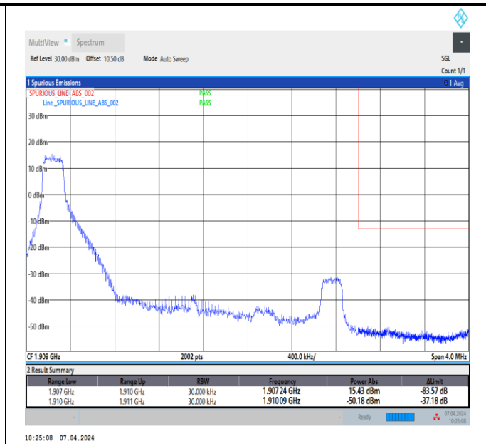
Band2_3MHz_64QAM_19185_1RB#0
