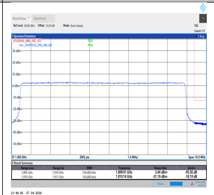
Band2_15MHz_16QAM_19125_75RB#0
