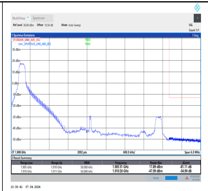
Band2_5MHz_16QAM_19175_1RB#0
