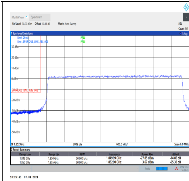
Band2_5MHz_16QAM_18625_25RB#0
