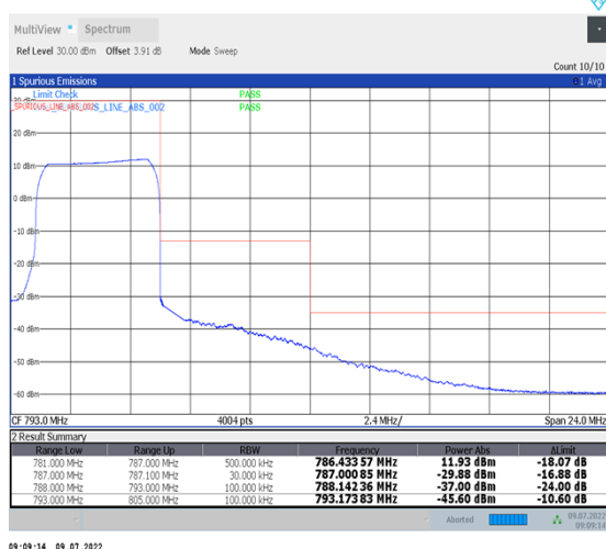
1-N13-PC3-15-5-H-6-CP-QPSK-Outer_Full-25@0-Ant1-PASS-see graph
