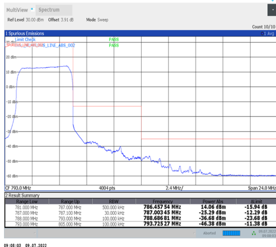
1-N13-PC3-15-5-H-3-DFT-PI2BPSK-Outer_Full-25@0-Ant1-PASS-see graph
