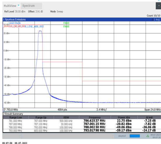
1-N13-PC3-15-5-H-2-DFT-PI2BPSK-Edge_1RB_Right-1@24-Ant1-PASS-see graph
