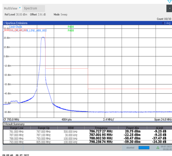
1-N13-PC3-15-5-H-5-CP-QPSK-Edge_1RB_Right-1@24-Ant1-PASS-see graph
