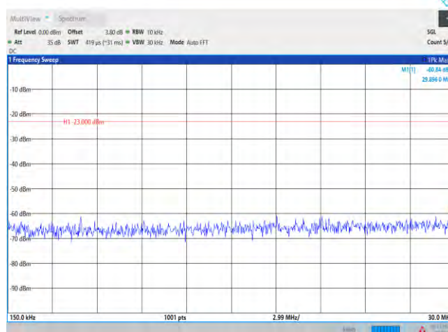
Band5-10MHz-QPSK-20450-1RB#0-Range2:0.15~30MHz
