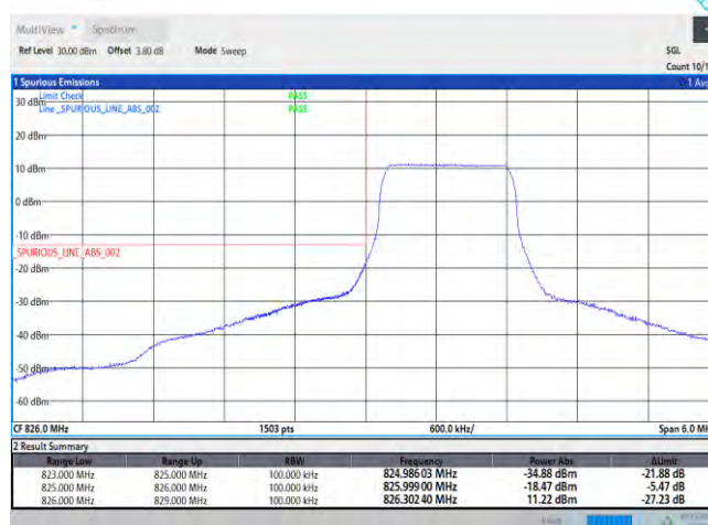
Band5-1.4MHz-QPSK-20427-6RB#0
