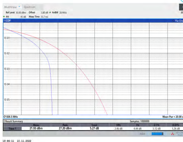
Band5-10MHz-QPSK-20525-50RB#0
