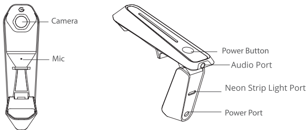
Gaming Camera
