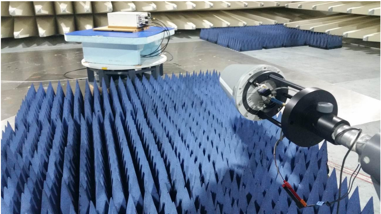
Test setup: Field Strength Emission >1 GHz @3m in the SAC
