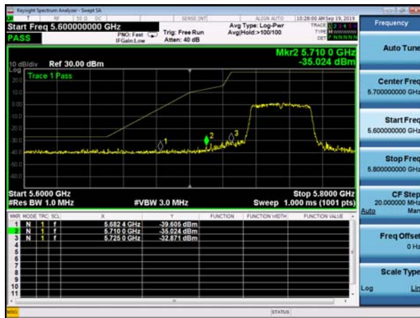
U-NII-3 Band Edge-802.11ac(80MHz) ,5775MHz, Ant2
