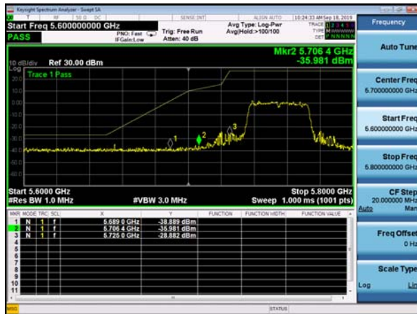
U-NII-3 Band Edge-802.11a(20MHz) ,5745MHz, Ant1
