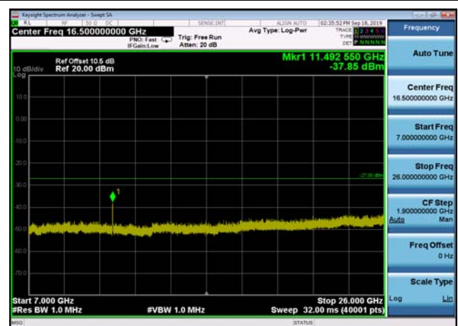
U-NII-3 ,Plot 4,7000MHz~26000MHz-802. 11ac(20MHz),5745MHz,Ant2
