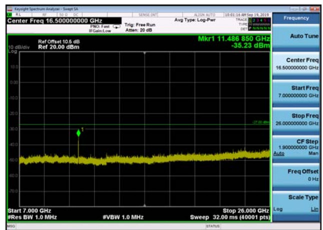
U-NII-3 ,Plot 4,7000MHz~26000MHz-802. 11a(20MHz),5745MHz,Ant2
