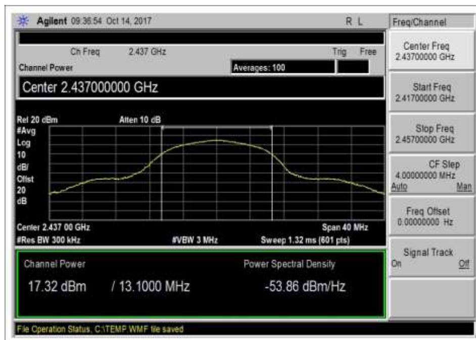
802.11b_Power_Middle_CH6_2437MHz
