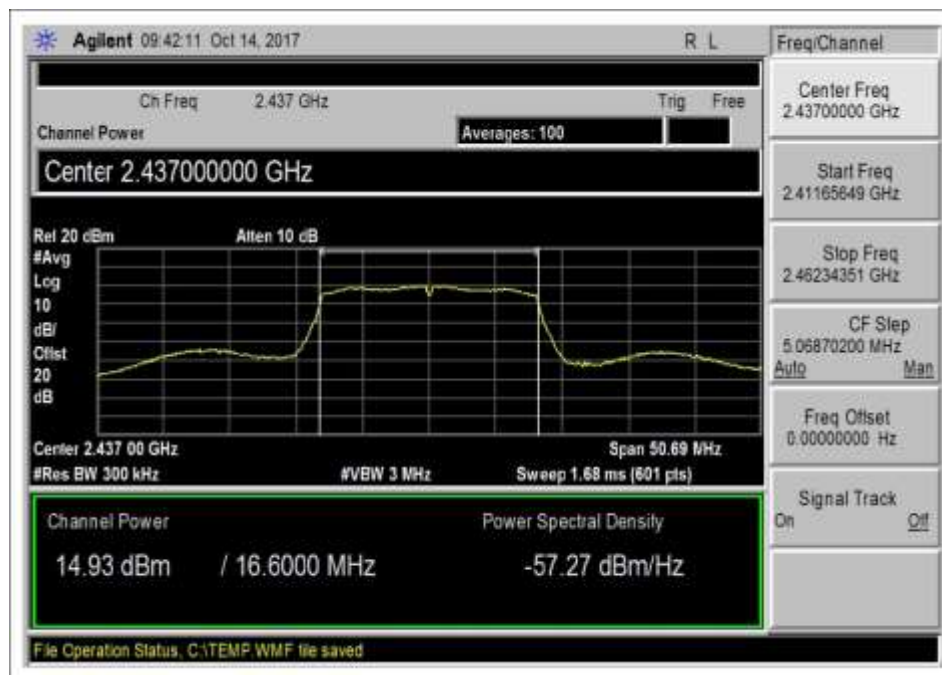
802.11g_Power_Middle_CH6_2437MHz
