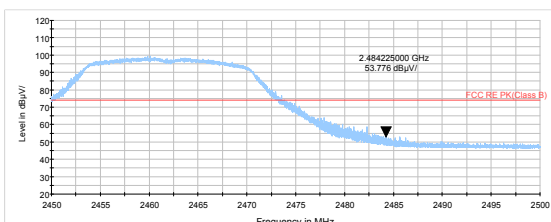
802.11n HT20 -Channel 11 Peak
