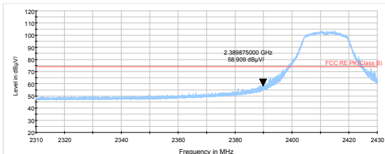
802.11g-Channel 1 Peak
