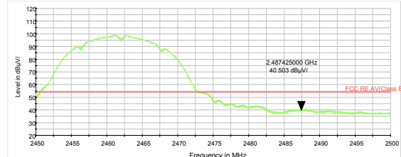
802.11b-Channel 11 Average
