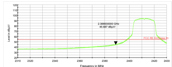
802.11g-Channel 1 Average
