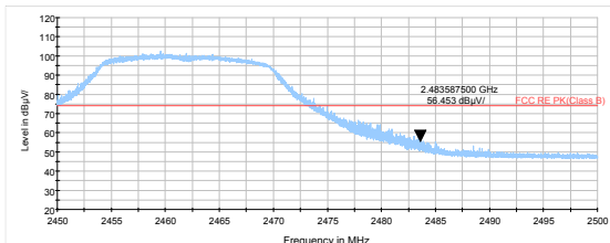
802.11g-Channel 11 Peak
