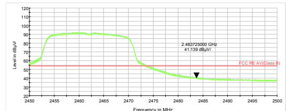
802.11g-Channel 11 Average
