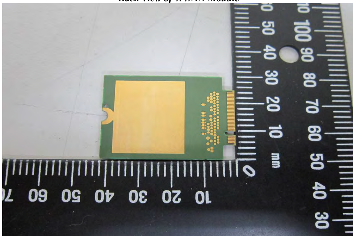
Back View of WWAN Module
