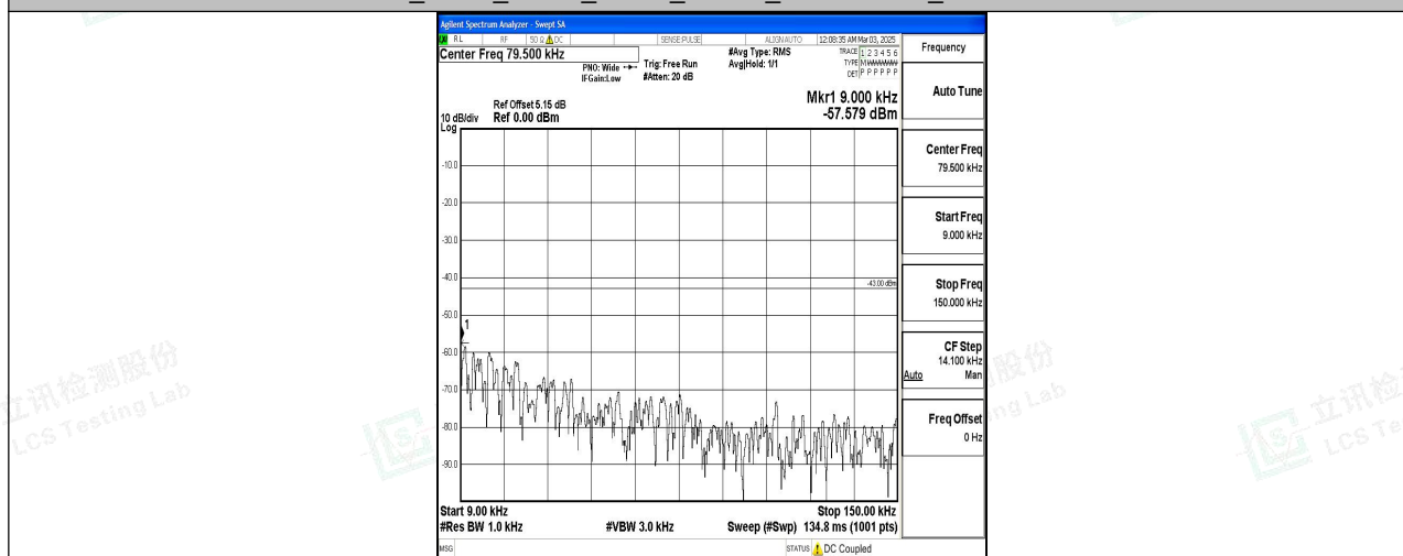
Band4_5MHz_16QAM_19975_1RB#0_0.009~0.15_0.009~0.15
