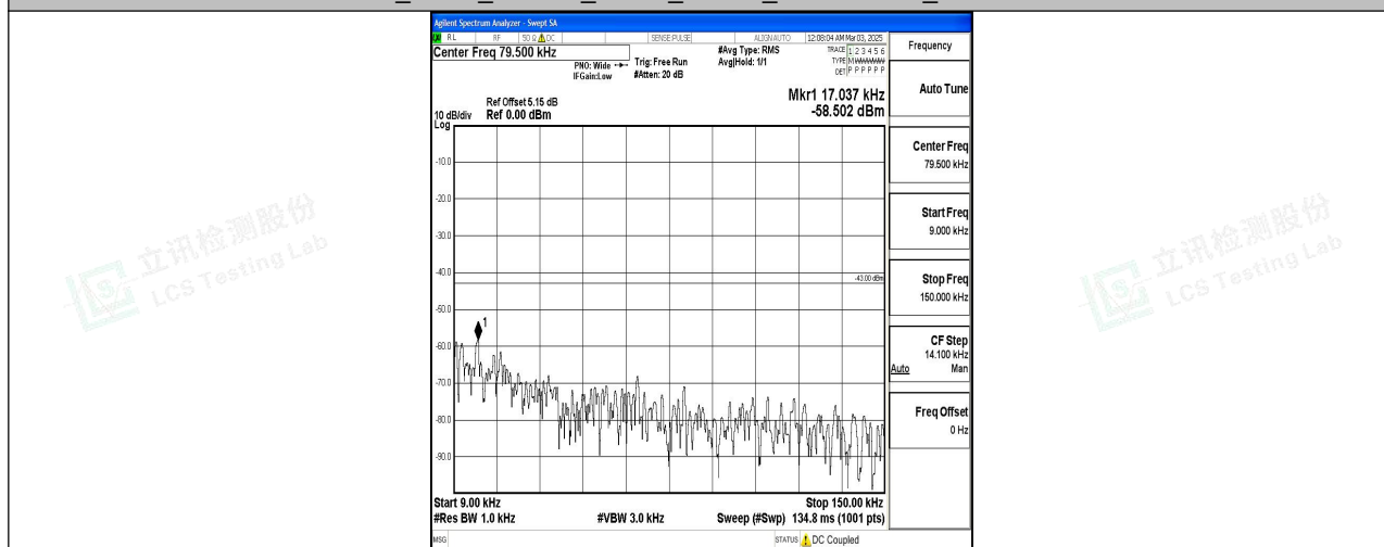
Band4_5MHz_QPSK_19975_1RB#0_0.009~0.15_0.009~0.15
