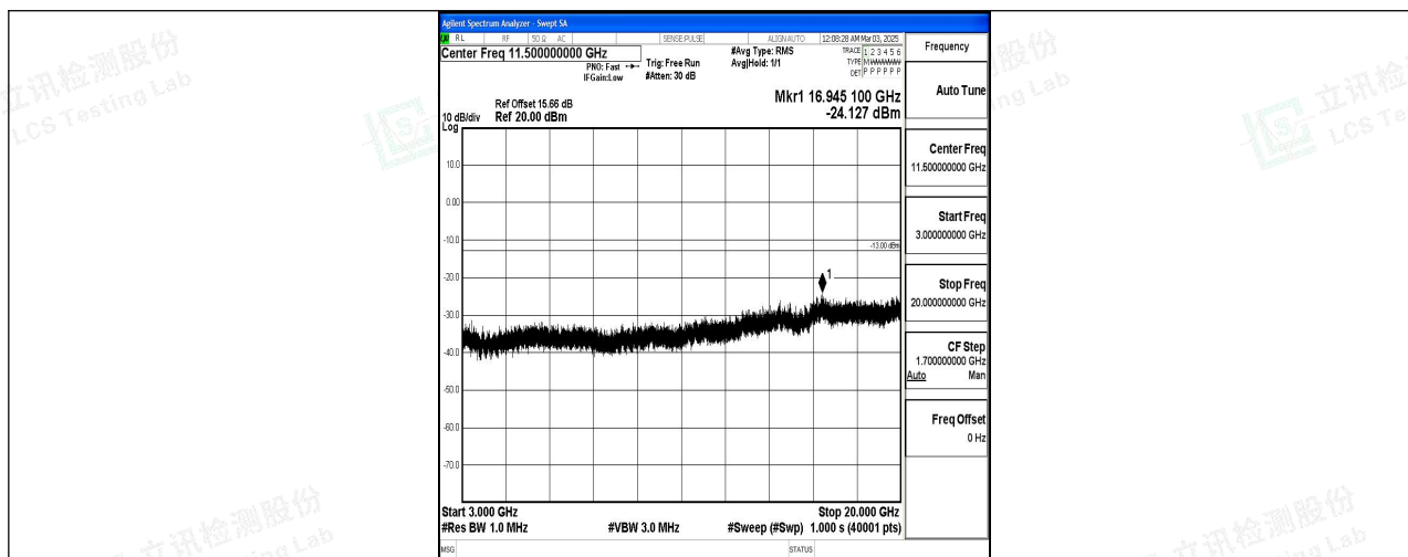
Band4_5MHz_QPSK_19975_1RB#0_3000~20000_3000~20000
