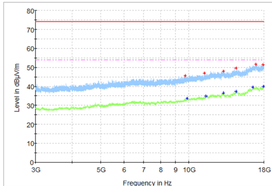
Fig.20 Radiated Spurious Emission (Ch0, 3GHz - 18GHz), 1M
