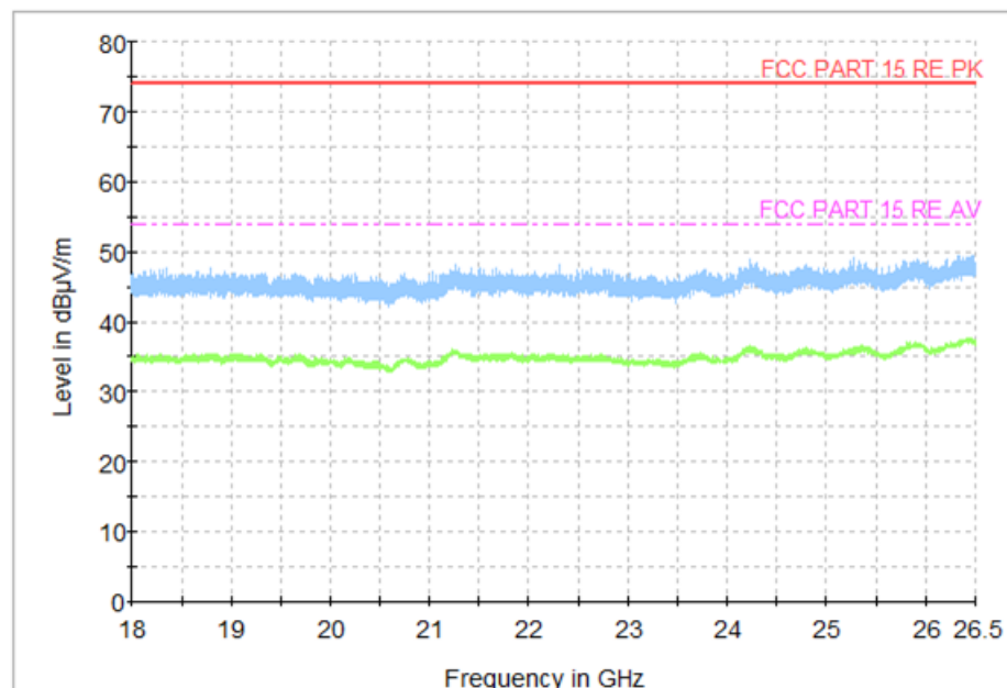
Fig.25 Radiated Spurious Emission (Ch19, 18GHz - 26.5GHz), 1M
