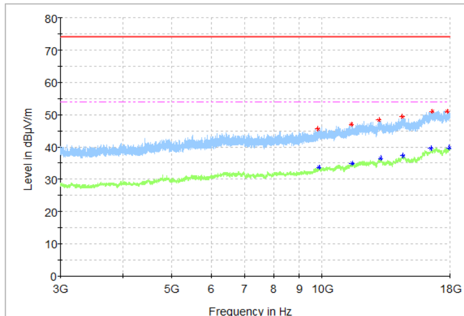
Fig.24 Radiated Spurious Emission (Ch19, 3GHz - 18GHz), 1M
