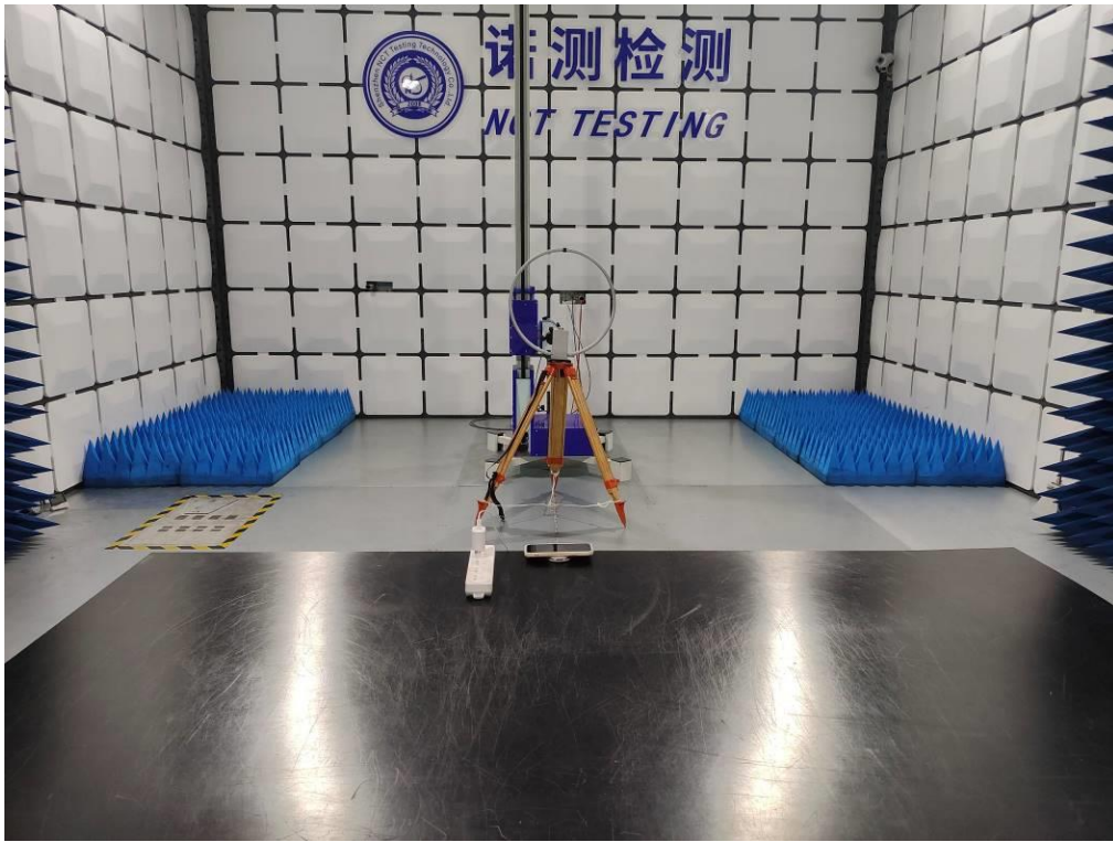
Setup Photo FCC ID: 2BFEUY103
