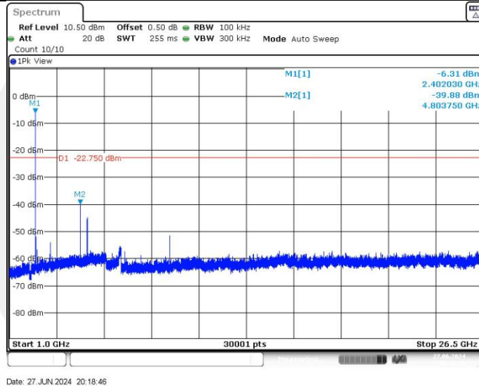
3DH5_Ant1_2402_1000~26500
