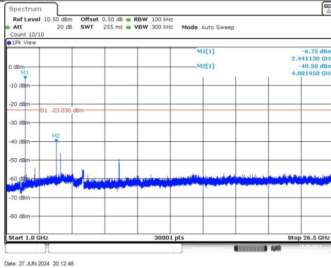
2DH5_Ant1_2441_1000~26500
