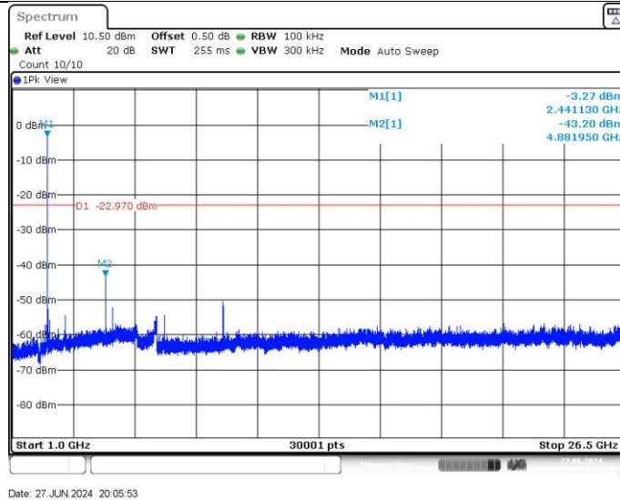
DH5_Ant1_2441_1000~26500
