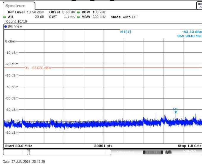
2DH5_Ant1_2441_30~1000
