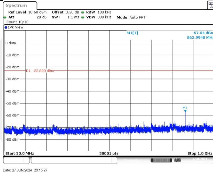
2DH5_Ant1_2480_30~1000
