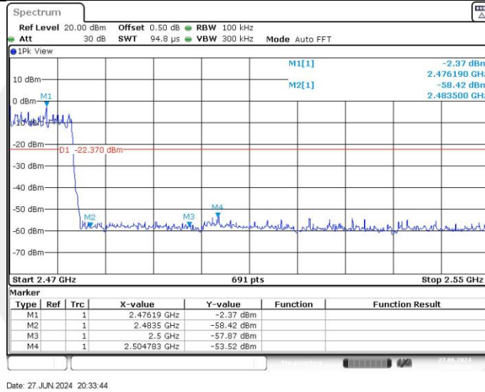
2DH5_Ant1_High_Hop_2480
