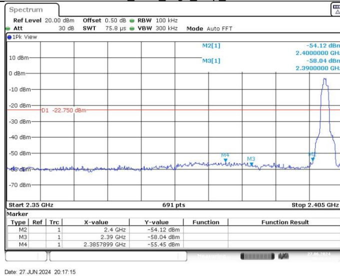
3DH5_Ant1_Low_2402
