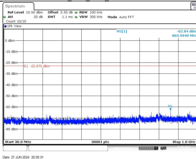
DH5_Ant1_2441_30~1000
