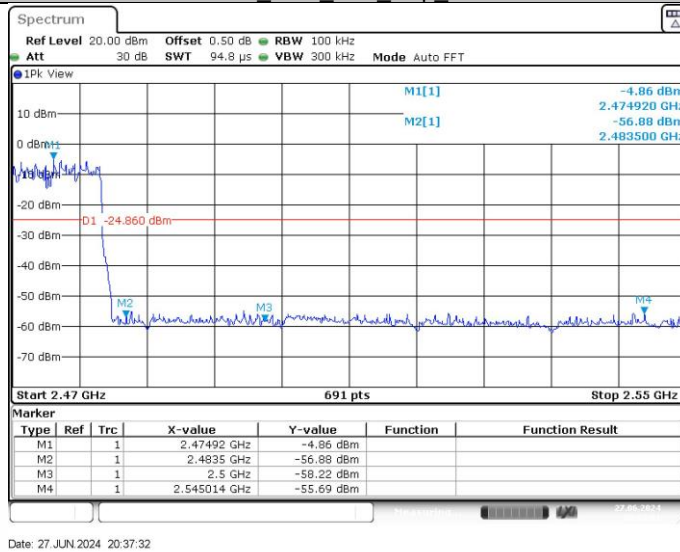
3DH5_Ant1_High_Hop_2480
