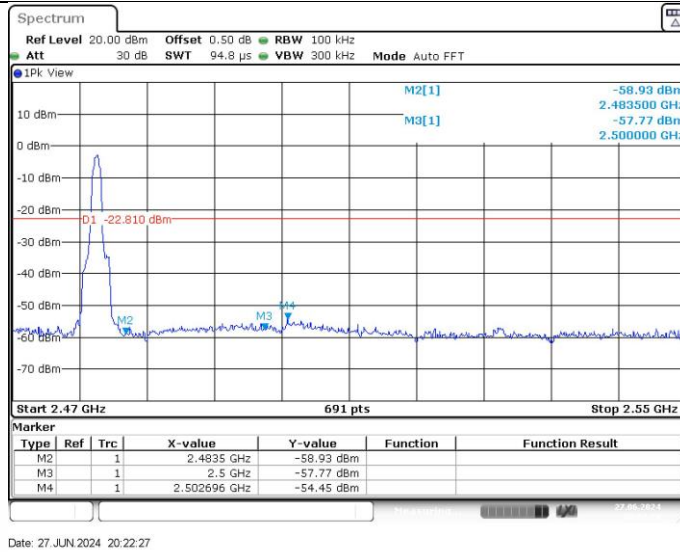
3DH5_Ant1_High_2480
