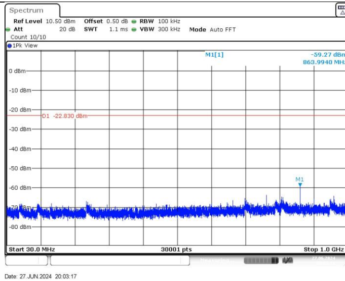
DH5_Ant1_2402_30~1000
