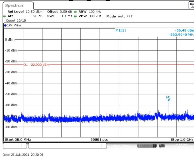
3DH5_Ant1_2441_30~1000
