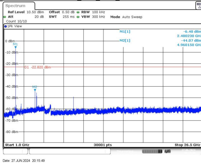
2DH5_Ant1_2480_1000~26500
