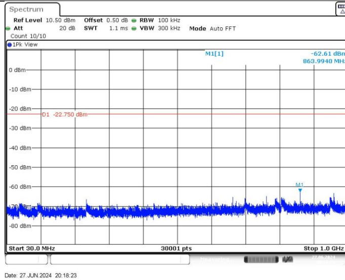
3DH5_Ant1_2402_30~1000
