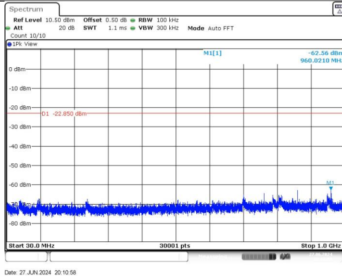
2DH5_Ant1_2402_30~1000
