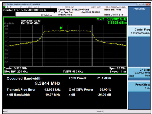
11A(10MHZ)-Ant2-5825
