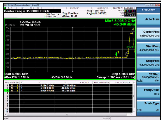
11N20MIMO-Ant2-5180-PASS
