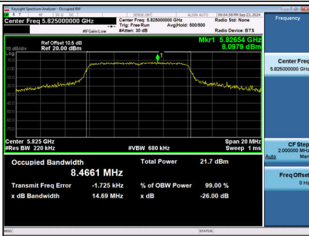
11A(10MHZ)-Ant1-5825
