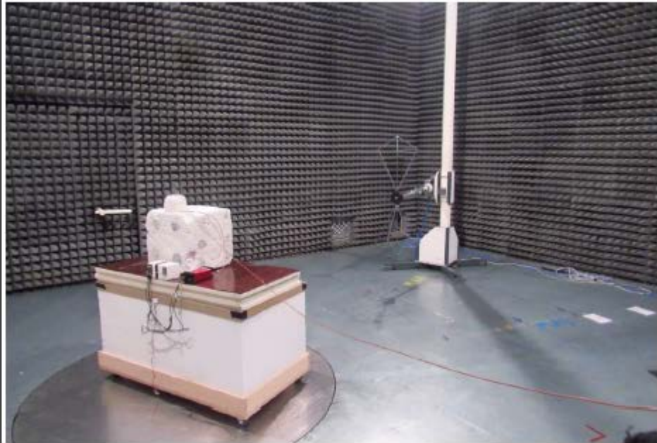
Setup 30-200MHz
